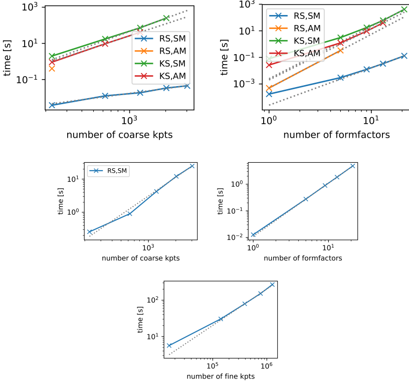
Figure 4.3.: Scaling of different implementations of the projection operation (described in the text) between channels (top row) and the calculation of the dual propagators in form-factor space (bottom row) with respect to momentum resolution and form-factor resolution. The gray dashed lines represent fits to the scaling curves.
