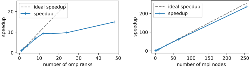
Figure 4.4.: The OMP (left) and MPI (right) scaling behaviour for the calculation of the right hand side for one RG step obtained on JURECA.
