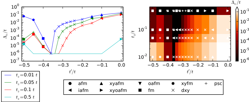
Figure 5.19.: Phase diagram of the anisotropic 3D-Hubbard model with t'_z = 0t in two different representations. Due to the limited numerical resolution no divergences for \Lambda_c < 10^{-6}t could be observed, so that all the corresponding cases are displayed by a critical scale \Lambda_c = 9 \cdot 10^{-7}t without a favourable ordering in the left plot. In the right plot, u as unidentified refers to an appearance of features of different ordering tendencies at the same time, such that even an educated guess is impossible.
