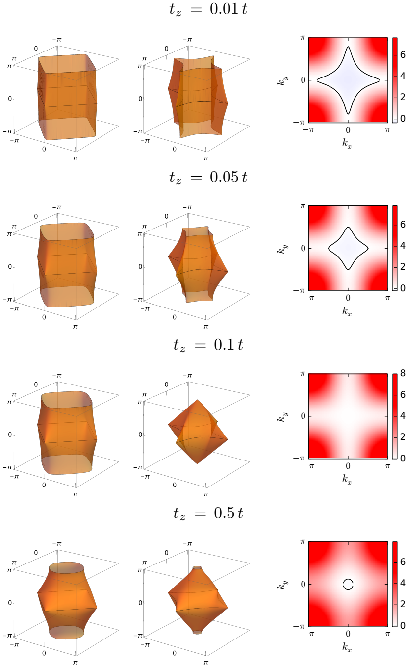
Figure 5.16.: Fermi-surfaces (left and middle column) and energy maps in the (z = \pi) -plane (right column) of the non-isotropic Hubbard model. The anisotropy increases from top to bottom corresponding to t_z/t = 0.01, 0.05, 0.1, 0.5 . For t_z = 0.5 , i.e. in the lowest row, the next-nearest neighbour hopping is t_z = 0t (left) and t' = -0.24t (centre and right) while in the other three cases it is set to t' = 0t (left) and t' = -0.45t (centre and right). When t' = -0.24t is further increased for t_z = 0.5t , the Fermi-surface does not reach the (z = \pi) -plane any more. Similarly, for t_z = 0.1t and t' = -0.45t the Fermi-surface only reaches the point (0, 0, \pi) .
