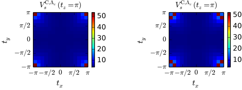
Figure 5.11.: The s -wave form-factor contribution of the full vertex at the final scale \Lambda_c projected to the C-channel is displayed in the z = \pi -plane for \mu = 0.0t (left) and \mu = -0.4t (right). The AFM nesting vector (\pi, \pi, \pi) splits up and becomes incommensurate upon doping, and, thus, moves along the (x, \pi, \pi) and along the (\pi, y, \pi) lines.
