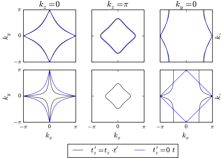
Figure 5.24.: Comparison of the Fermi-surface in the (k_z = 0) -, (k_z = \pi) - and (k_y = 0) -plane (from left to right) resulting from t'_z = 0t and t'_z = t_z \cdot t' for t' = -0.32t and t' = -0.45t in the top and bottom row, respectively, at t_z = -0.1t .
