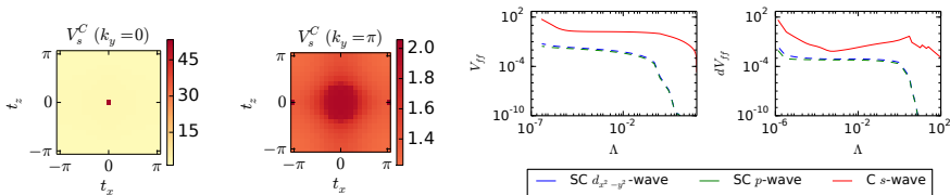
Figure C.16.: From left to right: Cut through the interaction in the C-channel on-site form-factor in the y = 0 -plane, in the y = \pi -plane, flow of the largest values of the three main channels and their derivatives for t' = -0.45t .
