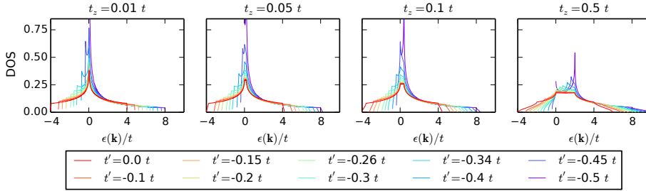
Figure 5.17.: Density of states (DOS) for t_z/t = 0.01, 0.05, 0.1, 0.5 from left to right and for various values of t' .
