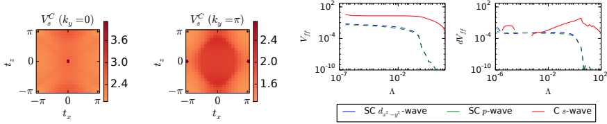
Figure C.12.: From left to right: Cut through the interaction in the C-channel on-site form-factor in the y = 0 -plane, in the y = \pi -plane, flow of the largest values of the three main channels and their derivatives for t' = -0.32t .
