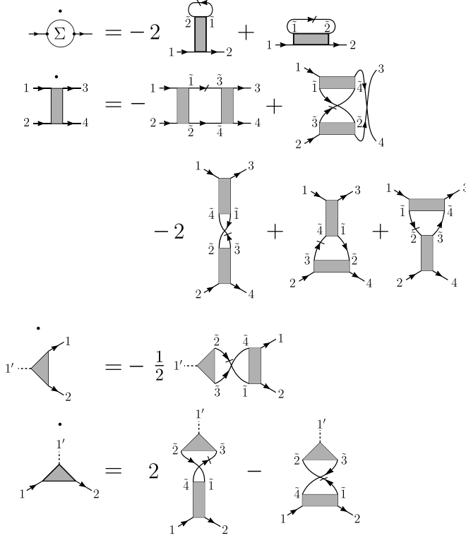
Figure 3.13.: Diagrammatic representation of the SU(2)-symmetric flow equations as provided by theorem 3.25.
