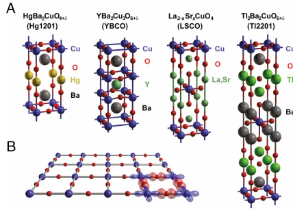
Figure 5.2.: A: Unit cells of the lattice of different copper-oxide superconductors. The characteristic CuO square layers in which the superconductivity takes place can be identified at the top and at the bottom of the unit cells except for YBCO, where it is above and below the Yttrium atom.
