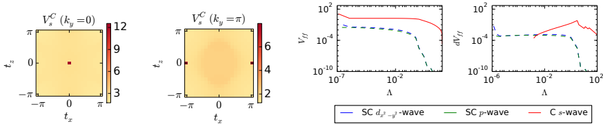
Figure C.14.: From left to right: Cut through the interaction in the C-channel on-site form-factor in the y = 0 -plane, in the y = \pi -plane, flow of the largest values of the three main channels and their derivatives for t' = -0.36t .
