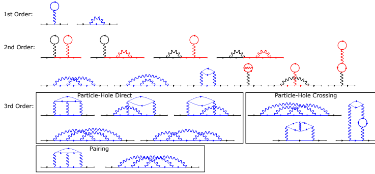
Figure 3.4.: Feynman Diagrams of the zeroth, first, second and (incomplete) third order interaction expansion corresponding to the Gell-Mann and Low theorem and to the Wick theorem for the one-particle Green's function. Here, the bare interaction V_0 is represented by an undirected wave line. The contributions to the self-energy of this expansion (see def. 30) are in blue. Those parts of the diagram which can be replaced by a full Green's function (see text) are red. The third-order diagrams are grouped corresponding to the channels they belong to. Remark that this diagrammatic representation does not account for correct prefactors and signs.
