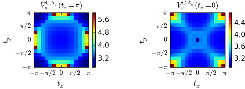
Figure 5.15.: The s -wave form-factor contribution of the full vertex at final scale \Lambda_c projected to the C-channel for \mu = -1.8t in the z = \pi -plane (left) and in the z = 0 -plane (right).
