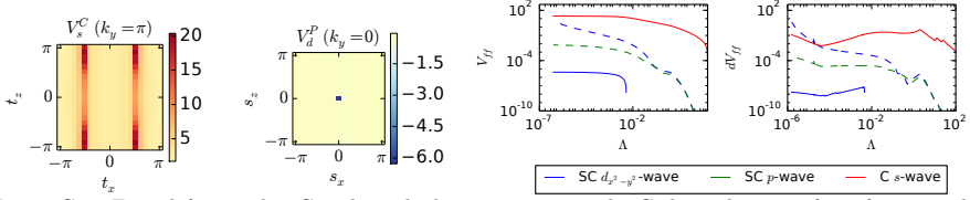
Figure C.1.: From left to right: Cut through the interaction in the C-channel on-site form-factor in the y = \pi -plane, in the P-channel d-wave form-factor in the y = 0 -plane, flow of the largest values of the three main channels and their derivatives for t' = -0.34 t .
