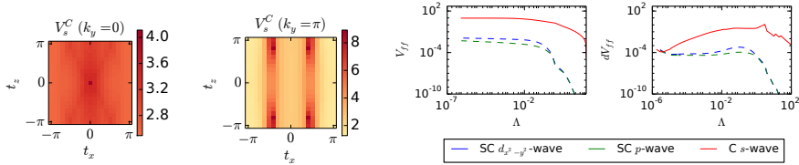
Figure C.4.: From left to right: Cut through the interaction in the C-channel on-site form-factor in the y = 0 -plane, in the y = \pi -plane, flow of the largest values of the three main channels and their derivatives for t' = -0.34 t .
