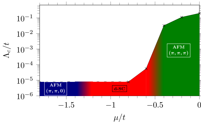
Figure 5.10.: Phase diagram of the three-dimensional Hubbard model upon doping. For \mu < 0.8t the flow did not converge within the precision range provided by our resolution, indicated by a horizontal dashed line. An investigation of the resulting vertex at the final scale and of the increase of the channels during the last steps of the flow lead to the indicated ordering tendencies in this range of parameters.
