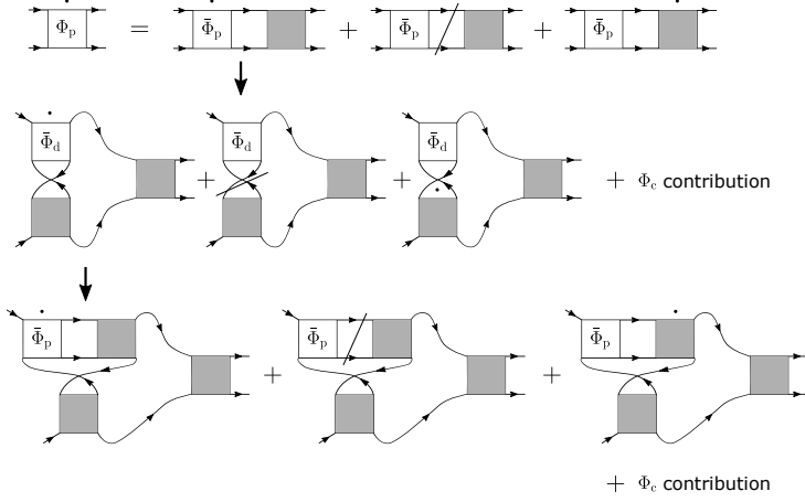
Figure 3.12.: Schematic representation of the procedure to obtain the derivative of the Parquet equation for the pairing channel. As the derivative also acts on the interactions, they have to be replaced by the derivative of its constituents, here we illustrate the insertion of the direct particle-hole contribution. In the inserted channel the derivative of the two-particle interactions has to be replaced again, here illustrated by an insertion of the pairing channel. This procedure continues until only the derivative of the dual propagator remains, thus resulting in an infinite hierarchy of equations.
