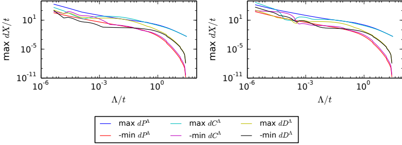
Figure 5.14.: Largest attractive and repulsive increments of the different channels (i.e. \max_{i,s}(d/d\Lambda P_{i,i}^\Lambda(\mathbf{s})) , \max_{i,t}(d/d\Lambda C_{i,i}^\Lambda(\mathbf{t})) , \max_{i,u}(d/d\Lambda D_{i,i}^\Lambda(\mathbf{u})) and similarly for |\min| ) for \mu = -1.2t (left) and \mu = -1.4t (right), indicating a tendency to SC and AFM order, respectively.
