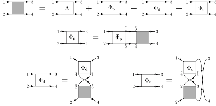
Figure 3.7.: Diagrammatic representation of the vertex decomposition according to the parquet scheme and to the corresponding Bethe-Salpeter equations.
