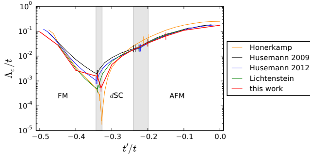
Figure 5.5.: Phase diagram of the 2D-Hubbard model calculated in this work in comparison to results obtained by others, i.e. Honerkamp [150], Husemann ('09) [67], Husemann ('12) [114] and Lichtenstein [2]. The critical temperature obtained by Honerkamp is directly compared to the critical cut-off scales of the other references, revealing the divergence appearing at similar scales, such that a comparison of both properties is reasonable. Further, the critical scales obtained in our calculation are in good agreement with those obtained in the presented works.
