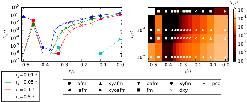
Figure 5.23.: Phase diagram of the anisotropic 3D-Hubbard model with t'_z \neq 0t in two different representations. Due to the limited numerical resolution no divergences for \Lambda_c < 10^{-6} t could be observed, so that all corresponding cases are displayed as \Lambda_c = 9 \cdot 10^{-7} t without a favourable ordering in the left plot. In the right plot, u refers to an appearance of features of different ordering tendencies at the same time, such that even an educated guess is impossible.
