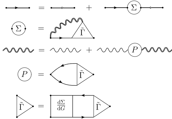
Figure 3.8.: Diagrammatic representation of the full set of Hedin equations. Due to the locality in space and time, the bare (effective) interaction is collapsed to a (double) wave line.
