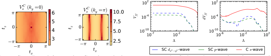
Figure C.2.: From left to right: Cut through the interaction in the C-channel on-site form-factor in the y = 0 -plane, in the y = \pi -plane, flow of the largest values of the three main channels and their derivatives for t' = -0.36 t .
