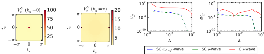
Figure C.15.: From left to right: Cut through the interaction in the C-channel on-site form-factor in the y = 0 -plane, in the y = \pi -plane, flow of the largest values of the three main channels and their derivatives for t' = -0.4t .
