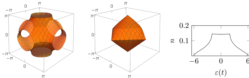
Figure 5.7.: Fermi-surface of the three-dimensional Hubbard model at half-filling (left) and at \mu = -2t (centre) and the density of states at half-filling (right).
