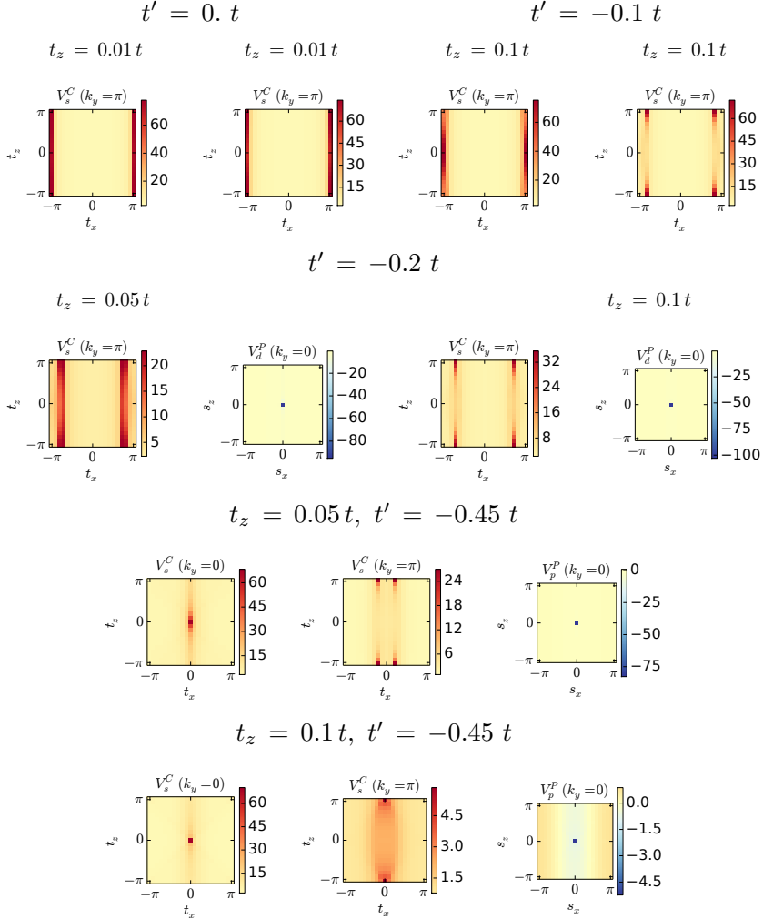
Figure 5.20.: Cuts through the full vertex projected to one channel at the end of the flow.
