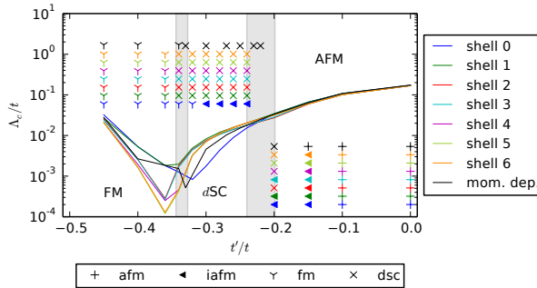
Figure 5.6.: Convergence of the TUFGR approach for the 2D-Hubbard model with an increasing number of shells towards the full momentum space result. According to section 4.2 0, 1, 2, 3, 4, 5, 6 shells correspond to 1, 5, 9, 13, 21, 25, 29 form-factors, respectively.
