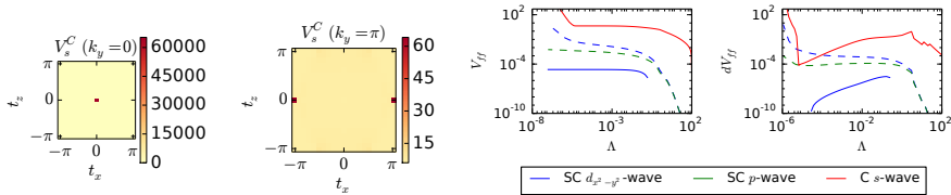
Figure C.6.: From left to right: Cut through the interaction in the C-channel on-site form-factor in the y = 0 -plane, in the y = \pi -plane, flow of the largest values of the three main channels and their derivatives for t' = -0.1 t .
