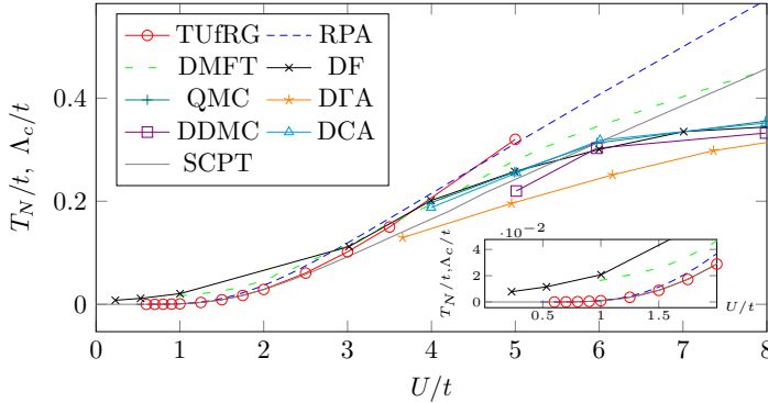
Figure 5.9.: Phase diagram of the half-filled three-dimensional Hubbard model. The critical scale \Lambda_c obtained in this thesis (TUFGR) indicates a transition to an AFM ground state with (\pi, \pi, \pi) ordering. This result is compared to the Néel temperature indicating a corresponding phase transition obtained by other methods, i.e. spin-fluctuation corrected Random Phase Approximation (RPA) [34, 152, 153], Dynamical Mean Field Theory (DMFT) [154], Dual Fermion (DF) [154], Quantum Monte Carlo (QMC) [155], Dynamical Vertex Approximation (DGA) [156], Determinantal Diagrammatic Monte Carlo (DDMC) [157] and Dynamical Cluster Approximation (DCA) [158].
