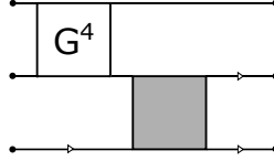
Figure 3.10.: Graphical representation of a term contributing to the three-particle Green's function. As the two-particle interactions are connected via a torso line, the contribution is one-particle irreducible.
