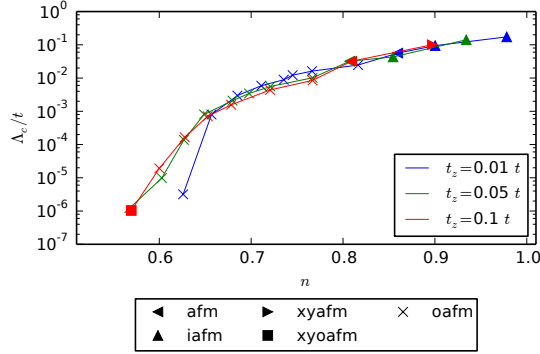
Figure 5.25.: Phase diagram \Lambda_c versus electron density n for the anisotropic 3D-Hubbard model for t'_z = t_z \cdot t' . The symbols are the same as in figures 5.19 and 5.23.
