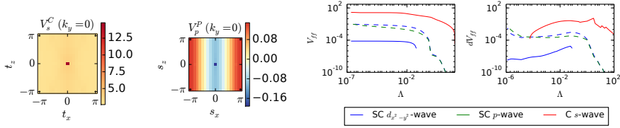
Figure C.5.: From left to right: Cut through the interaction in the C-channel on-site form-factor in the y = 0 -plane, in the P-channel p-wave form-factor in the y = 0 -plane, flow of the largest values of the three main channels and their derivatives for t' = -0.36 t .
