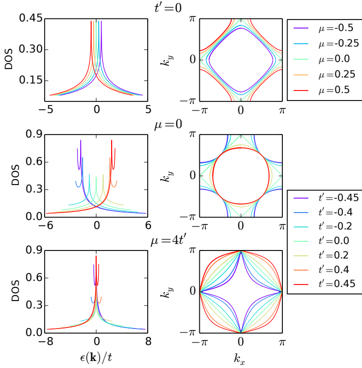
Figure 5.3.: Density of states (DOS) (left) and Fermi-surface (right) of the 2D-Hubbard model. At the top for various values of \mu at t' = 0t . At the centre and bottom for various values of t' at \mu = 0 and \mu = \epsilon_{vH} , respectively.
