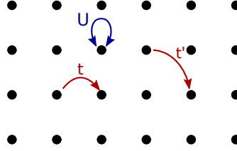
Figure 5.1.: Schematic representation of the effects included in the Hubbard model with onsite-repulsion U (blue), nearest neighbour hopping t and second nearest neighbour hopping t' (red) on an isotropic two-dimensional lattice.
