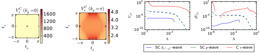
Figure C.8.: From left to right: Cut through the interaction in the C-channel on-site form-factor in the y = 0 -plane, in the y = \pi -plane, flow of the largest values of the three main channels and their derivatives for t' = -0.2t .
