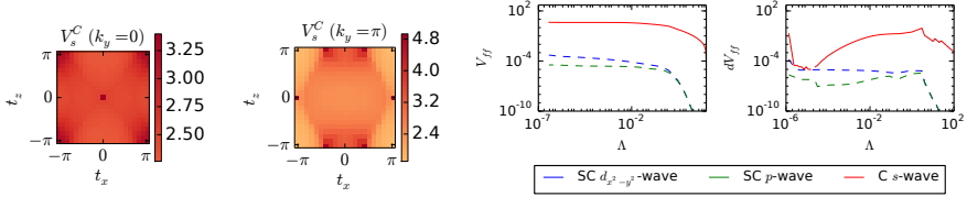
Figure C.7.: From left to right: Cut through the interaction in the C-channel on-site form-factor in the y = 0 -plane, in the y = \pi -plane, flow of the largest values of the three main channels and their derivatives for t' = -0.15t .
