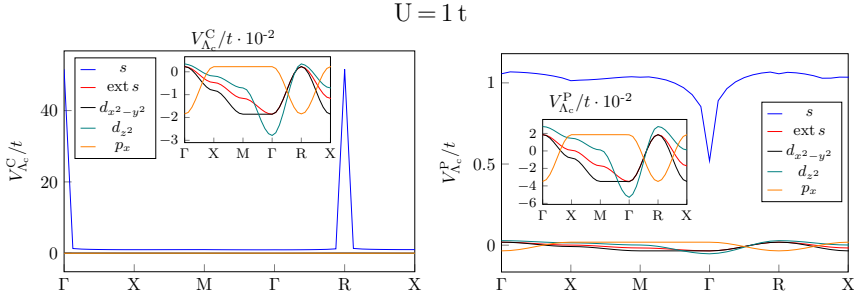
Figure 5.8.: Linescan along the high-symmetry lines connecting \Gamma = (0, 0, 0) , X = (\pi, 0, 0) , M = (\pi, \pi, 0) and R = (\pi, \pi, \pi) for the final vertex projected to the form-factor resolved C-channel (left) and the P-channel (right) at half-filling for an initial interaction of U = 1t .
