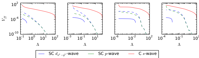
Figure 5.18.: Flow of the charge chantage in the on-site form-factor (C s -wave) and pairing chantage in the p_x (SC p -wave) and the d_{x^2-y^2} (SC d_{x^2-y^2} -wave) form-factors towards the critical scales. The sets of parameters correspond, from left to right, to a final antiferromagnetic ( t' = 0 t ), d -wave superconducting ( t' = -0.24 t ), ferromagnetic ( t' = -0.4 t ) and p -wave superconducting ( t' = -0.45 t ) phase as t_z = 0.05 t .
