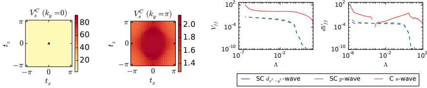
Figure C.13.: From left to right: Cut through the interaction in the C-channel on-site form-factor in the y = 0 -plane, in the y = \pi -plane, flow of the largest values of the three main channels and their derivatives for t' = -0.34t .
