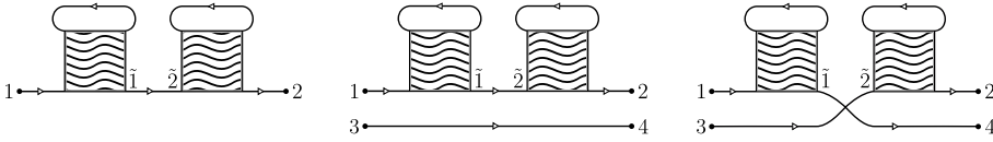
Figure 3.2.: Graphical representation of the operation of cutting a propagator line of the left diagram: An unconnected line is inserted (middle) and a permutation of the slots of the line which is supposed to be cut with the new external arguments is performed (right).
