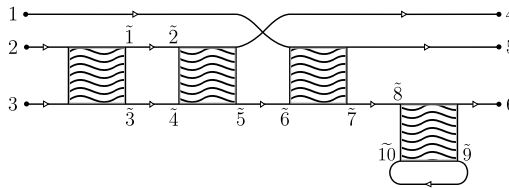
Figure 3.3.: Diagrammatic representation of the terms defined in Def. 28. The lines connecting the graph with the labels 1, \dots, 6 are external lines, while all the others are internal ones. The lines connecting the two interactions in the left ( \tilde{1}-\tilde{2}, \tilde{3}-\tilde{4} ) and the line connecting the rightmost interaction with itself ( \tilde{9}-\tilde{10} ) are non-essential, as the graph remains connected upon cutting those lines, while the other two internal lines ( \tilde{5}-\tilde{6}, \tilde{7}-\tilde{8} ) are essential, so that the graph is one-particle irreducible. The graph is also amputable, as the line \tilde{7}-\tilde{8} is an extremity propagator, as after cutting, the part of the rightmost interaction has exactly two external lines, while the line \tilde{5}-\tilde{6} is a torso-propagator. Considering only the part of the diagram containing the two interactions to the left, one obtains a two-particle reducible diagram, as it separates after the simultaneous splittings of the two propagators \tilde{1}-\tilde{2} and \tilde{3}-\tilde{4} .
