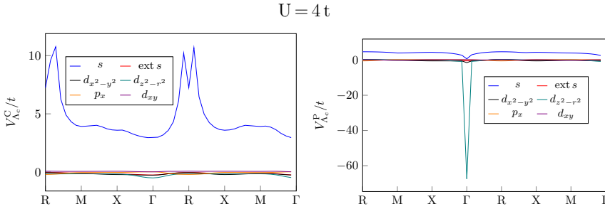
Figure 5.12.: Linescan along the high-symmetry lines connecting \Gamma = (0,0,0) , X = (\pi,0,0) , M = (\pi,\pi,0) and R = (\pi,\pi,\pi) for the final vertex projected to the form-factor resolved C-channel (left) and to the P-channel (right) with \mu = -0.6t .
