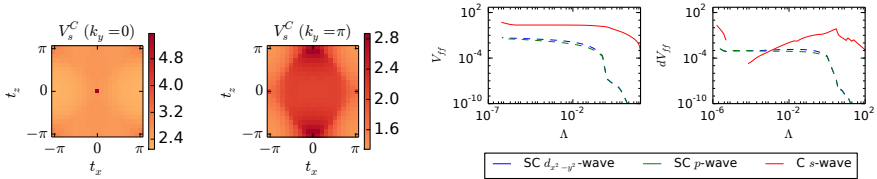
Figure C.10.: From left to right: Cut through the interaction in the C-channel on-site form-factor in the y = 0 -plane, in the y = \pi -plane, flow of the largest values of the three main channels and their derivatives for t' = -0.26t .
