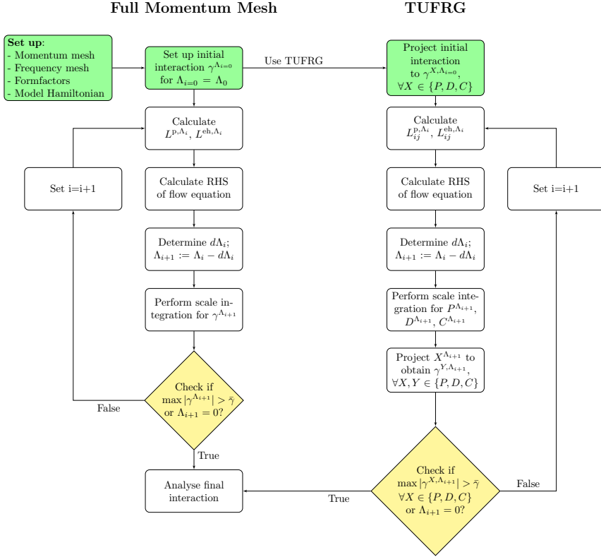
Figure 4.1.: The basic scheme of the code developed within this thesis for the FRG with the vertex in a pure momentum representation (left) and in the TUFGR parametrisation. To simplify the representation we use the abbreviation \gamma := \gamma^{(4,0)} for the two-fermion interaction and \bar{\gamma} := \gamma_{\max} for the threshold which is used to determine the divergence of the flow. The SU(2)-symmetric version of the code follows the same scheme with \gamma replaced by its SU(2)-symmetric counterpart.
