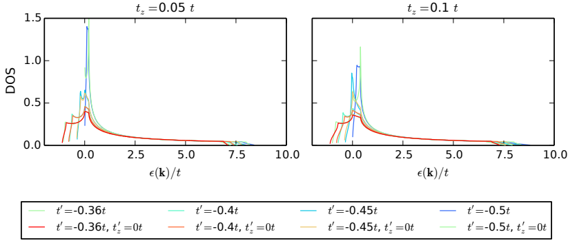
Figure 5.22.: Non-isotropic Hubbard model: Comparison of the density of states (DOS) for t_z = 0.05 t (left) and t_z = 0.1 t (right) with t'_z = 0t and t'_z = t_z \cdot t' .
