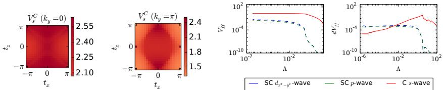
Figure C.11.: From left to right: Cut through the interaction in the C-channel on-site form-factor in the y = 0 -plane, in the y = \pi -plane, flow of the largest values of the three main channels and their derivatives for t' = -0.28t .
