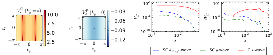
Figure C.3.: From left to right: Cut through the interaction in the C-channel on-site form-factor in the y = \pi -plane, in the P-channel d-wave form-factor in the y = 0 -plane, flow of the largest values of the three main channels and their derivatives for t' = -0.32 t .
