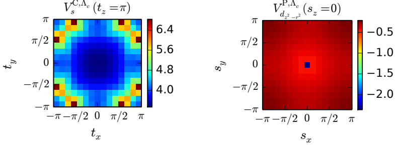
Figure 5.13.: Full vertex at the final scale \Lambda_c projected to the C-channel (left) and to the P-channel (right) for \mu = -1.0t . For the C-channel the s -wave contribution is shown in the z = \pi -plane, while the d_{3z^2-r^2} form-factor contribution in the z = 0 -plane is shown for the P-channel.
