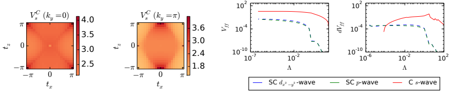
Figure C.9.: From left to right: Cut through the interaction in the C-channel on-site form-factor in the y = 0 -plane, in the y = \pi -plane, flow of the largest values of the three main channels and their derivatives for t' = -0.24t .
