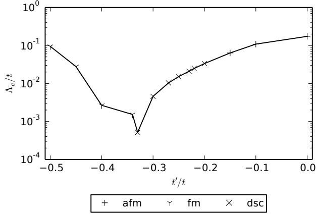
Figure 5.4.: Phase diagram of the 2D-Hubbard model based on the vertex with a full momentum parametrisation.
