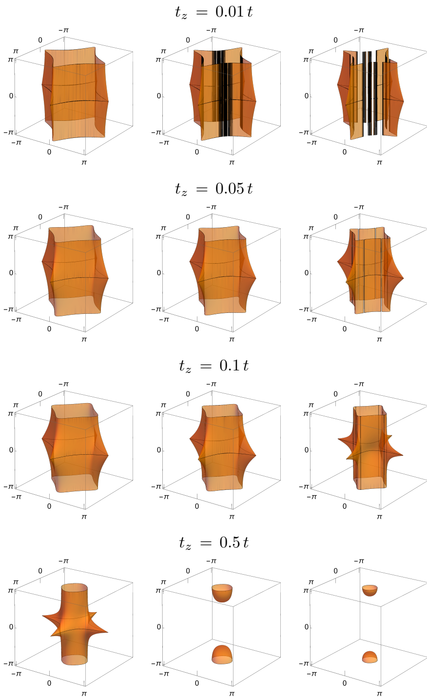
Figure 5.21.: Fermi-surface of the anisotropic Hubbard model with (from top to bottom) t_z = 0.01 t, 0.05 t, 0.1 t, 0.5 t and (from left to right) t' = 0.32 t, -0.4 t, -0.45 t while t'_z = t_z \cdot t' .
