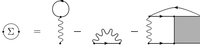
Figure 3.6.: Diagrammatic representation of the Schwinger-Dyson equation for the calculation of the self-energy.
