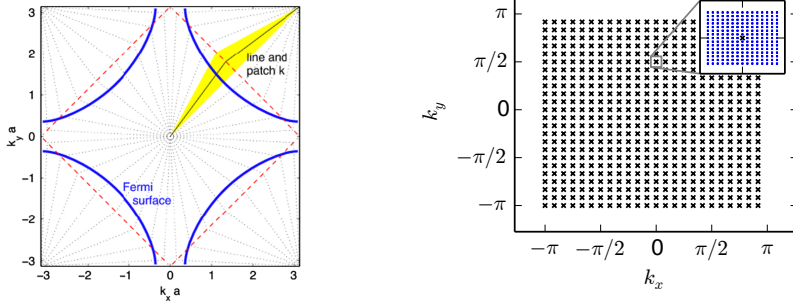
Figure 4.2.: Left: Representation of the N -patch FRG discretisation taken from Metzner [104]. The Brillouin zone is divided into N patches. All interactions depending on a momentum in the patch are represented by the corresponding momentum located at the Fermi-surface, as the dominant interactions are expected close to the Fermi-surface.
