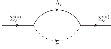
Figure 3. Loop diagrams of the self-energy for \Sigma_c^{(*)} .
