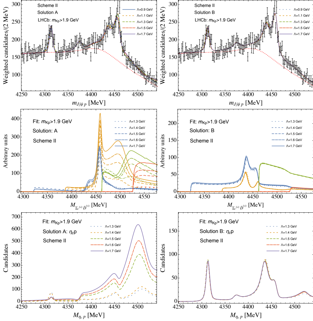
Figure 8. First row: best fit results for solutions A (left) and B (right) for different cutoffs \Lambda using a potential of scheme II. The background is shown as red-dotted curve. Second row: cutoff dependence of the predicted line shapes of \Sigma_c \bar{D} (blue), \Sigma_c^* \bar{D} (orange), \Sigma_c \bar{D}^* (green), and \Sigma_c^* \bar{D}^* (red) mass distributions. Third row: cutoff dependence of the predicted line shapes for the \eta_c p mass distributions. No background is included for predicted line shapes.
