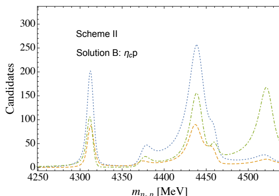
Figure 11. Predictions for the line shapes of the \eta_{cp} invariant mass distributions based on various fit results for solution B of scheme II. The blue dotted, orange dashed and green dot-dashed curves correspond to the predictions from the three fit results ( \cos\theta_{P_c} -weighted, m_{Kp} > 1.9 GeV and m_{Kp} -all) of figure 9, in order. The contribution from background is not considered.
