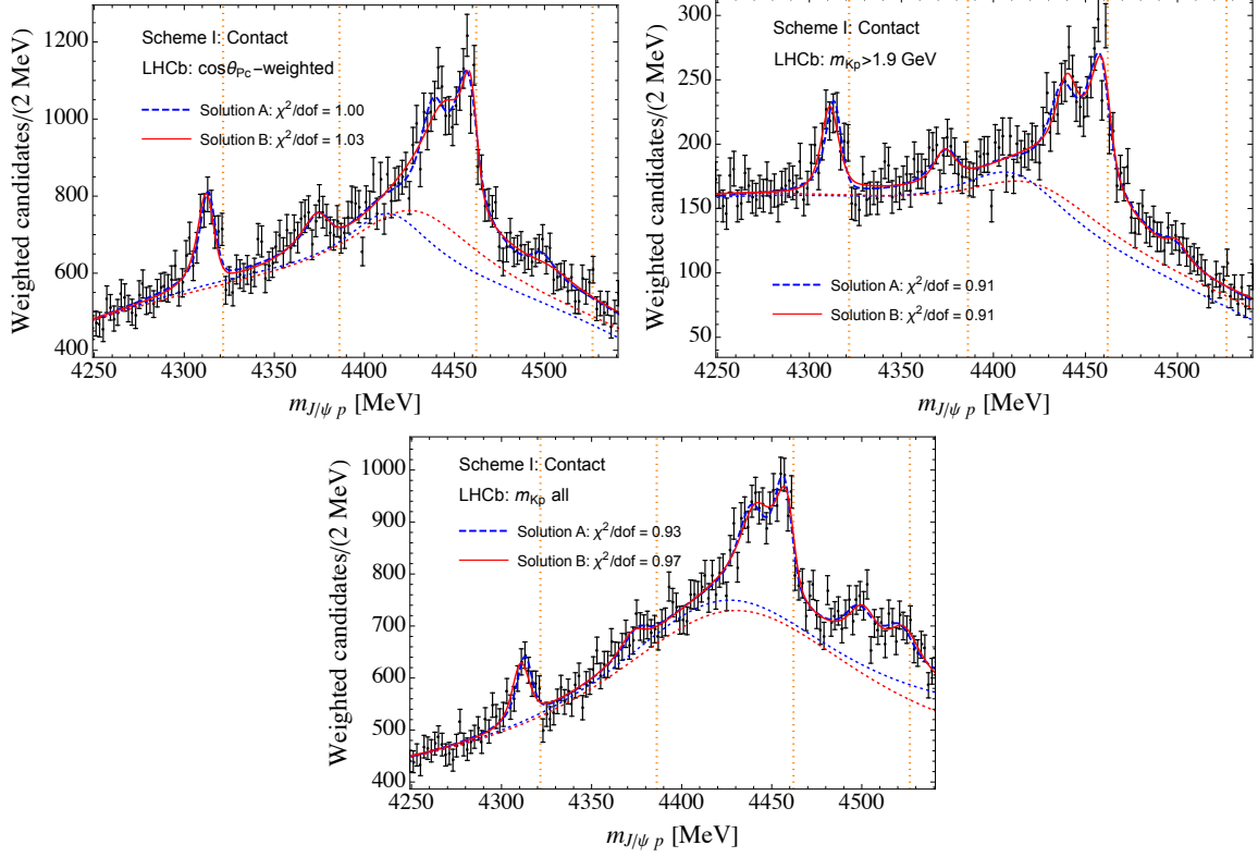
Figure 4. The best fits to the different experimental data [17] for both solution A (blue dashed curves) and solution B (red solid curves) of scheme I. The corresponding backgrounds are shown as red-dotted and blue-dotted curves, respectively. The vertical dashed lines from left to right are the \Sigma_c \bar{D} , \Sigma_c^* \bar{D} , \Sigma_c \bar{D}^* , and \Sigma_c^* \bar{D}^* thresholds, respectively.
