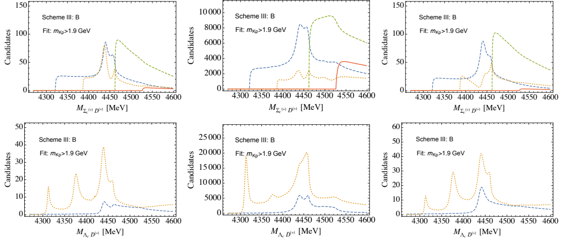
Figure 13. Predictions for the line shapes in the \Sigma_c^{(*)} \bar{D}^{(*)} and \Lambda_c \bar{D}^{(*)} channels based on the fit results of scheme III (solution B) for three different backgrounds. The left, middle and right columns show the results that are related to the blue, orange and green lines in figure 12, respectively. First row: mass distributions in the \Sigma_c \bar{D} (blue dashed curves), \Sigma_c^* \bar{D} (orange dotted curves), \Sigma_c \bar{D}^* (green dot-dashed curves), and \Sigma_c^* \bar{D}^* (red solid curves) channels. Second row: mass distributions in the \Lambda_c \bar{D} (blue dashed curves) and \Lambda_c \bar{D}^* (orange dotted curves) channels. Note the different scales on the y-axes of the different plots. No contribution from a possible background is included.
