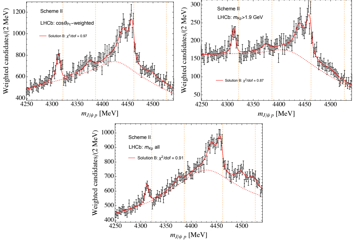
Figure 9. The best fits to the different experimental data [17] for solution B (red solid curves) of scheme II. The corresponding backgrounds are shown as red-dotted curves. The vertical dashed lines from left to right are the \Sigma_c \bar{D} , \Sigma_c^* \bar{D} , \Sigma_c \bar{D}^* , and \Sigma_c^* \bar{D}^* thresholds, respectively.
