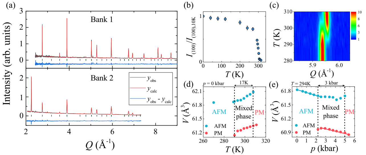
FIG. 1. (a) Rietveld refinement of powder neutron diffraction data collected at 10 K on banks 1 (backscattering) and 2 (90°) of HRPD, ISIS. Black tick marks indicate the reflections from the antiperovskite phase. The minor additional peaks, e.g., at Q = 5.1 \text{ \AA}^{-1} , are from MnO. (b) Temperature dependence of the fitted (100) peak intensity. (c) Thermodiffractogram of the (321) reflection. (d) Temperature dependence of the lattice volume at ambient pressure close to T_i for both the AFM and PM states. (e) Pressure dependence of the lattice volume at 294 K. Dotted vertical lines in (d) and (e) separate the single and mixed phase magnetic regimes, as described in the text. Solid lines in (e) are guides to the eye. Error bars in (d) and (e) are smaller than the symbol size.
