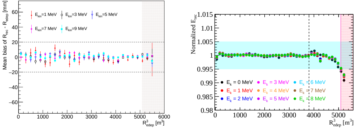
Figure 31: Left: Radial bias of the vertex reconstruction versus R^3 for different energies with deep learning. The two dashed lines are at y = \pm 20 mm, and the shadow corresponds to r > \text{fiducial volume} . Right: Uniformity of the normalized E_{rec} with respect to R^3 at various energies.
