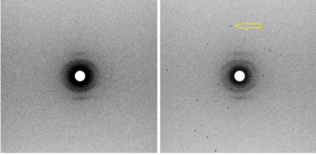
Figure 2: Neutron diffraction image, close to the beamstop, at t = 0.55 h (left), where the sample is still a clear solution, and at t=60.78 h (right), where Bragg peaks, due to the formation of the single crystal, can be observed. The yellow arrow points to the [2,-1,4] Bragg peak, whose intensity has been evaluated during the crystallization.
