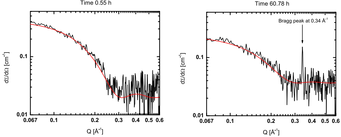
Figure 3: SANS curves for 30 mg/ml Lysozyme with 3 wt % of NaCl in D 2 O at two different times during the crystallization process. Black lines: experimental data, Red lines: fit to the data.
