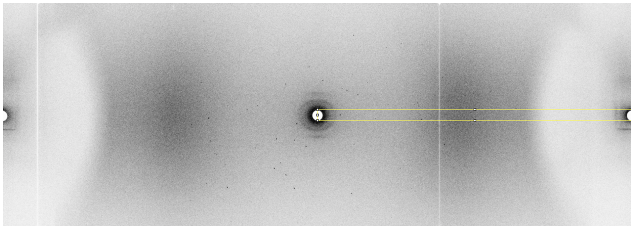
Figure 1: Neutron diffraction image, at t = 60.78 h. The yellow rectangle describes the strip where the scattering signal has been integrated to obtain the small angle scattering curve.
