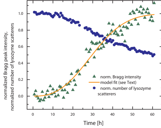
Figure 5: Temporal evolution of the normalized intensity of a single integrated Bragg peak (green triangles) and the normalized number of the Lysozyme scatterers (blue circles). The solid orange line describes the fit the data obtained with the JMAK mode.
