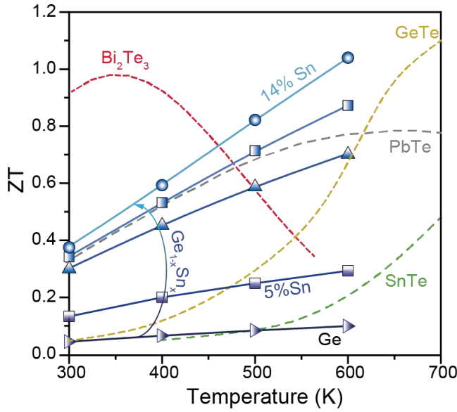
Figure 6. Benchmarking of ZT for GeSn alloys (this work) and \text{BiTe} , \text{PbTe} 35, pristine \text{SnTe} 7 and \text{GeTe} 5 thermoelectric materials in the temperature range 300-600K.
