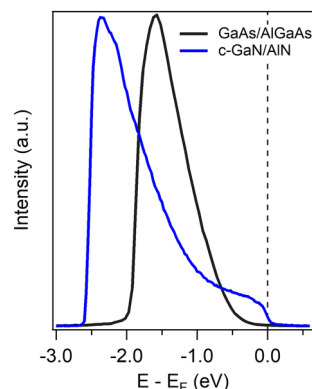
Figure 5. Comparison of the angle-integrated ARPES spectra at h\nu=7 eV from the GaAs/AlGaAs heterostructure and from the c-GaN/AlN heterostructure. At the Fermi energy (0 eV), only the spectra from the c-GaN/AlN heterostructure show a non-vanishing photoemission intensity, which can be reconducted to the presence of the QW states.
