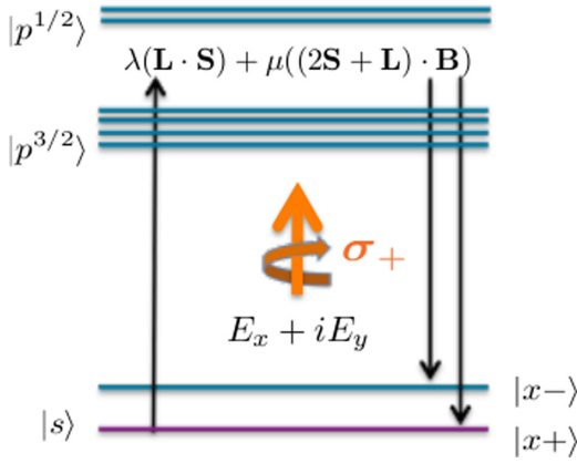
FIG. 2. The energy level scheme of the single-spin system.
