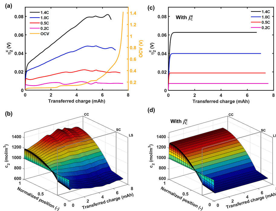
Fig. 4. (a) Comparison of electrolyte concentration overpotential ( \eta_2^c ) at various C-rates with the OCV as a reference. (b) The c_2 profile as a function of normalized position and transferred charge under a 0.5C charging current. (c) \eta_2^c at various C-rates with assumptions of j_c^u . (d) c_2 profile at 0.5C with j_c^u . The normalized position at 0, 0.26, and 1 represents the LS, SC, and CC interface.
