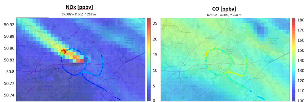
Figure 7: Evolution of industrial plume emissions of NO x and CO based on the EURAD-IM model overlaid by the field-derived Zeppelin observations.
