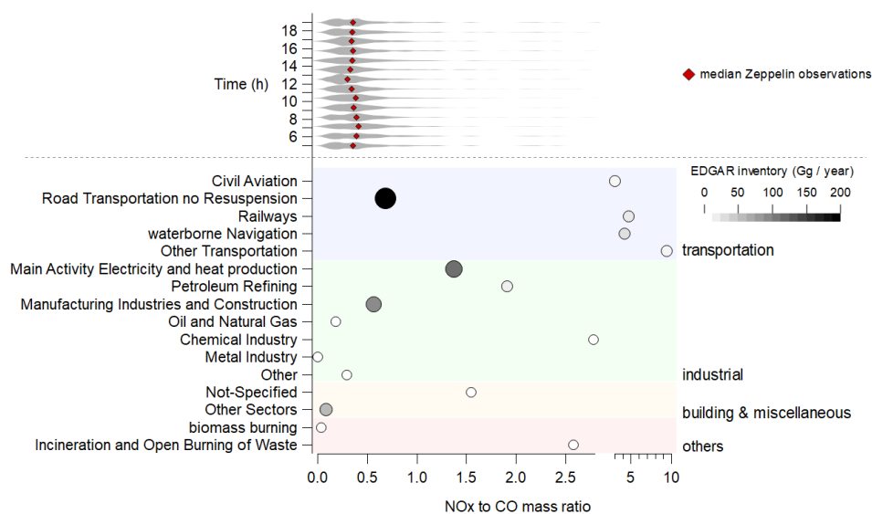
Figure 5: Distribution of the NO x to CO ratio (g / g) during the Zeppelin flights shown as a violin plot for measurements ranging from 250 to 450 meters in height. These ratios are compared to the ratios of different pollution sources following the EDGAR 2015 emission inventory. The size and color of the markers indicate the NO x emission strength for each EDGAR source.
