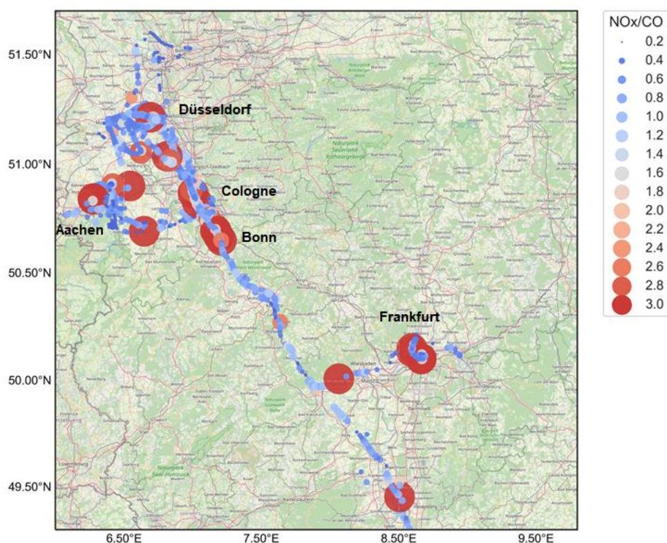
Figure 6: Identified areas of high NO x relative to CO emissions in Germany during the Zeppelin flights (© OpenStreetMap contributors 2021. Distributed under the Open Data Commons Open Database License (ODbL) v1.0.).
