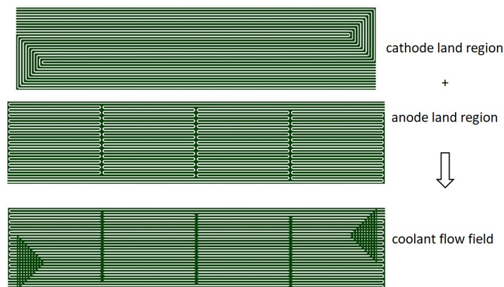
Figure 14. The resulting coolant flow field by combination of the land area of cathode and anode plate.
