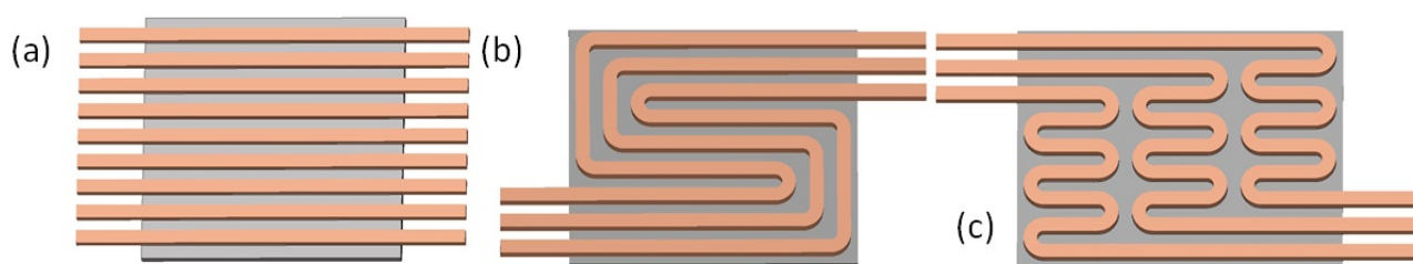
Figure 7. Example of the channel configurations generated by the toolbox. (a) Straight channel; (b) parallel serpentine; and (c) separate serpentine.
