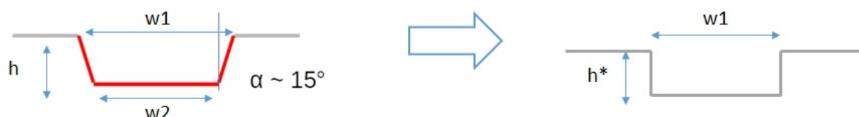
Figure 8. Realistic channel cross section and equivalent model cross section with identical hydraulic diameter. h and h^* —channel depth; w1 —channel top width; w2 —channel bottom width.
