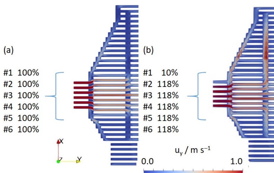
Figure 17. Fluid velocity (y-component) for the manifold region of the anode plate (MAX condition); cross section at half anode channel depth. (a) Normal flow at the inlet channels and (b) partial blocking of channel #1.
