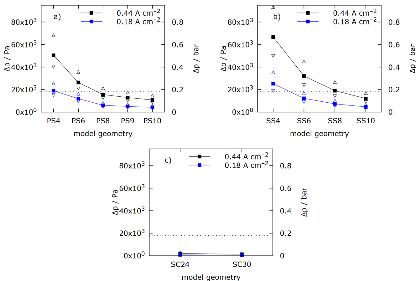
Figure 10. Pressure difference for the cathode flow fields. \Delta/\nabla show results for a variation of \pm 0.05 mm in channel depth. (a) parallel serpentine; (b) separate serpentine; (c) straight channels; dotted line at target value of 0.18 bar.
