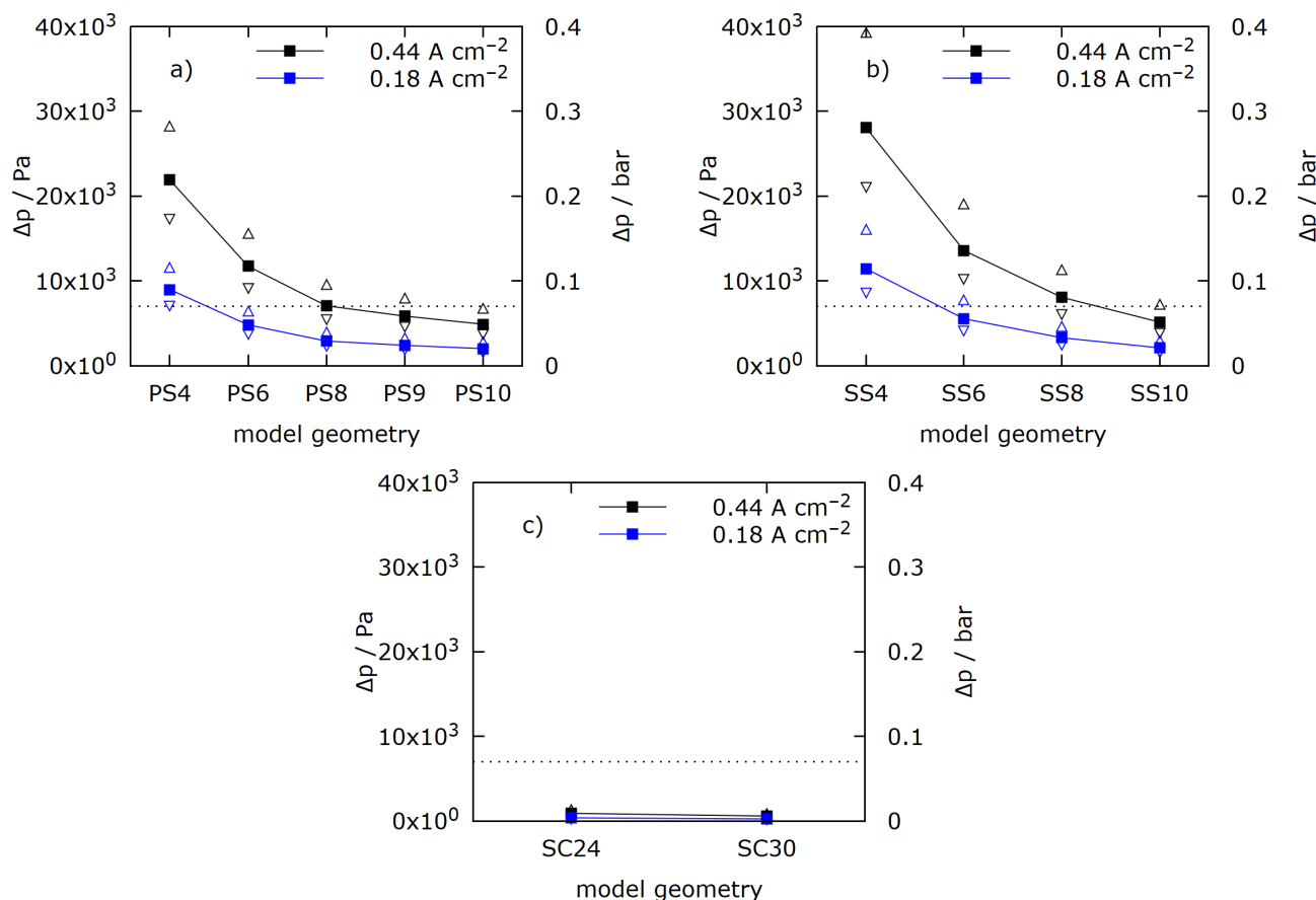
Figure 11. Pressure difference for the anode flow fields. \triangle/\nabla show results for a variation of \pm 0.05 mm in channel depth. (a) parallel serpentine; (b) separate serpentine; (c) straight channels; dotted line at target value of 0.07 bar.
