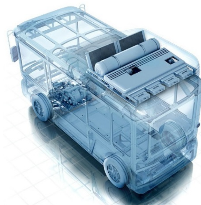
Figure 1. Sketch of a zero-emission light commercial vehicle with a fuel cell range extender mounted on the roof [21], reproduced with permission from e.GO REX GmbH.
