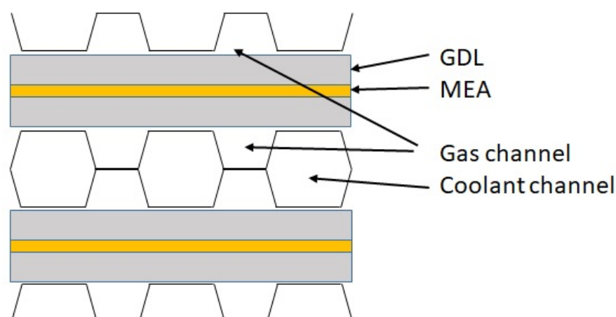
Figure 2. Cross section of two neighboring cells with resulting coolant channels in the middle. GDL—gas diffusion layer; MEA—membrane electrode assembly.
