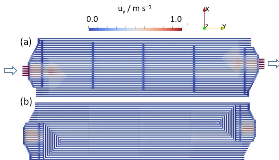
Figure 16. Fluid velocity (y-component) inside the coolant flow field for the MAX condition. (a) Cross section at half anode channel depth and (b) at half cathode channel depth.
