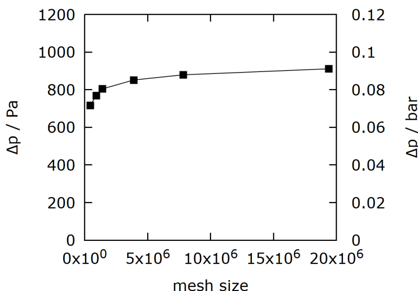
Figure 9. Pressure difference as a function of the mesh resolution for a parallel serpentine plate with a geometric area of 10 \text{ cm}^2 at 0.44 \text{ A cm}^{-2} .
