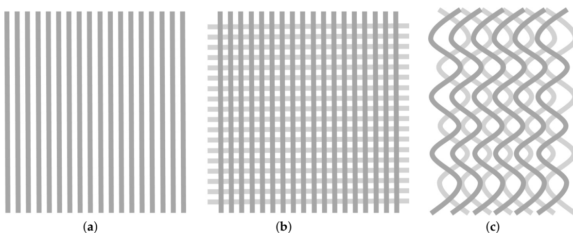
Figure 5. Sketch of common channel configurations for visualization of the contact area: (a) parallel, superimposed; (b) parallel, criss-crossed; and (c) wave-like, mirrored.
