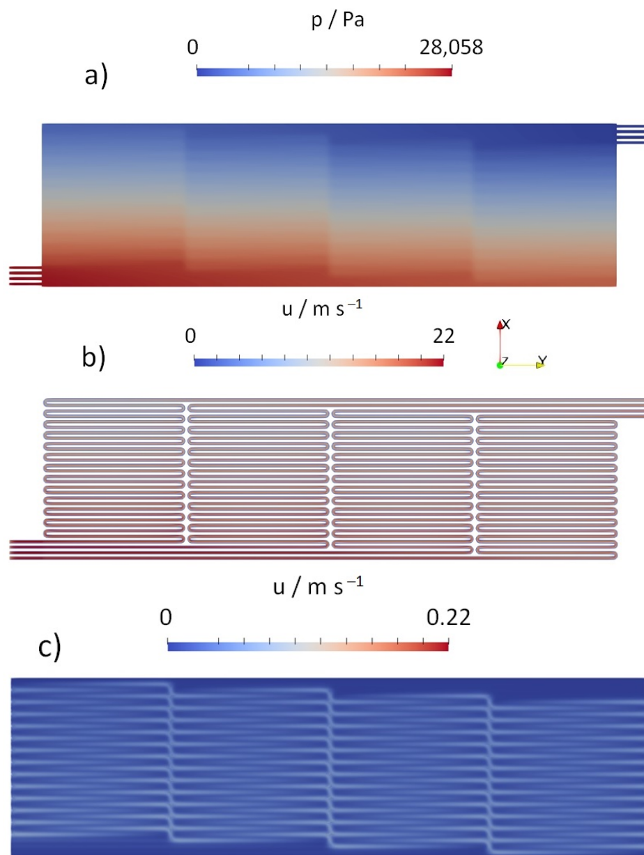
Figure 13. Flow distribution for the anode plate at 0.44 \text{ A cm}^{-2} . (a) Pressure distribution; (b) velocity (magnitude) at half channel depth; (c) velocity (magnitude) at half GDL height.
