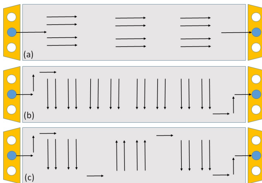
Figure 4. Coolant flow configuration. (a) In flow direction of hydrogen and air, (b) in cross-flow, and (c) cross-flow in separated blocks.
