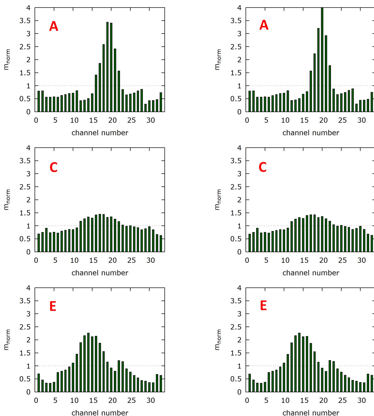
Figure 19. Normalized mass flow at positions A (inlet), C (middle), and E (outlet) for condition MAX. (Left) Normal flow at the inlet channels and (Right) partial blocking of channel #1.
