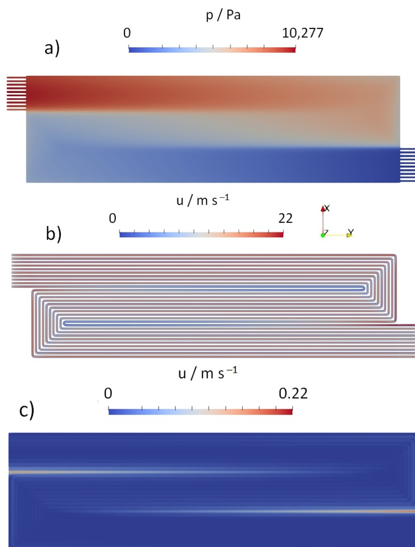
Figure 12. Flow distribution for the cathode plate at 0.44 \text{ A cm}^{-2} . (a) Pressure distribution; (b) velocity (magnitude) at half channel depth; (c) velocity (magnitude) at half GDL height.
