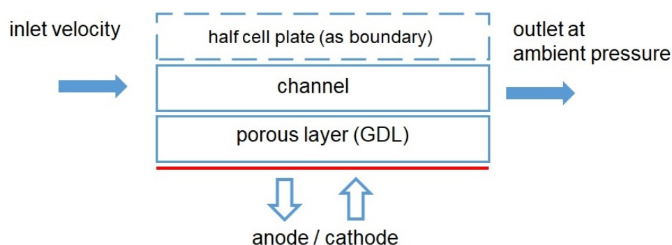
Figure 6. Sketch of the overall principle for the CFD simulations of anode and cathode plates.
