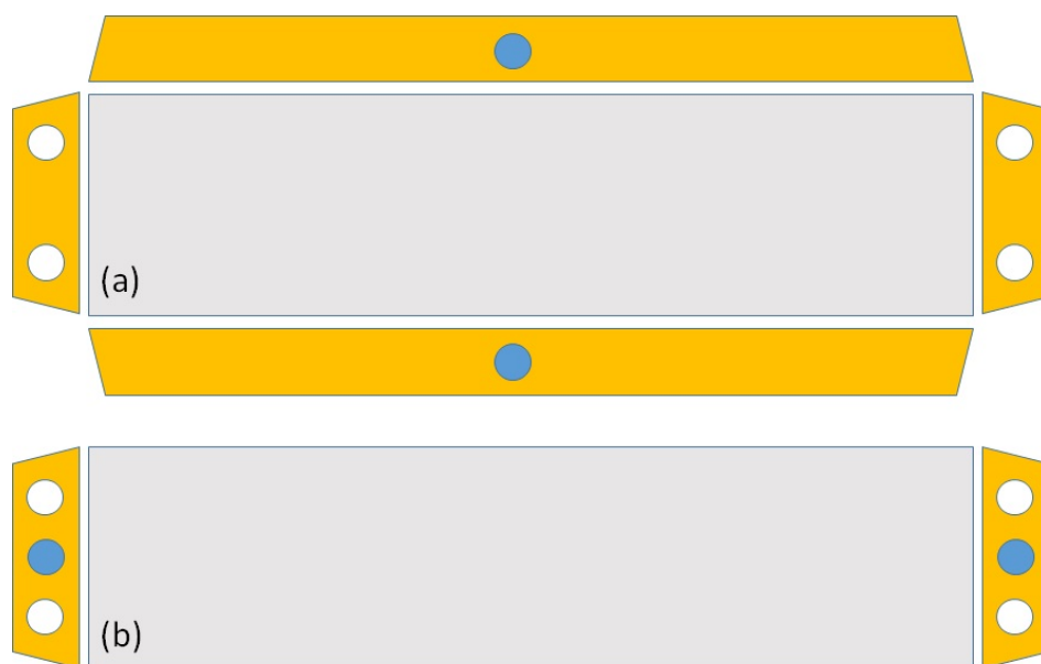
Figure 3. Location of stack manifolds with manifold areas shown in yellow, gas manifolds in white, and coolant manifolds in blue. (a) Separate cooling manifolds at the sides and (b) combined manifolds in the head and tail position.
