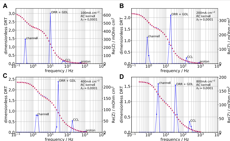
FIGURE 5 | DRT (solid line, left axis) calculated with the RC kernel using real part of the experimental PEMFC impedance (blue dots, right axis) for the current densities (A) 100, (B) 200, (C) 400, and (D) 800 \text{mA cm}^{-2} . Red open circles— \text{Re}(Z) reconstructed from the calculated DRT.
