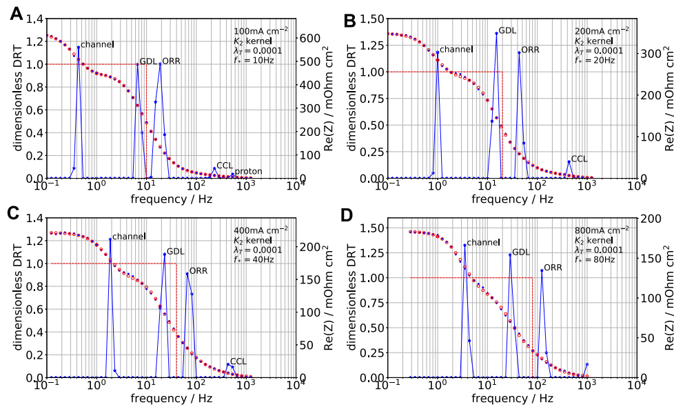
FIGURE 7 | DRT (solid line, left axis) calculated with the K_2 kernel using real part of the experimental PEMFC impedance (blue dots, right axis) for the current densities (A) 100, (B) 200, (C) 400, and (D) 800 \text{mA cm}^{-2} . Red open circles— \text{Re}(Z) reconstructed from the calculated DRT. Dashed line shows the plot of \alpha , Eq. 14, switching the K_2 kernel from TL- to RC-one at the frequency marked by vertical line.
