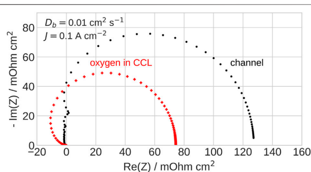
FIGURE 2 | Nyquist spectra of the channel impedance, Appendix Eq. A1 and of impedance of oxygen transport in the CCL (Kulikovsky, 2017).
