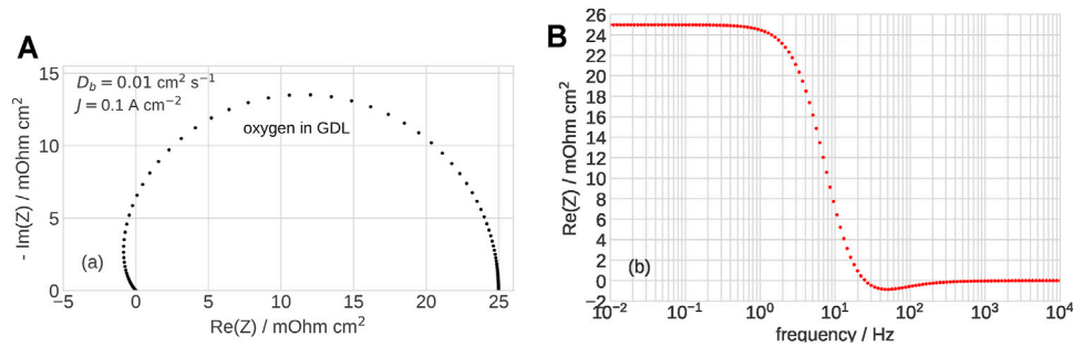
FIGURE 1 | (A) Nyquist spectrum of the gas-diffusion layer impedance, Eq. 10 . (B) Frequency dependence of the real part of impedance in (A) . Parameters for calculations are listed in Table 1 .
