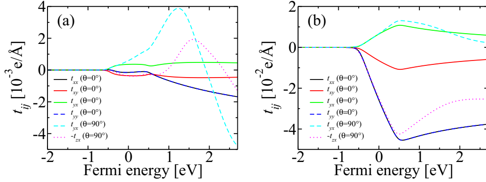
FIG. 3. (a) Magnonic spin-orbit torque (SOT) and (b) nonmagnonic SOT for \alpha^R = 720 \text{ meV } \text{\AA} and \Gamma = 136 \text{ meV} .
