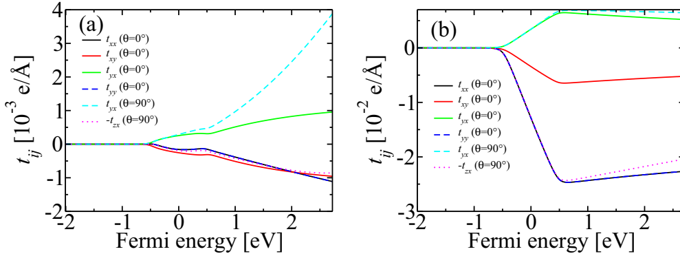
FIG. 6. (a) Magnonic spin-orbit torque (SOT) and (b) nonmagnonic SOT for \alpha^R = 360 \text{ meV } \text{\AA} and \Gamma = 136 \text{ meV} .
