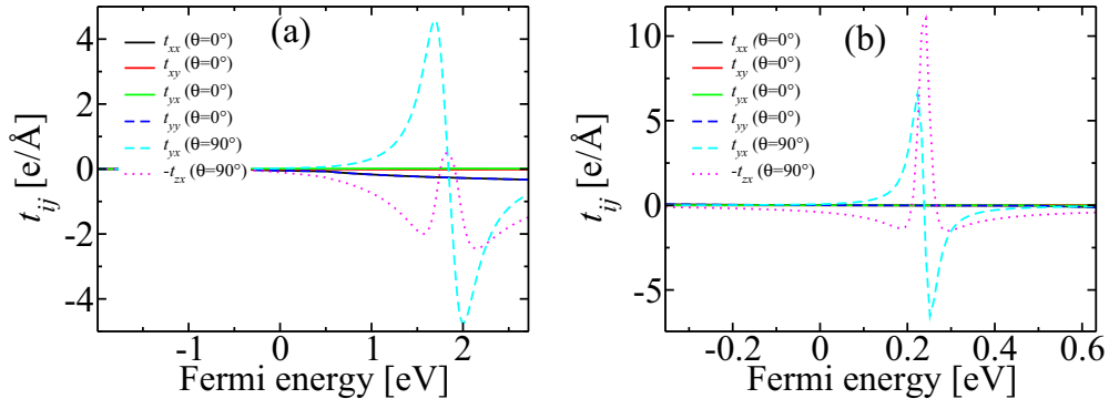
FIG. 9. Magnonic spin-orbit torque (SOT) for (a) \alpha^R = 720 \text{ meV } \text{\AA} and \Gamma = 25 \text{ meV} and (b) \alpha^R = 2 \text{ eV } \text{\AA} and \Gamma = 25 \text{ meV} .
