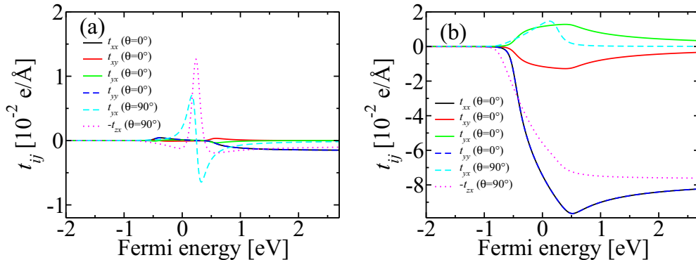
FIG. 8. (a) Magnonic spin-orbit torque (SOT) and (b) nonmagnonic SOT for \alpha^R = 2 \text{ eV } \text{\AA} and \Gamma = 136 \text{ meV} .
