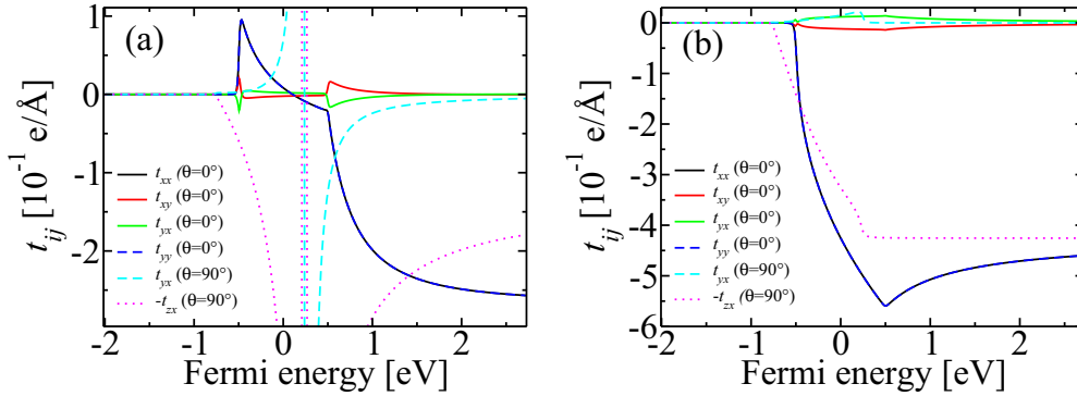
FIG. 7. (a) Magnonic spin-orbit torque (SOT) and (b) nonmagnonic SOT for \alpha^R = 2 \text{ eV } \text{\AA} and \Gamma = 25 \text{ meV} .
