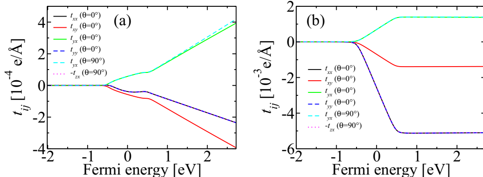
FIG. 4. (a) Magnonic spin-orbit torque (SOT) and (b) nonmagnonic SOT for \alpha^R = 72 \text{ meV } \text{\AA} and \Gamma = 136 \text{ meV} .
