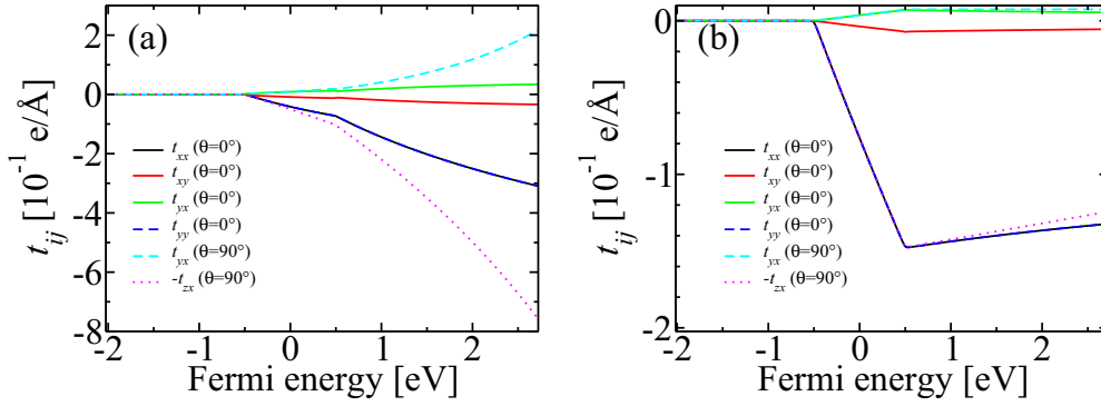
FIG. 5. (a) Magnonic spin-orbit torque (SOT) and (b) nonmagnonic SOT for \alpha^R = 360 \text{ meV } \text{\AA} and \Gamma = 25 \text{ meV} .
