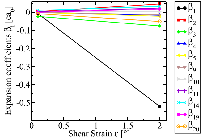
FIG. 9. Expansion coefficients \beta_i in Eq. (A9) of the odd torque in shear-strained PtMnSb obtained in GGA.
