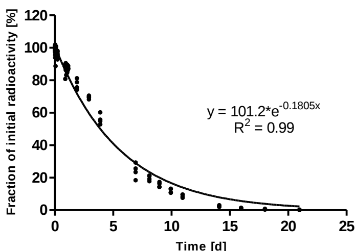
Figure 1. Deposition of ^{14}\text{C} -wMWCNT in a static water phase (M4 medium) over 21 days (d). The measured amount of radioactivity at t = 0 d was set to 100%. The proportion of decrease (%) of the initially applied radioactivity over the test period is shown. An exponential decay equation model was fitted to the experimental data. Data points represent single replicates ( n = 4 ). ( R^2 = coefficient of determination)
