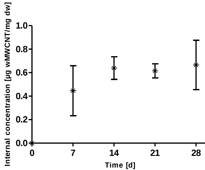
Figure 7. Uptake of ^{14}\text{C} -wMWCNT in a developing D. magna population over 28 days. Renewal of medium and simultaneous reapplication of ^{14}\text{C} -wMWCNT was performed once a week. Error bars indicate standard deviations for arithmetic average of 4 replicates ( n = 4 ).
