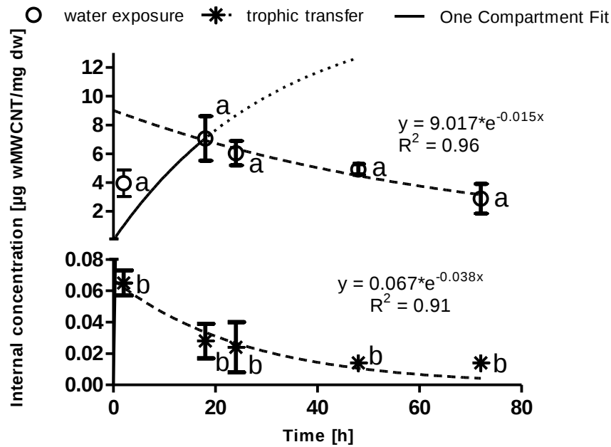
Figure 4. Uptake of ^{14}\text{C} -wMWCNT in D. magna after waterborne exposure (circles) and trophic transfer (asterisks). For trophic transfer green algae R. subcapitata was pre-loaded by radioactively labeled wMWCNT over 72 hours (h). A one compartment model ( R^2 = 0.96 ) was fitted to experimental data of uptake via water exposure (solid line, 0 h – 18 h). Additionally, the further course of the modelling is shown (dotted line). An exponential fit was adapted to areas with uptake decline for water exposure (dashed line, 18 h – 72 h) and trophic transfer (dashed line) scenario. Error bars indicate standard deviation ( n = 4 ). For all timepoints, mean values of uptake via water exposure and trophic transfer proved to be significantly different (visualized using the letters a and b, t-test, \alpha = 0.05 ).
