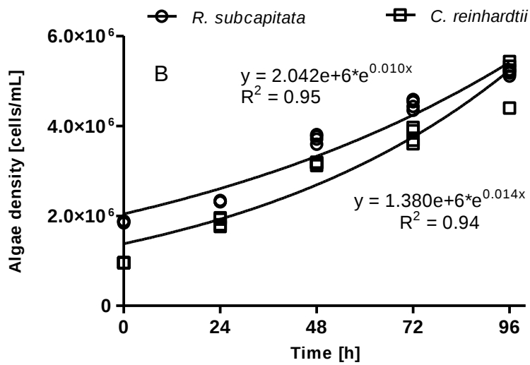
Figure 3. Weathered multi-walled carbon nanotube (wMWCNT) concentration linked to green algae over time. A 14 C-wMWCNT concentration of 100 µg L -1 was applied to suspensions of R. subcapitata (circles) and C. reinhardtii (squares) (A). The mean values and standard deviations are given (n = 4). For all timepoints, mean values for uptake of wMWCNT in R. subcapitata and C. reinhardtii proved to be significantly different (visualized using the letters a and b, t-test, α = 0.05). An exponential fit was plotted for the corresponding growth curves, algae density (cells mL -1 ) was measured over time in uptake experiment (B). Growth rates for C. reinhardtii and R. subcapitata are µ = 0.014 h -1 and µ = 0.010 h -1 , respectively. A significant difference over time was identified (two-sample t-test). Data points represent single replicates (n = 4).
