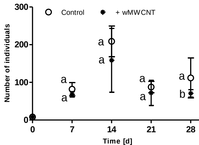
Figure 6. D. magna population dynamics. In 800 mL M4 medium, a population of D. magna developed from initially 5 neonate and 3 adult animals over 28 days. D. magna were fed daily 0.5 mg carbon (green algae). Two wMWCNT concentrations were tested: 0 \text{ mg L}^{-1} (Control, circles) and 0.1 \text{ mg L}^{-1} (asterisks). Total number of individuals over time is given. Error bars indicate the standard deviation on the mean of four replicates ( n = 4 ). The combination of the letters a and b visualizes the identified significant difference (t-test, \alpha = 0.05 ).
