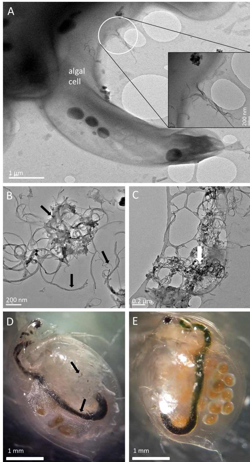
Figure 2 (A – D): Transmission electron microscopy (TEM) images of wMWCNT in association with green alga R. subcapitata (A), wMWCNT dispersion ( 0.1 \text{ mg L}^{-1} ) (B) and excreted wMWCNT by D. magna after uptake period of 24 h (C). D and E show the light microscopy image of an adult D. magna exposed to 100 \text{ µg wMWCNT L}^{-1} and without exposure over a period of 72 h, respectively.
