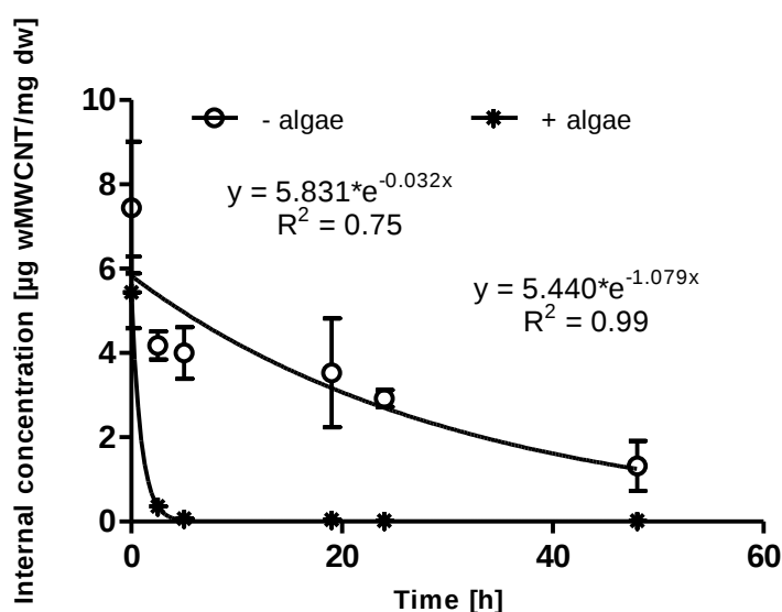
Figure 5. Internal ^{14}\text{C} -wMWCNT concentration in D. magna after depuration over a period of 48 hours (h). Start wMWCNT-concentration in -algae (circles) and +algae (asterisks) scenario was calculated from 5 and 7 replicates, respectively. Daphnia were fed with green algae (0.1 mg carbon) after transfer to clean medium. Elimination rates ( k_2 ) were determined (exponential fit) to 0.032 \text{ h}^{-1} and 1.079 \text{ h}^{-1} in scenario -algae and +algae, respectively. Elimination in presence and absence of algae was significantly different over time (two-sample t-test). Error bars indicate standard deviation ( n = 4 ).
