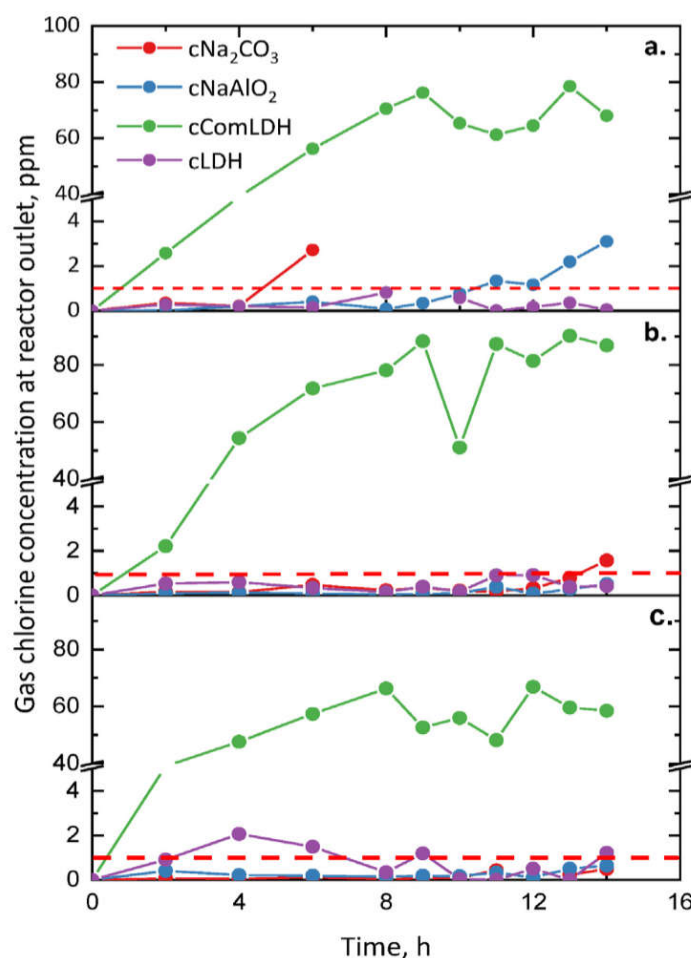
Figure 6. Concentration of HCl in the effluent at 400 (a), 500 (b), and 600 °C (c) for each sorbent. (The horizontal red dashed line represents the 1 ppm breakthrough threshold) [109].
