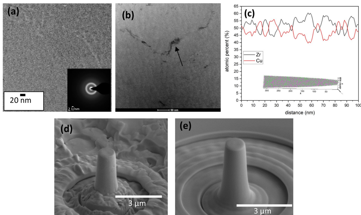
Figure 1: (a) TEM image of \text{Cu}_{50}\text{Zr}_{50} nanoglass. Inset shows a selected area electron diffraction pattern with the diffused halo confirming the amorphous nature of the sample. (b) STEM-HAADF image showing the Cu–Zr nanoglass, arrow indicates a porous region. (c) Composition profile along the length of the APT tip (shown in the inset) obtained using a cylinder of diameter 3 nm. Micro-pillars of (d) nanoglass and (e) metallic glass before compression imaged by SEM.
