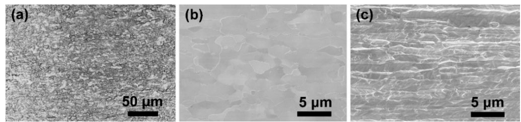
Figure 5. The microstructure of the original W foil. (a) Metallographic structure of the etched rolling surface, and SEM microstructure of (b) the rolling surface and (c) the side surface.
