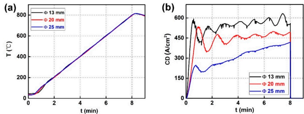
Figure 3. (a) FAST joining process and (b) the current density (CD) change curves of the W foil laminates with different diameters.
