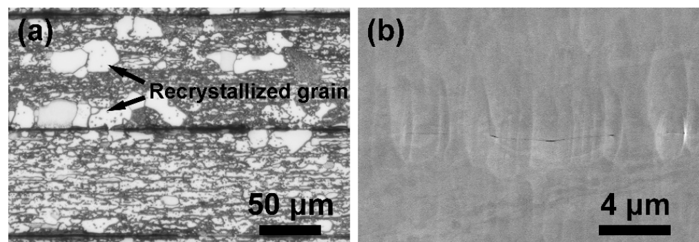
Figure 9. (a) The metallographic structure and (b) a representative W–W interface of the W foil laminate FAST joined in an artificial operation mode.
