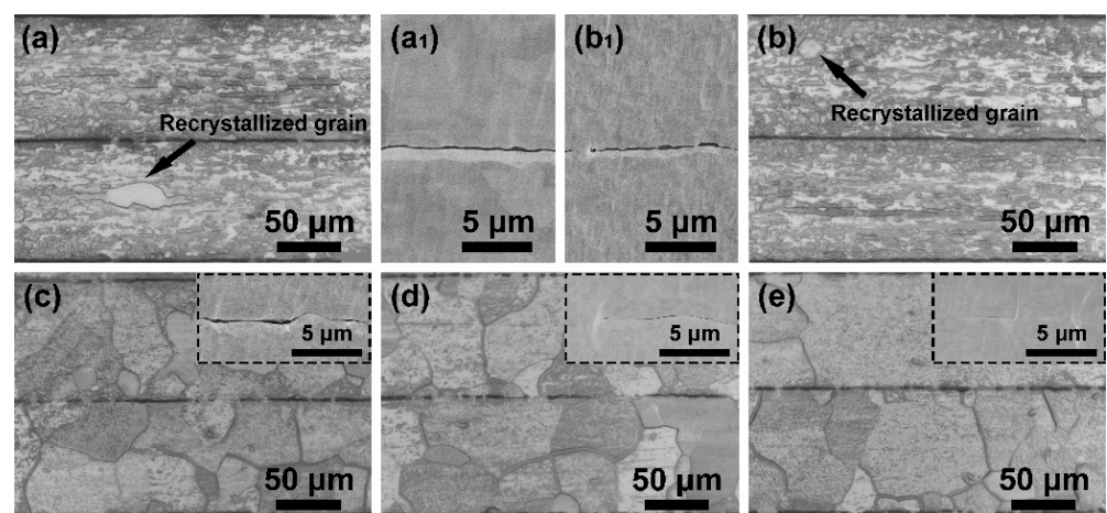
Figure 6. The metallographic structures viewed from transverse direction of the W foil laminates joined at different temperatures (a) 600 °C, (b) 800 °C, (c) 1000 °C, (d) 1200 °C, and (e) 1400 °C. (a 1 , b 1 ) and the insert images are the SEM images of the corresponding interfaces.
