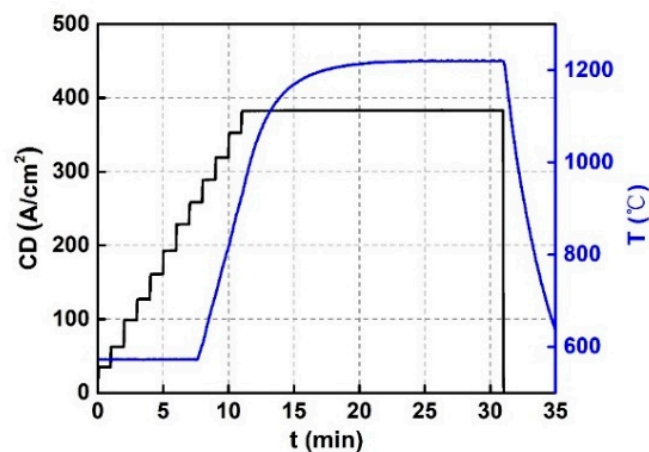
Figure 4. The change curves of current density (CD) and temperature during the FAST joining process of W foil laminate in an artificial operation mode.
