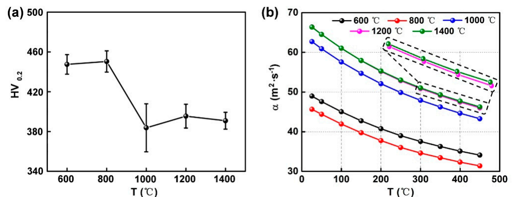
Figure 7. (a) The Vickers hardness and (b) the thermal diffusivity of the W foil laminates as a function of the joining temperature.
