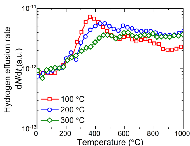
Figure 9. Hydrogen effusion rate dN/dt as a function of temperature (heating rate 20\text{ }^\circ\text{C/min} ) for \text{PO}_x/\text{Al}_2\text{O}_3 stacks deposited at different temperatures. The measurements were done in vacuum, and the apparatus was baked out prior to the measurements to eliminate influences of background water on the measured hydrogen effusion spectra.
