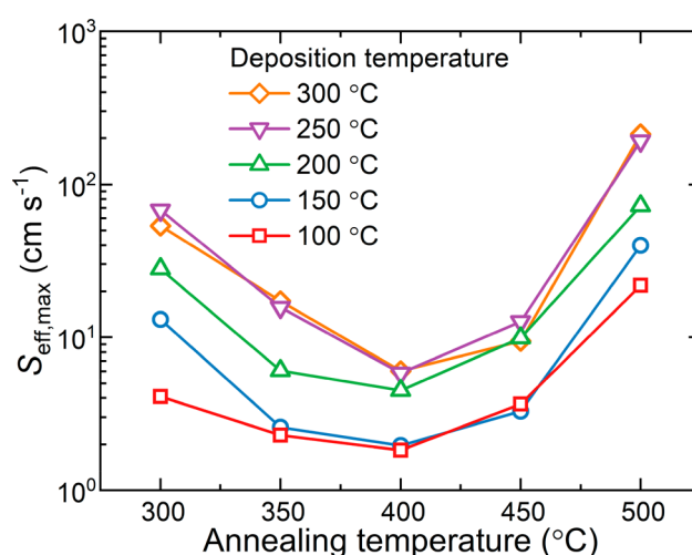
Figure 2. Maximum effective surface recombination velocity ( S_{\text{eff,max}} ), as a function of annealing temperature for \text{PO}_x/\text{Al}_2\text{O}_3 stacks on 280 \Omega\text{m} -thick double-side-polished 3.3–3.7 \Omega\text{cm} n -type FZ Si wafers with deposition temperatures ranging from 100 to 300 ^\circ\text{C} . Annealing was performed at consecutively higher annealing temperatures starting at 300 ^\circ\text{C} in steps of 50 ^\circ\text{C} up to 500 ^\circ\text{C} on the same samples for 10 min in \text{N}_2 .
