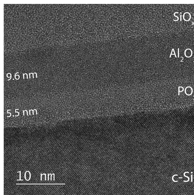
Figure 6. Cross-sectional bright-field TEM image of a \text{PO}_x/\text{Al}_2\text{O}_3 stack deposited at 100 °C on c-Si. The sample was annealed at 400 °C. \text{SiO}_x was deposited on top of the stack to protect the layers during the TEM lamella preparation by FIB.
