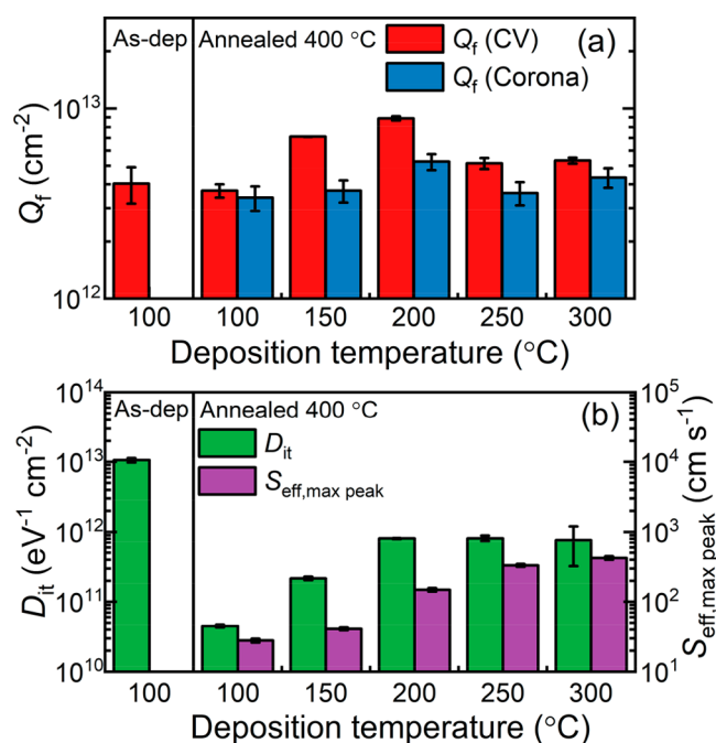
Figure 5. Interface properties of \text{PO}_x/\text{Al}_2\text{O}_3 stacks deposited at various deposition temperatures annealed at 400 °C and an as-deposited stack deposited at 100 °C. (a) Fixed charge density ( Q_f ) as determined by CV measurements and corona-lifetime experiments. (b) Interface defect density ( D_{it} ) as determined by CV measurements and the peak value of the maximum surface recombination velocity S_{\text{eff,max peak}} determined from the data in Figure 4. This value is a measure for the surface defect density.
