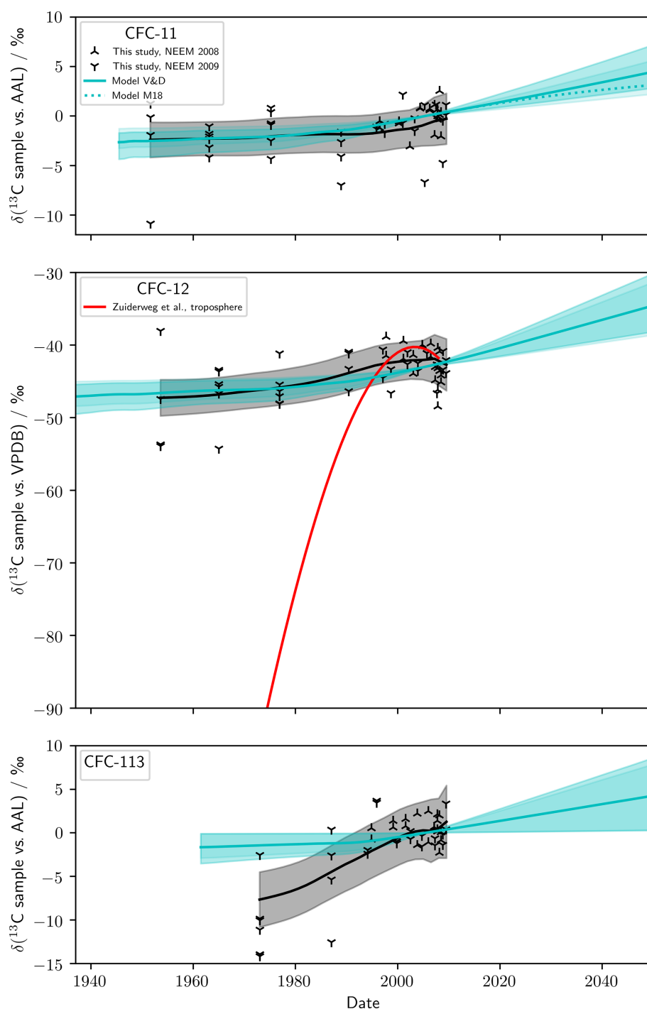
Figure 4. Measured and modelled \delta_{\text{T}}(^{13}\text{C}, \text{CFC-11}) , \delta_{\text{T}}(^{13}\text{C}, \text{CFC-12}) , and \delta_{\text{T}}(^{13}\text{C}, \text{CFC-113}) . The smoothed trend and 95 % confidence intervals for measured \delta_{\text{T}}(^{13}\text{C}) are shown by the solid black line and grey shading, respectively. The solid blue line shows the mean modelled \delta_{\text{T}}(^{13}\text{C}) for the Velders and Daniel (2014) scenario (V&D) and the two stratosphere–troposphere exchange parameterisations (Holton, 1990; Appenzeller et al., 1996). \epsilon_{\text{app}}(\text{high-latitude}) was used for each CFC. Blue shading shows the 95 % uncertainty envelope for the Holton (1990) and Appenzeller et al. (1996) parameterisations. For CFC-11 only, the dotted blue line shows the mean modelled \delta_{\text{T}}(^{13}\text{C}) for the M18 scenario, with the uncertainty envelope omitted for clarity. For CFC-12, the red line shows \delta_{\text{T}}(^{13}\text{C}) as predicted by Zuiderweg et al. (2013) (amending a typo in the coefficients presented by Zuiderweg et al. (2013), \delta_{\text{T}}(^{13}\text{C}, \text{CFC-12}) = -265.4280 + 4.8315x + (7.8555 \times 10^{-5})x^2 - (3.3070 \times 10^{-4})x^3 , where x = t - 1933.5 , and t gives the date).
