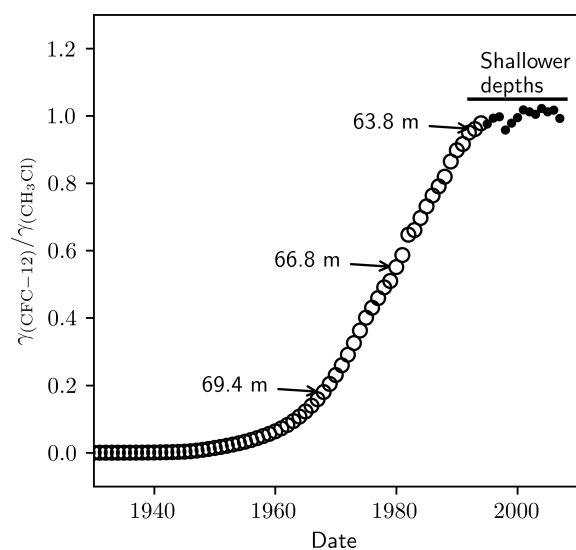
Figure C1. The ratio of the tropospheric mole fraction of CFC-12 to \text{CH}_3\text{Cl} . Circles were taken from Butler et al. (1999). The dots were calculated using data from the National Oceanic and Atmospheric Administration – Halocarbons & other Atmospheric Trace Species (NOAA-HATS). The annotations indicate the points on the curve that correspond to different depth samples in the NEEM 2009 firn profile.
