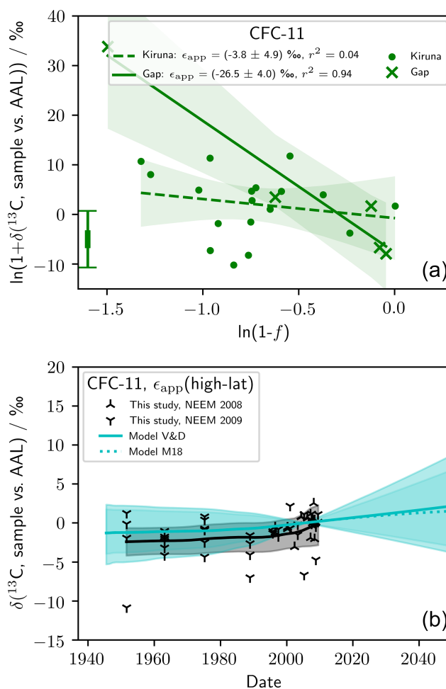
Figure D1. (a) Rayleigh plot showing observations of \delta(^{13}\text{C}, \text{CFC-11}) and derived \epsilon_{\text{app}}(\text{CFC-11, high-latitude}) and \epsilon_{\text{app}}(\text{CFC-11, mid-latitude}) . (b) Also shown is measured and modelled \delta_T(\text{CFC-11}) (see Fig. 4 and Sect. 2.5 for a description of the model). The model was forced with \epsilon_{\text{app}}(\text{CFC-11, high-latitude}) . The error bar in the bottom left corner of (a) shows the median repeatability of the reference gas measurements over the measurement days and the median error deriving from the fractional release factor.
