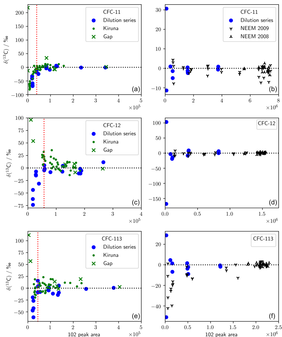
Figure A1. Dilution series for the analytical methodologies used in this work. (a, c, e) Method A, which was used to measure stratospheric samples. The dotted red line shows the lower limit of m/z 102 peak areas that were retained. (b, d, f) Method B, which was used to measure firm air. Dilution series measurements are relative to SX-0706077 (2009 air), and stratospheric and firm air measurements are relative to AAL (2005 air).
