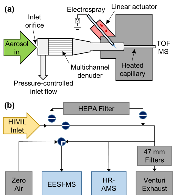
Figure 1. (a) Schematic of the EESI-MS source, pressure-controlled inlet, and automated capillary stage; (b) EESI-MS and HR-AMS sampling configuration flown during FIREX-AQ. The linear actuator controlling the capillary position is opposed by a spring (not drawn) to allow for bidirectional control of the capillary position, as shown by red arrows. The valves in (b) are drawn in the positions used for ambient sampling
