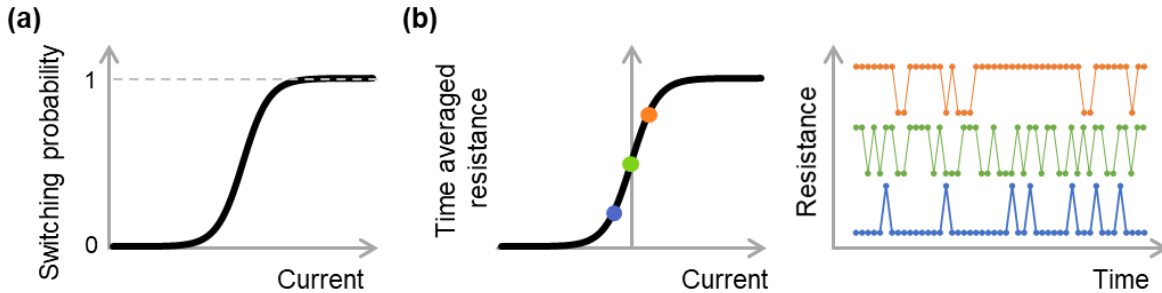
Figure 15. Two approaches to utilize stochastic behavior of SOT devices. (a) The first approach, where switching probability of binary devices is utilized. (b) The second approach, where the thermal fluctuation of superparamagnetic devices controlled by SOT is utilized. The right graph shows the temporal change of device resistance at three levels of applied current, indicated by closed circles with the same color in the left graph.
