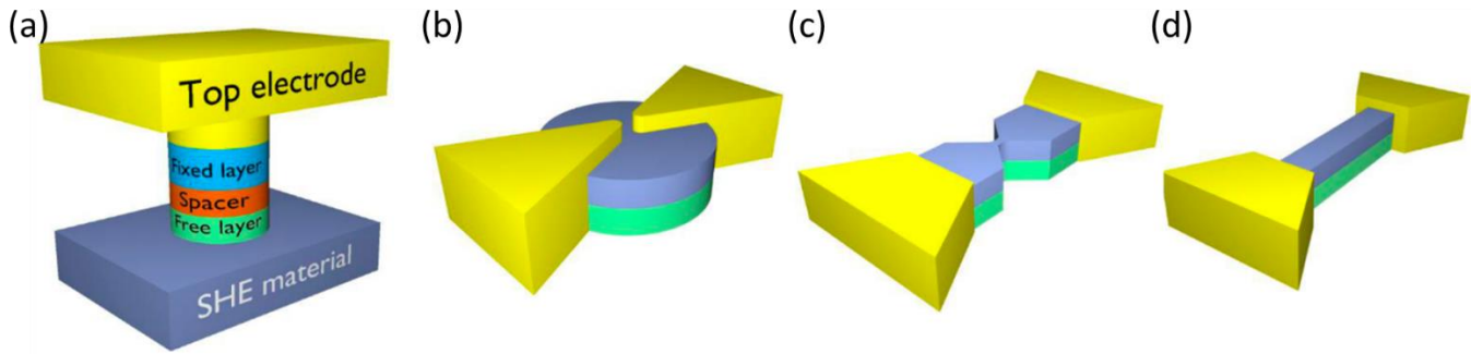
Figure 18. Device schematics of SOT nano-oscillators. (a) nano-pillar; (b) nano-gap; (c) nano-constriction; (d) nanowire
