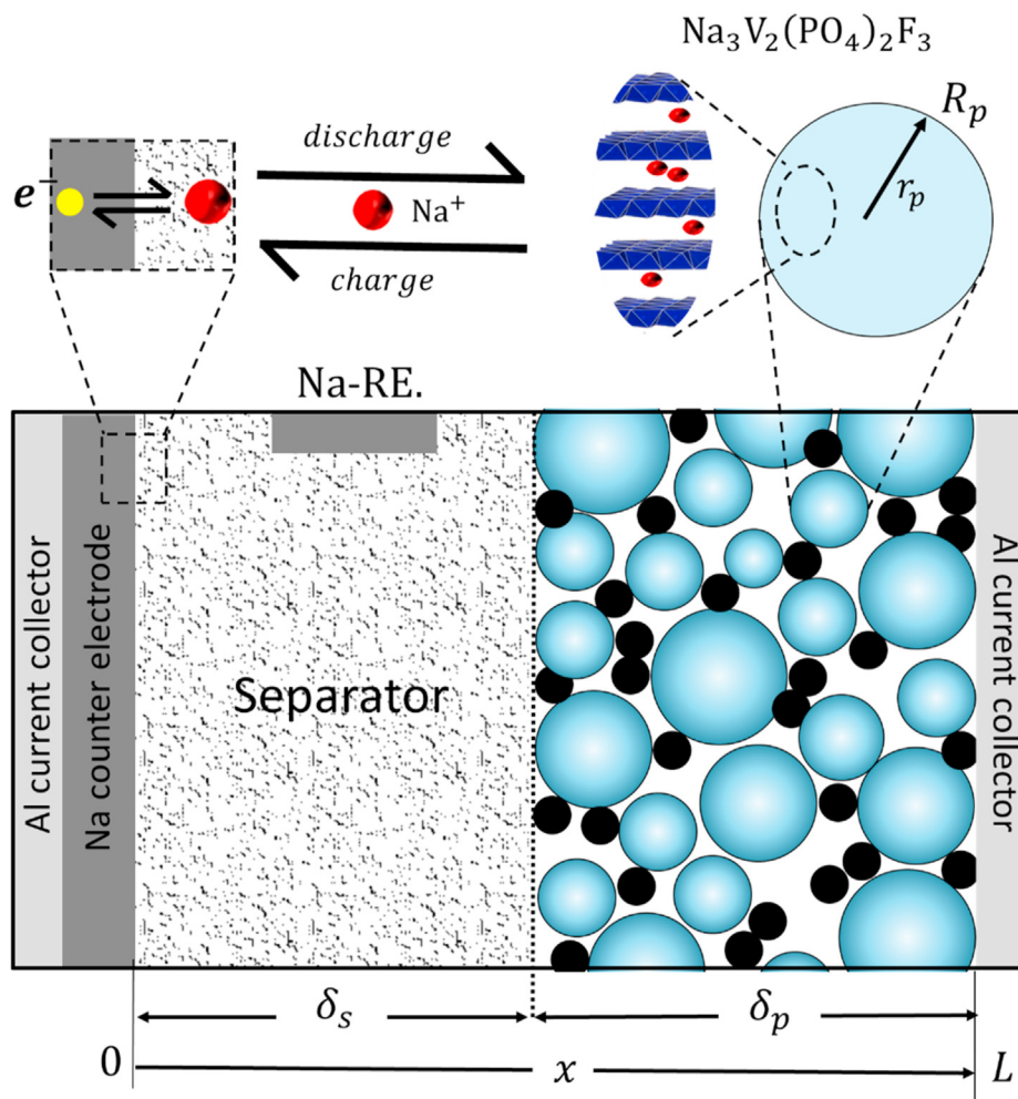
Fig. 1. Three electrode half-cell setup used in GITT experiments. The blue circles represent the NVPF active electrode material, and the black circles represent the carbon-based conductive filler. At the particle scale and at the electrode interface, the charge insertion mechanisms are shown. The red and yellow spheres represent sodium cations and electrons, respectively. (For interpretation of the references to colour in this figure legend, the reader is referred to the Web version of this article.)
