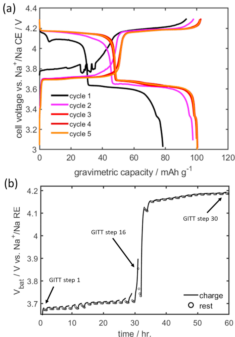
Fig. 2. Experimental results obtained for the Na//NPVP SIB half-cell. Formation cycles recorded at a CC of 0.1 mA ( 0.039 \text{ mA cm}^{-2} , C/30) (a). Overview of 30 GITT steps during (de)sodiation (solid lines) at a CC of 0.1 mA and OCV rest periods (circles) (b). All measured 30 GITT steps are shown.
