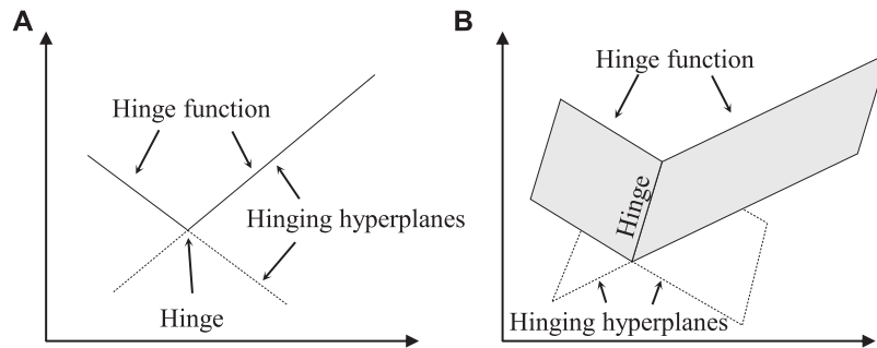
FIGURE 2 | Sketch of hinging hyperplanes, the hinge, and the hinge function are illustrated in two dimensions (A) and three dimensions (B) , adapted from Pucar and Sjöberg (1998).
