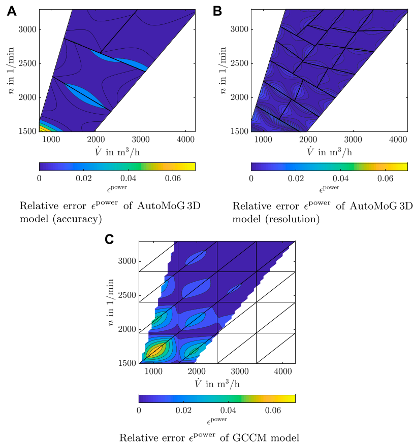
FIGURE 7 | Relative error of the AutoMoG 3D model with same accuracy (A) and comparable resolution (B) compared to the relative error of the generalized-convex-combination method (GCCM) model (C) for the power function of a variable-speed pump.
