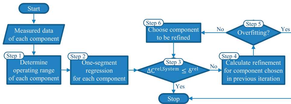
FIGURE 1 | AutoMoG 3D for multidimensional automated model generation using hinging-hyperplane trees. \Delta C^{\text{rel, System}} is the relative error of the overall multi-energy system model. \delta^{\text{rel}} is the allowed relative error of the overall multi-energy system model as specified by the user.
