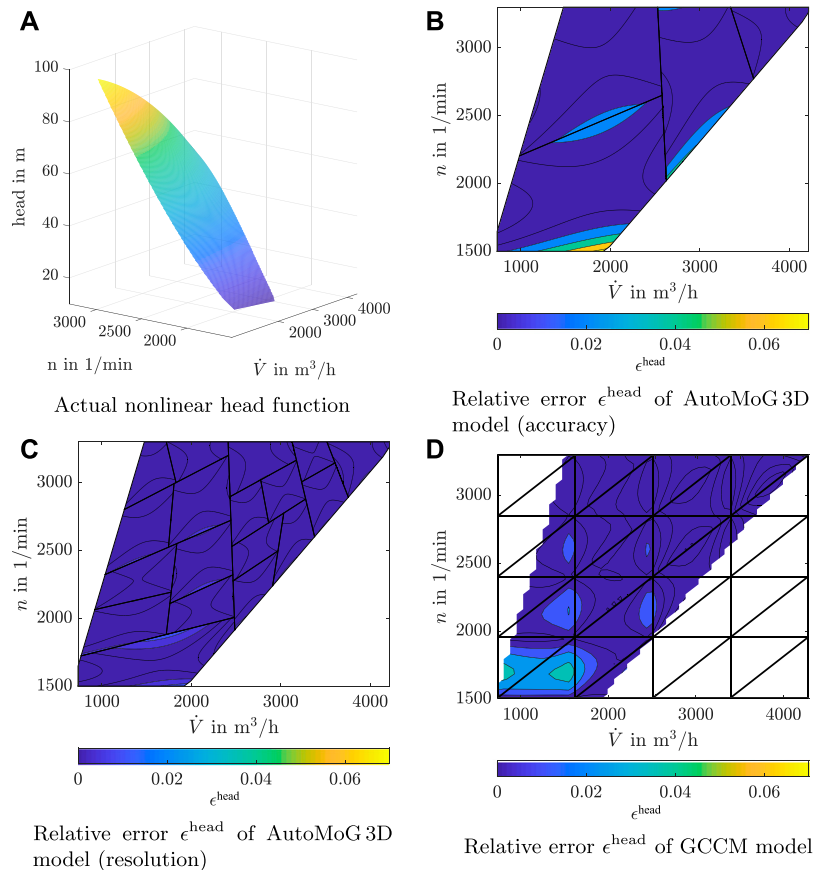
FIGURE 8 | Actual nonlinear head function of a variable-speed pump (A), and the relative errors of the AutoMoG 3D model with same accuracy (B) and comparable resolution (C) compared to the relative error of the generalized-convex-combination method (GCCM) model (D) for the head function of a variable-speed pump.
