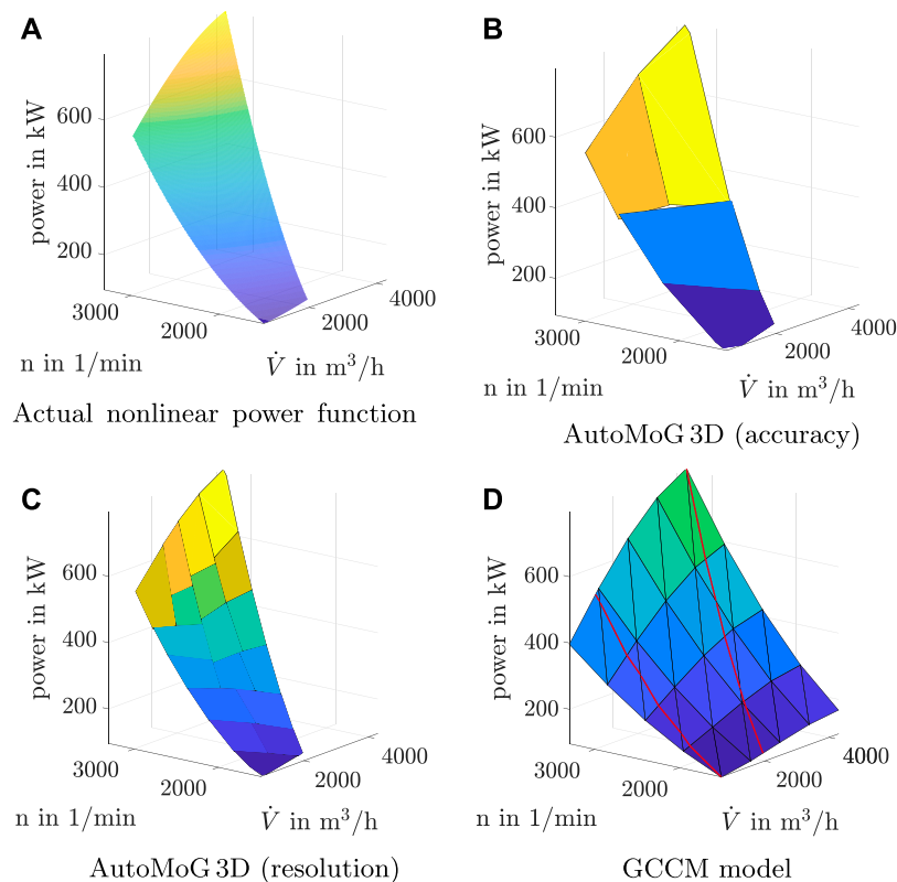
FIGURE 6 | Actual nonlinear power function of a variable-speed pump (A) , AutoMoG 3D model with the same accuracy as the model of the generalized-convex-combination method (GCCM model) (B) , AutoMoG 3D model with a comparable resolution as the GCCM model (C) , and the GCCM model used by Bahl et al. (2018) (D) . The power depends on the rotational speed n and the volumetric flow rate \dot{V} . The generalized-convex-combination method needs a rectangular grid, whereas AutoMoG 3D automatically considers the actual operating limits of the pump. The red lines in (D) show the actual operating limits. The color code only supports the visual differentiation of the piecewise-affine regions.
