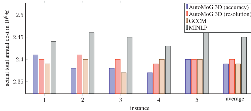
FIGURE 10 | Actual total annual cost for all instances and models. The actual total annual cost is determined by fixing the solution of every model and recalculating the total annual cost of this solution in the MINLP model. All MILP models find a better solution in all instances than the MINLP model finds within 48 h.
