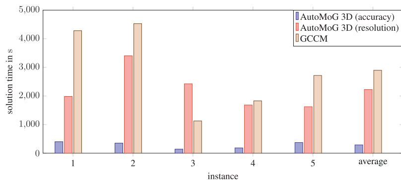
FIGURE 9 | Solution time to satisfy the optimality gap of 2% for all instances and all models except the MINLP model. The MINLP model did not fulfill the optimality gap in any instance at the time limit of 48 h. Therefore, there are no solution times for the MINLP model.
