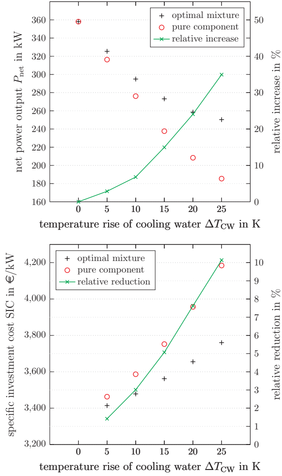
Figure 8: Net power output P_{\text{net}} (top) and specific investment cost SIC (bottom) of the optimal mixture and pure component for varying temperature rise of the cooling water \Delta T_{\text{CW}} . Additionally, the relative increase (top) and reduction (bottom) of the objective is shown, respectively.
