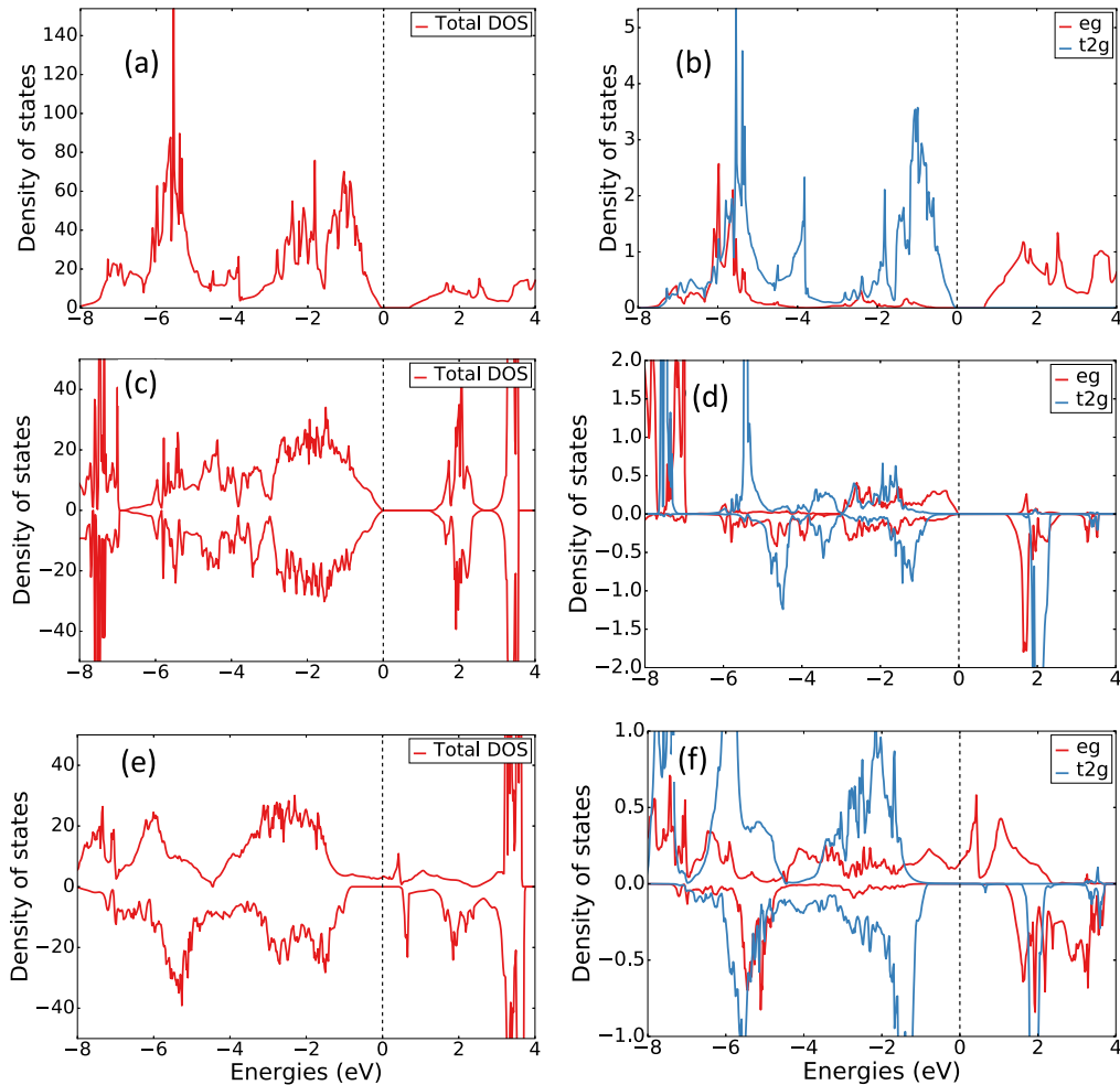
FIG. 8. Total and partial densities of states for (a), (b) Pm\bar{3}m (NM) at V = 8.96 Å³/atom (LS state), for (c), (d) Pm\bar{3}m (AFM) with V = 11.51 Å³/atom (HS state), and for (e), (f) Pm\bar{3}m (FM) at V = 10.18 Å³/atom (IS state). Zero energy corresponds to the Fermi energy. Positive and negative values of DOS correspond to spin-up and spin-down.
