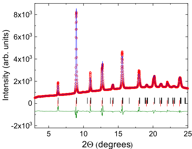
FIG. 4. The Rietveld refinement of the synchrotron x-ray diffraction data for \text{La}_{0.75}\text{Ba}_{0.25}\text{CoO}_{2.9} measured at 50 K and 16 GPa, with experimental data in open circles, the calculated pattern in blue, and the difference curve in green. The tick marks indicate Bragg peak positions for R\bar{3}c (black) and Pm\bar{3}m (red) phases.
