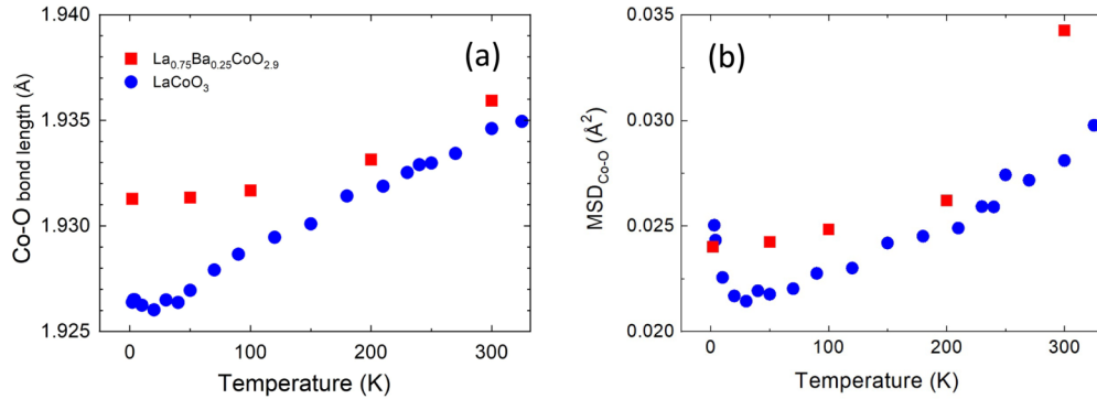
FIG. 3. The temperature dependence of (a) Co-O bond length and (b) MSD of Co-O bond, both obtained from the Rietveld refinement of the neutron powder diffraction data for \text{La}_{0.75}\text{Ba}_{0.25}\text{CoO}_{2.9} and \text{LaCoO}_3 samples.
