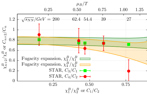
FIG. 6. Our continuum estimates of the fluctuation-ratios \chi_3^B/\chi_1^B and \chi_4^B/\chi_2^B compared with STAR data on net-proton fluctuations from Ref. [88]. Both values of the fluctuations and the trend as a function of baryon density are consistent.
