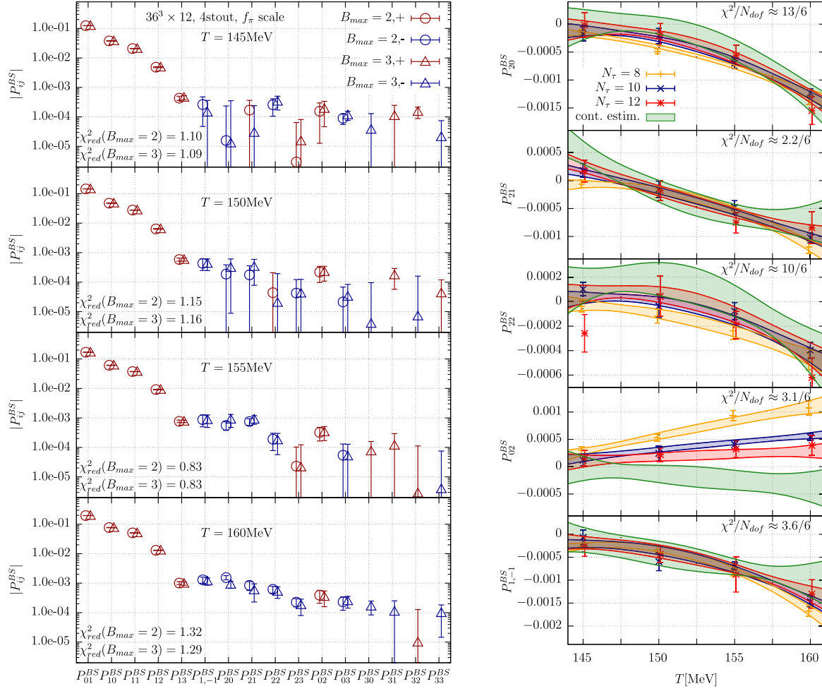
FIG. 1. Left: The four panels refer to four temperatures, each showing the obtained coefficients of the fugacity expansion on a logarithmic scale (negative values are shown in blue). Only the leftmost five are accounted for by the ideal HRG model. The next seven appear in the next order, which we use later for phenomenology. For the next order (last four coefficients with B = 3 ) we see no stable signal. There are two symbols per coefficient, triangles for the complete fit and circles for the case without the B = 3 part. The data refer to our finest lattice spacing. Right: Example for the combined continuum extrapolation of the extracted coefficients.
