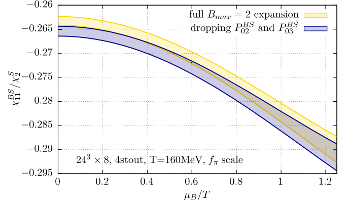
FIG. 4. Multi-kaon interactions have a negligible impact on the fluctuations ratios studied in this work. Here we show the effect of dropping the multi-kaon sectors from the fugacity expansion, demonstrated on the N_\tau = 8 data, at T = 160 MeV, where they are the largest in our temperature range. Note also that, on the N_\tau = 8 lattices, the magnitude of the multi-kaon sectors is larger than our continuum estimate for them.
