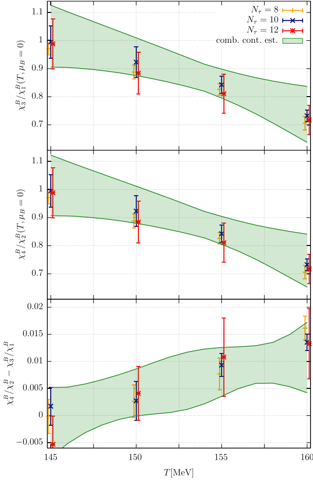
FIG. 3. Fluctuation-ratios \chi_3^B/\chi_1^B and \chi_4^B/\chi_2^B obtained from the fugacity expansion truncated at the B_{\max} = 2 level at \mu_B = 0 on our N_\tau = 8, 10 , and 12 lattices and our continuum estimates from these data. The points at finite lattice spacing include a systematic error coming from whether we used the 12- or the 16-parameter fit to determine the B_{\max} = 2 sectors. The continuum results include systematic errors from four fits, in addition to the 12- vs 16-parameter fits at fixed N_\tau and T . We also include a 5- vs 6-parameter combined T and N_\tau continuum fit.
