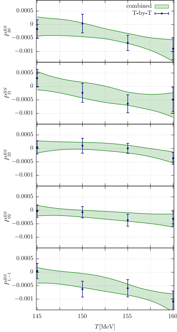
FIG. 2. Our continuum estimates of the beyond-ideal-HRG sector coefficients. We show the results both from our combined temperature and continuum fit (green bands) and of a T -by- T continuum limit extrapolation (blue points). Systematic errors are included, in the first case by varying B_{\max} = 2 vs 3 and b_2 = 0 or b_2 \neq 0 , and in the second case by varying B_{\max} = 2 vs 3.
