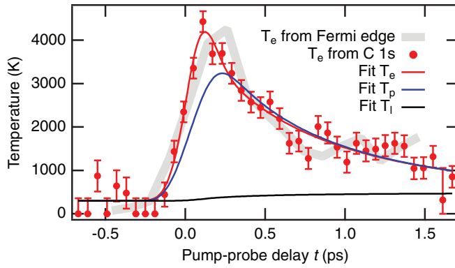
FIG. 2. Time-dependent electronic temperature extracted from the fit of the C 1s core level data in Fig. 1(a) (red markers). The red solid line is a fit to the electronic temperature T_e using a three-temperature model, giving the temperatures of the strongly coupled phonons T_p (blue line) and the remaining lattice T_l (black line). The gray, thick line corresponds to the T_e obtained from an analysis of the Fermi-Dirac distribution in the valence band.
