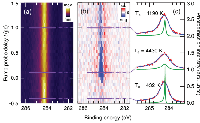
FIG. 1. (a) C 1s photoemission intensity as a function of pump-probe delay and binding energy. (b) Same as in (a) but with the average spectrum before excitation subtracted. Red and blue indicate an increase and decrease in electron counts, respectively. (c) Selected spectra (cuts at specific time delays) along with best fit to the model described in the text (blue line). The temperature-dependent asymmetry kernel for each fit is shown in green. The electronic temperatures resulting from the fit are noted close to the spectra.
