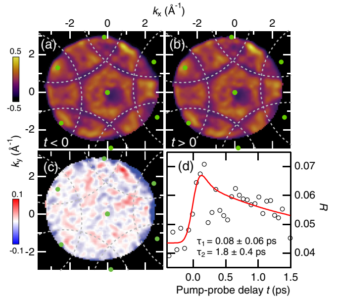
FIG. 3. (a) C 1s photoemission intensity integrated over negative pump-probe delay times, displayed as a modulation function in momentum space. The \Gamma points are shown in green. The dashed lines emphasize regions of low photoemission intensity (“dark lines”) arising from a combination of scattering by the graphene reciprocal lattice and reflection at the surface potential. (b) The same as in (a), but integrated over positive time delays. (c) Difference of the modulation functions in (a) and (b). (d) Comparison between the time-dependent modulation function and the equilibrium modulation function, quantified by R(t) . A fit to the data using a double decaying exponential convoluted with a Gaussian is shown in red.
