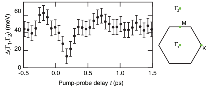
FIG. 4. Time-dependent C 1s bandwidth obtained from the energy difference between the C 1s peaks at the \Gamma_1 and \Gamma_2 points of the first and the neighboring Brillouin zone (see sketch on the right-hand side).
