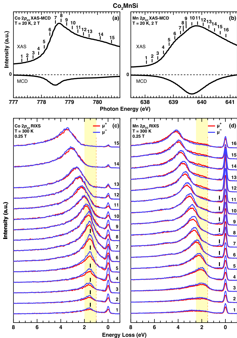
Figure 2. (a,b) XAS and XAS-MCD spectra of \text{Co}_2\text{MnSi} obtained at the Co and Mn 2p_{3/2} edges. (c,d) Photon energy dependence of the Co and Mn 2p_{3/2} RIXS spectra for \text{Co}_2\text{MnSi} obtained by \mu^+ and \mu^- configurations recorded at the excitation photon energies indicated by the numbers above the vertical bars on the XAS spectra. The hatched regions are guides to the eye for showing the evolution of the RIXS structures, and the vertical dashed lines indicate the threshold energies.
