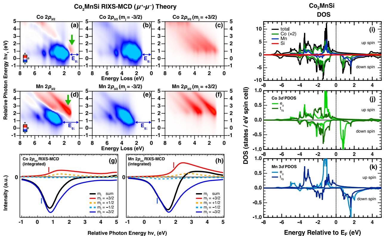
Figure 4. Theoretical RIXS-MCD spectra for \text{Co}_2\text{MnSi} at the \text{Co } 2p_{3/2} edge (a). The m_j = -3/2 and +3/2 components are shown in (b,c). Theoretical RIXS-MCD at the \text{Mn } 2p_{3/2} edge (d) and the m_j = \pm 3/2 components are shown in (e,f). The green arrows in (a,d) indicate the m_j = +3/2 components located in the down-spin gap ( E_{g\downarrow} ) of m_j = -3/2 components obtained in (b,e). The incoming photon energy dependence of the m_j resolved MCD intensity integrated over whole loss energies are also shown in (g,h) for Co and Mn edges, respectively. The vertical bars indicate the threshold energies of the m_j = \pm 3/2 components. (i) the theoretical prediction of the spin-dependent DOS and PDOS of Co, Mn, and Si. (j,k) the e_g and t_{2g} components of the PDOS of Co and Mn, respectively.
