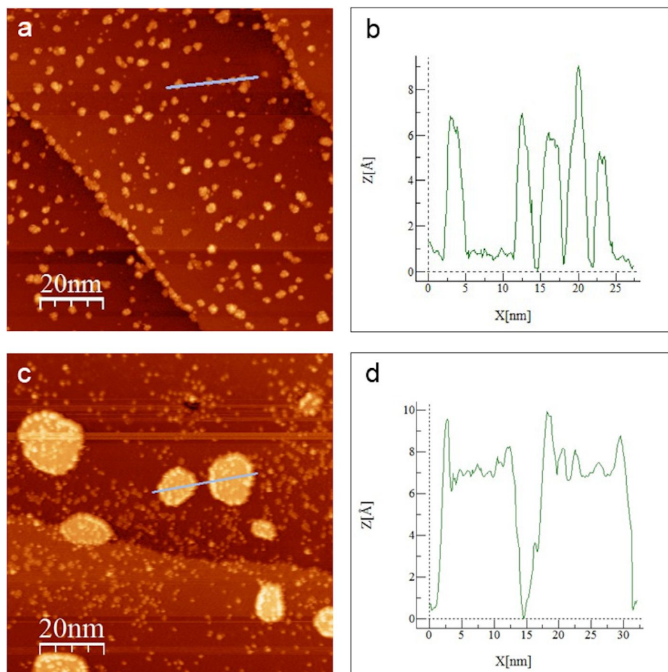
Figure 5: STM images of the initially \text{W}_3\text{O}_9 -covered w' - \text{TiO}_x phase grown on \text{Pt}_3\text{Ti}(111) after annealing the sample for 5 min. (a) Flashing the surface to 600 K leads to cluster agglomerations on the terraces and decoration of the step edges ( 98 \times 98 nm; U_B = 1.48 V; I_T = 75 pA). (b) The height profile along the line marked in (a). The cluster agglomerations have a typical thickness between 0.6 and 0.9 nm. (c) Flashing the surface to 900 K leads to the formation of larger \text{WO}_3 islands ( 98 \times 98 nm; U_B = 1.60 V; I_T = 75 pA). (d) The height profile along the line marked in (c). The islands have always a thickness of \approx 0.6 nm with residues of clusters on top.
