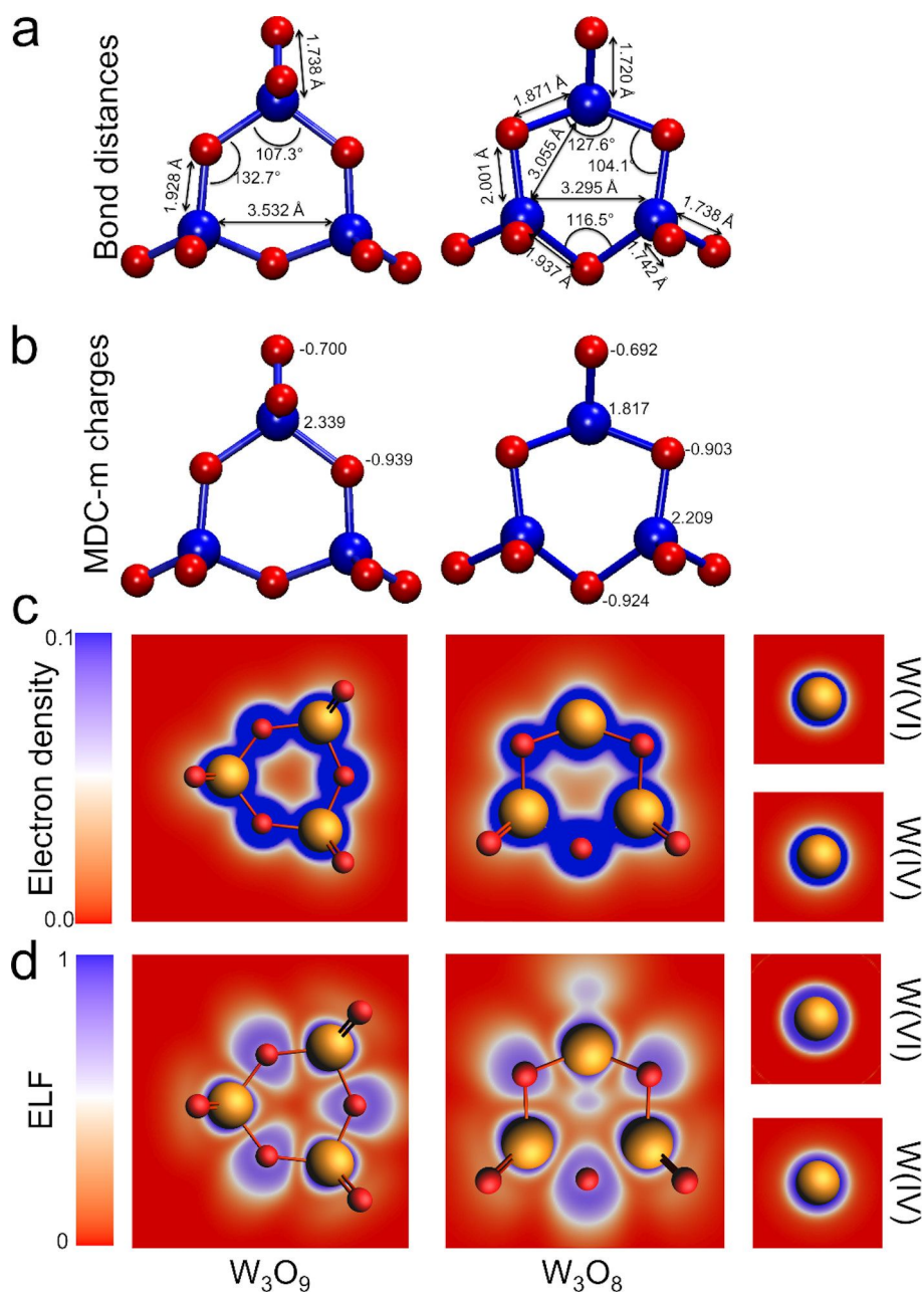
Figure 4: Structural and electronic properties of simulated W_3O_9 and W_3O_8 clusters. (a) Relaxed structures with the respective D_{3h} and C_s symmetries and the selected bond distances and bond angles. (b) Multipole-derived charges using monopoles (MDC-m) of all atoms, showing that two types of W atoms are present in the W_3O_8 cluster, corresponding to +VI and +IV oxidation states. (c) Total electron density (p) and (d) electron localization function (ELF). The latter two show differences in the electron density and localization not only for W atoms but also for O atoms within the hexagonal ring.
