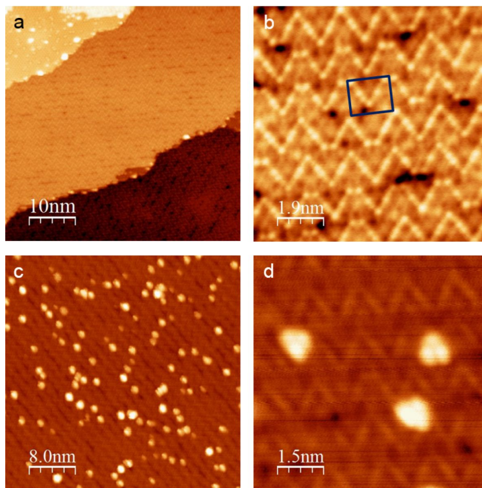
Figure 1: STM images of the z' -TiO x phase grown on Pt 3 Ti(111): (a) An overview image (50 × 50 nm; U_B = 1.57 V; I_T = 160 pA) of the clean oxide phase. In the upper left area, oxide-free patches of the metallic substrate can still be found. (b) An atomic resolution scan (9.4 × 9.4 nm; U_B = 1.22 V; I_T = 160 pA) of the z' -TiO x phase with a marked unit cell. The dark areas inside the trenches represent holes in the oxide film. (c) The z' -TiO x phase after deposition of W 3 O 9 (≈0.1 monolayer coverage; 40 × 40 nm; U_B = 1.00 V; I_T = 86 pA). The clusters are always aligned along the trenches. (d) A submolecular resolution scan (7.7 × 7.7 nm; U_B = 1.00 V; I_T = 86 pA) of individual W 3 O 9 clusters.
