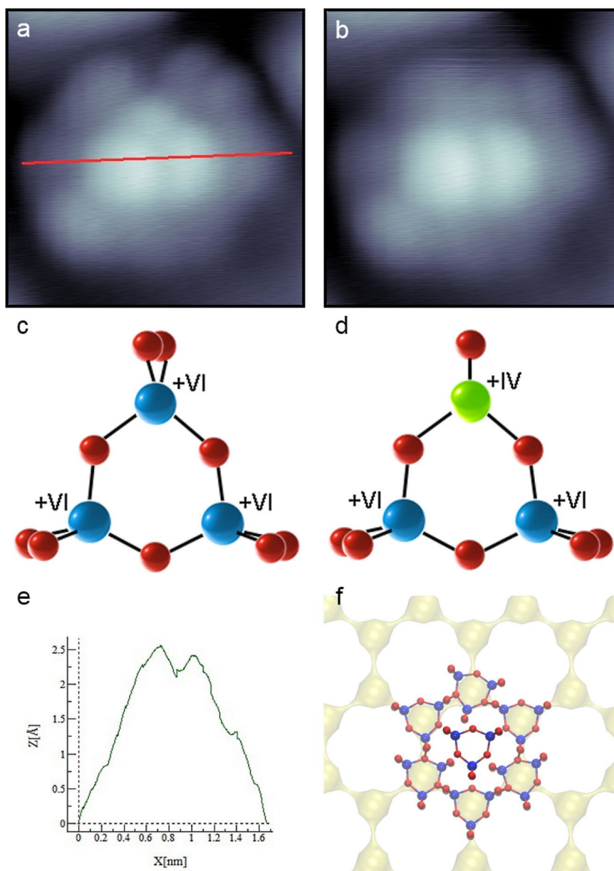
Figure 3: High-resolution STM images (both 1.8 \times 1.8 nm; U_B = 0.50 V; I_T = 62 pA) of a supramolecular assembly of W_3O_9 molecules on the w' - TiO_x phase grown on Pt_3Ti(111) before (a) and after (b) an intermediate scan with U_B = -1.00 V and I_T = 40 pA. By this procedure, the appearance from the top-laying molecule changed from a three-lobe to a two-lobe structure, indicating a partial reduction of one of the tungsten atoms resulting in W_3O_8 . Panels (c) and (d) illustrate the proposed structures before and after the procedure. The graph in (e) shows the corresponding height profile of the W_3O_9 stack in (a) marked by the red line. Panel (f) illustrates the proposed orientation on the w' - TiO_x phase grown on Pt_3Ti(111) .
