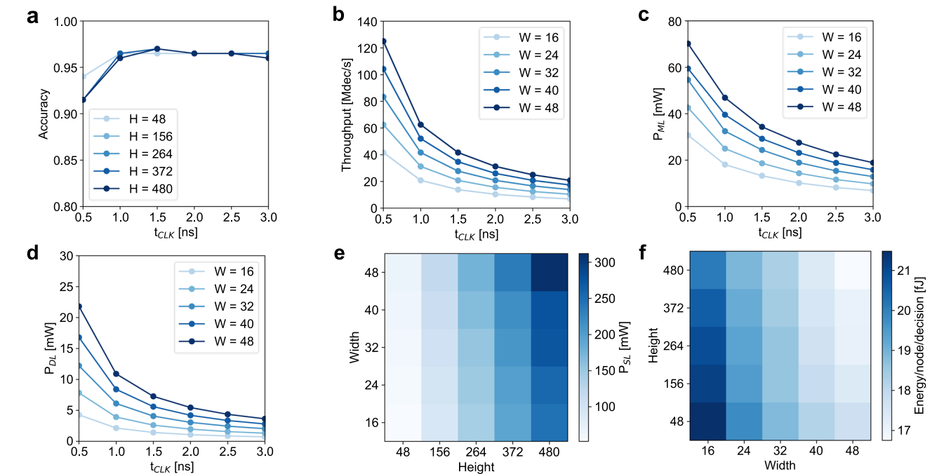
Fig. 5 Performance evaluation. a Classification accuracy as a function of t_{clk} for different tile height H at fixed tile width W = 16 . Accuracy does not depend on H as expected, until for nominal operational frequency namely for t_{clk} > 1 ns, below which mapping in the chosen conductance range is not possible. Throughput ( b ), ML dynamic power consumption ( c ) and DL dynamic power consumption ( d ) as a function of t_{clk} for different W at fixed H = 48 . e SL static power consumption as a function of H and w for t_{clk} = 1 ns. f Energy per DT node per decision as a function of H and w for t_{clk} = 1 ns.
