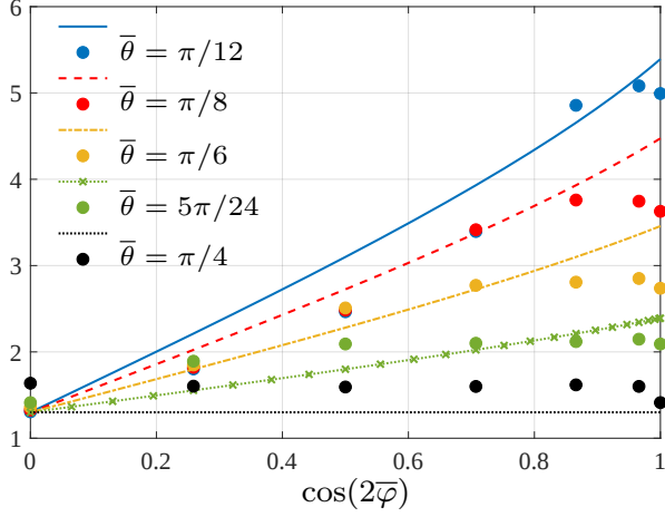
FIG. 4. Comparison between the theoretical bound a_1 Q_{\Psi} + a_2 (lines), with Q_{\Psi} \in [0, 1] , and -\log_2 \varepsilon_{\max} (dots) as a function of \cos(2\bar{\varphi}) and 5 different values of \cos(2\bar{\theta}) corresponding to \bar{\theta} = k\pi/24 with k = 2, \dots, 6 . Again the values of the model parameters a_1 and a_2 , here respectively equal to 7.5 and 1.3, are obtained by means of a single fitting procedure operating at once on all the 5 curves depicted in the figure.
