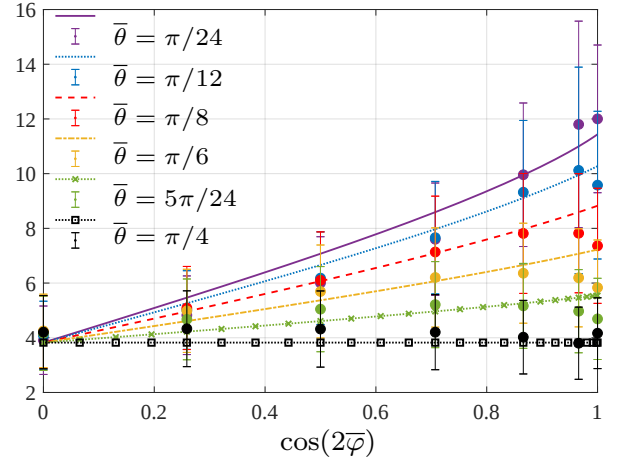
FIG. 2. Qubit-qubit control scheme. Comparison between the theoretical bound a_1 Q_{\bar{\Psi}} + a_2 (lines), with Q_{\bar{\Psi}} \in [0, 1] , and -\log_2 \langle \varepsilon \rangle (dots) as a function of \cos(2\bar{\varphi}) and 6 different values of \cos(2\bar{\theta}) , with \bar{\varphi}, \bar{\theta} = k\pi/24 and k = 1, \dots, 6 . The error bars denote the standard deviation of the negative logarithm of the control error, while the values of the model parameters a_1 and a_2 , respectively equal to 11.8 and 3.8, are obtained by means of a single fitting procedure operating at once on all the 6 curves depicted in the figure. The control error is obtained by solving numerically the proposed fully-quantum control problem for 1000 different target states \hat{\rho}_S and then making the average over all the sampled target states. It is worth noting that for \cos(2\bar{\varphi}) \rightarrow 1 with \bar{\theta} \neq 0 the numerical average control error slightly increases (i.e. -\log_2 \langle \varepsilon \rangle slightly decreases when \cos(2\bar{\varphi}) is very close to 1) – see Appendix for more details.
