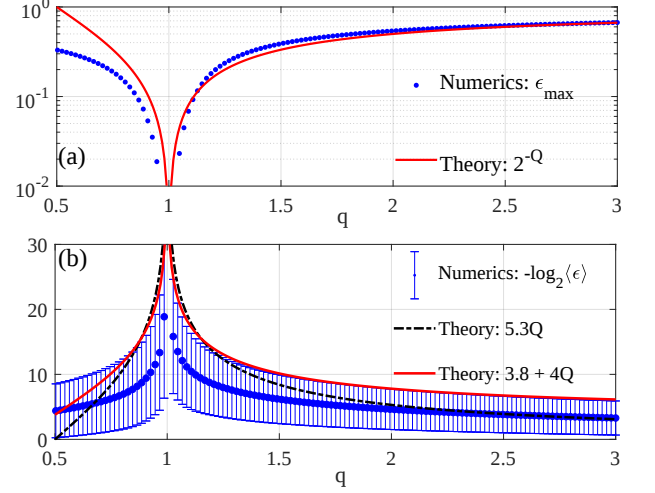
FIG. 3. Fully-quantum control associated to a one-mode Bosonic Gaussian channel. (a) Comparison between the maximum values \varepsilon_{\max} of the control error \varepsilon (blue dots), obtained by numerically solving the control problem for 1000 different target covariance matrices, and 2^{-Q_{\Psi}} \equiv q/|1-q| (red solid line) for q \in [0.5, 3] by using a logarithmic scale for the y -axis (for the sake of brevity, Q_{\Psi} is denoted as Q in the legends of the two panels of the figure). Note that, although the comparison in (a) is more qualitative (indeed, a_1 = a_2 = 1 ), the link between \varepsilon_{\max} and Q_{\Psi} can be clearly assessed. (b) Linear-scale comparison between the numerical values of -\log_2(\langle \varepsilon \rangle) and the empirical model a_1 Q_{\Psi} + a_2 as a function of q \in [0.5, 3] . The blue dots denote the average values \langle \varepsilon \rangle of the control error over the sampled target covariance matrices, while the corresponding standard deviations are represented by blue error bars. Here, the values of a_1 and a_2 are respectively provided by the sets (5.3, 0) (black dotted line) and (4, 3.8) (red solid line). Also notice that Q_{\Psi} \in [0, \infty) : Q_{\Psi} = 0 for q = 1/2 and q \rightarrow \infty , while Q_{\Psi} \rightarrow \infty when q = 1 .
