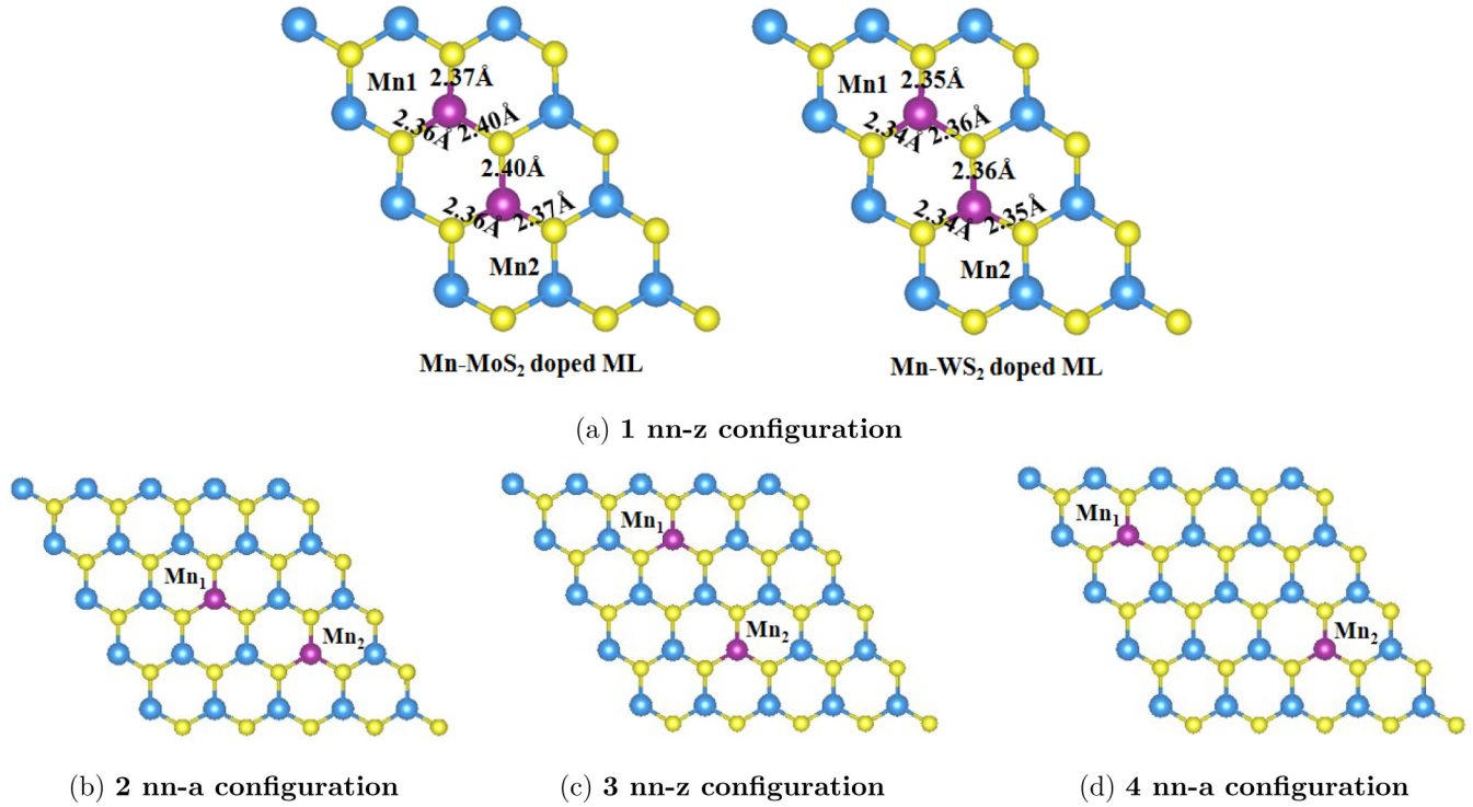
FIG. 9. Top view of the atomic structures corresponding to 8%-Mn-doped 5 \times 5 \times 1 \text{MoS}_2 supercells. Four doping configurations have been considered: (a) 1 nn configuration, (b) 2 nn configuration, (c) 3 nn configuration, and (d) 4 nn configuration. The yellow atoms are the sulfur (S), the blue atoms are the molybdenum (Mo), and the manganese atom is denoted by purple color.
