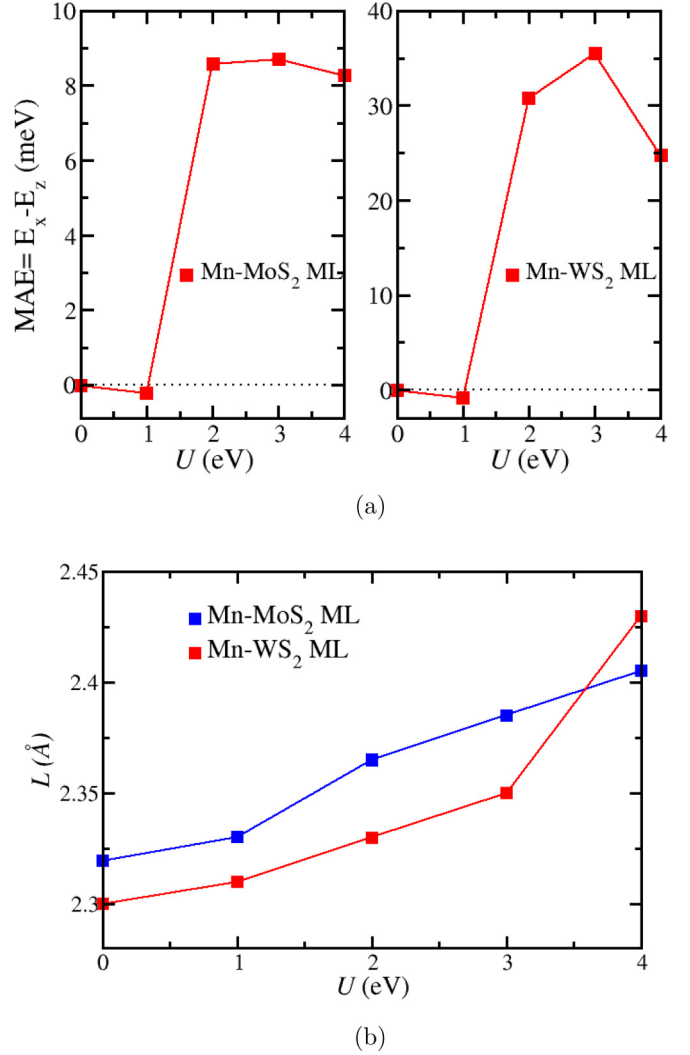
FIG. 2. (a) The magnetic anisotropy energy (MAE) of Mn- MS_2 -doped MLs as a function of the Hubbard parameter U . (b) The length L of the bonds formed between Mn dopant and the first nearest-neighbor S host atoms as a function of U .
