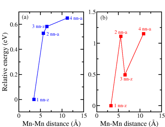
FIG. 10. Mn-Mn distance dependence of relative energy of Mn pair doped (a) \text{MoS}_2 ML and (b) \text{WS}_2 ML.
