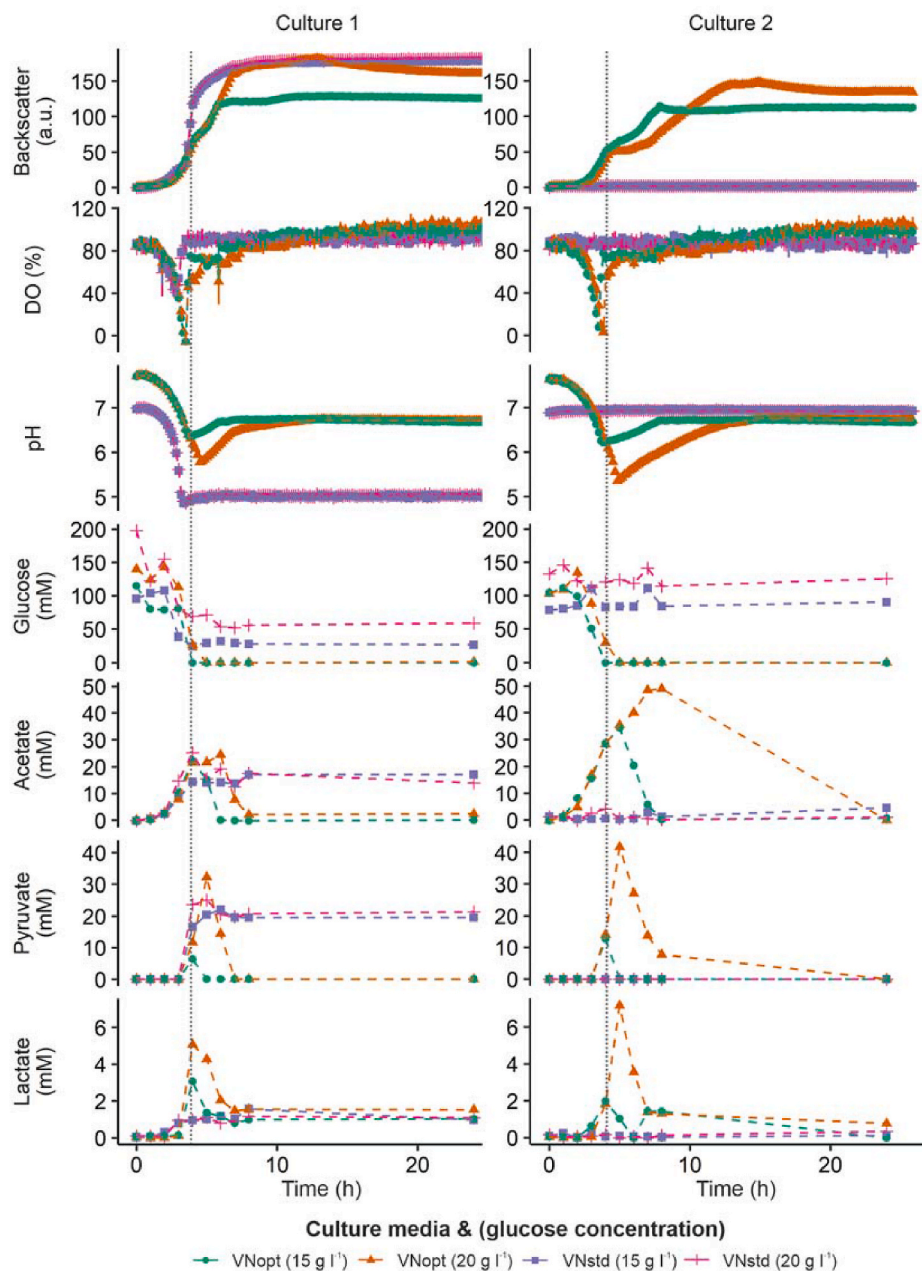
Fig. 1. Optimization of a V. natriegens growth medium suitable for repetitive-batch cultivation. V. natriegens growth in standard VN (VNstd) with 15 g l -1 glucose or 20 g l -1 glucose, and optimized VN (VNopt) with 15 g l -1 glucose or 20 g l -1 glucose. For two repetitive cultivations, backscatter (indicates biomass), dissolved oxygen and pH were measured online ( n = 3 , mean and standard deviation are shown), and samples were taken for measurement of glucose, acetate, pyruvate and lactate concentrations ( n = 1 representative culture). Vertical grey lines indicate end of first exponential phase of culture in VNopt with 15 g l -1 glucose.
