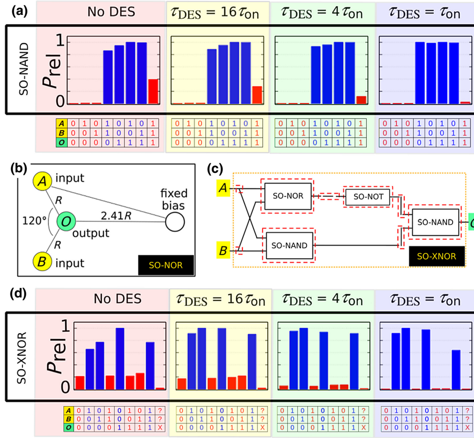
FIG. 5. The performance of the SO-NAND gate and the SO-XNOR gate with dynamic error suppression (DES). (a) The state probability distributions of a SO-NAND gate for different DES check times, \tau_{\text{DES}} . The relative probability P_{\text{rel}} is obtained by dividing the probabilities of all of the possible states by the probability of the most likely logical state. (b) The SO-NOR gate is realized with the same geometry as the balanced SO-NAND gate, the only difference being the reversed magnetization of the fixed-bias island. (c) A schematic representation of a SO-XNOR gate. (d) The state probability distributions of a SO-XNOR gate for different \tau_{\text{DES}} . The symbol “?” means that input islands A or input islands B are not logically consistent. All logically inconsistent states are aggregated into the X state (X stands for 0 or 1).
