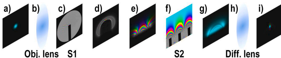
Fig. 1. Schematic diagram showing the evolution of an electron beam through an orbital angular momentum sorter. See text for details.
