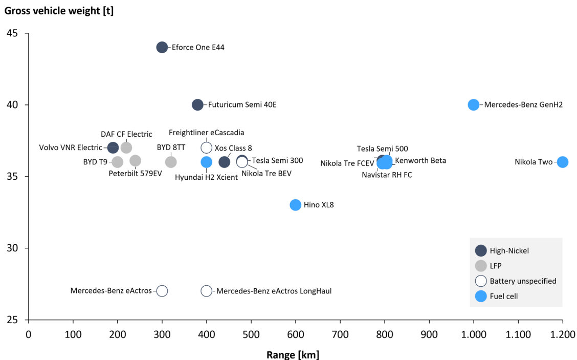
Fig. 1. Summary of BETs and FCETs currently on the market or in commercialization based on vehicle range, maximal gross vehicle weight and truck propulsion technology.
