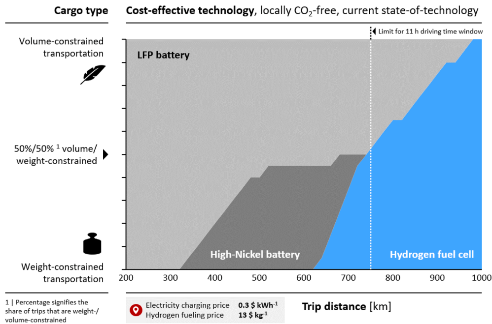
Fig. 3. Cost-effective technology choice for locally CO 2 -free trucks at current technology level under current U.S. regulation and energy prices.
