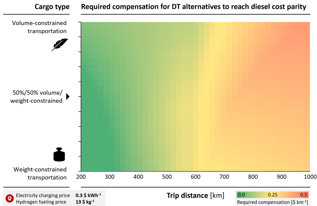
Fig. 5. Required compensation for cost parity with diesel trucks, depending on trip distance and cargo type.
