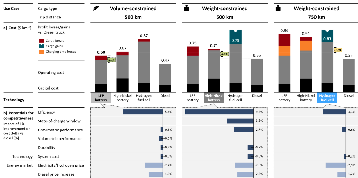
Fig. 6. Cost comparison for different truck use cases and potentials to increase competitiveness versus DT.
