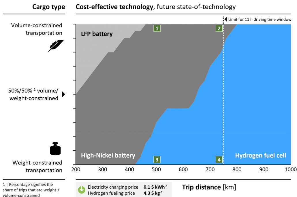
Fig. 7. Cost-effective technology choice at potential future technology level under current U.S. regulation & optimistic energy prices.
