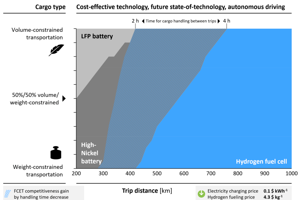
Fig. 9. Impact of autonomous driving on cost-effective technology choice depending on different cargo handling times that can be used for BET charging.
