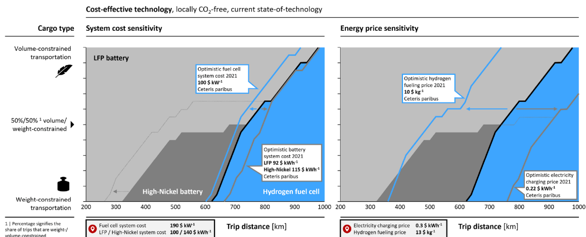
Fig. 4. The effect of different system and energy cost assumptions on the cost-effectiveness of technologies at current technology level.
