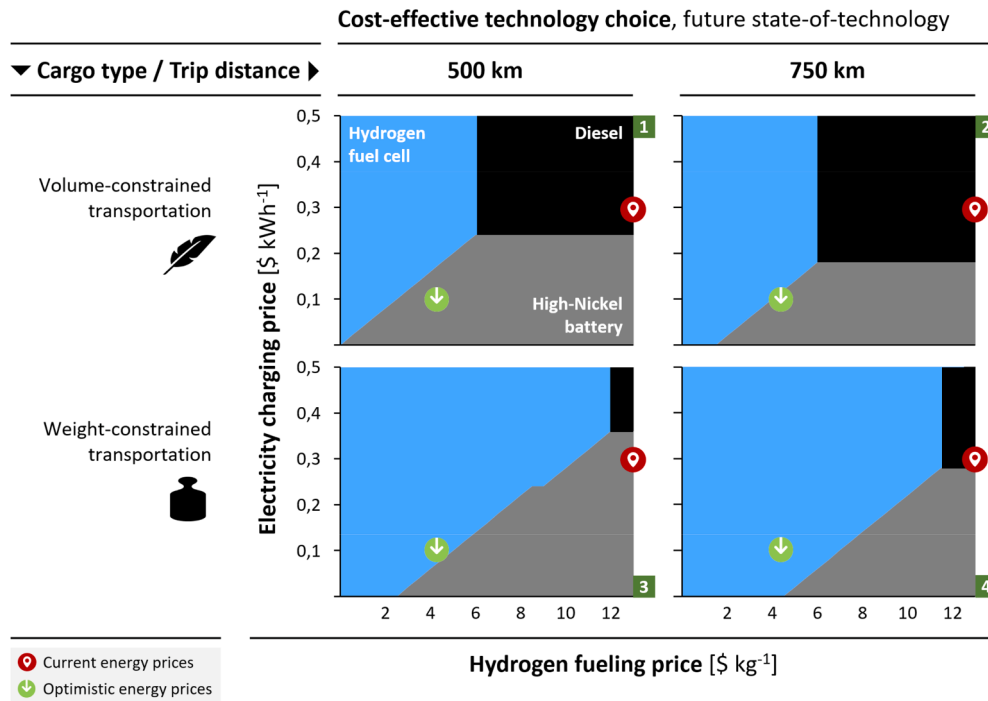
Fig. 8. Impact of hydrogen fueling price and electricity charging price developments on cost-effective technology choice in different use cases.
