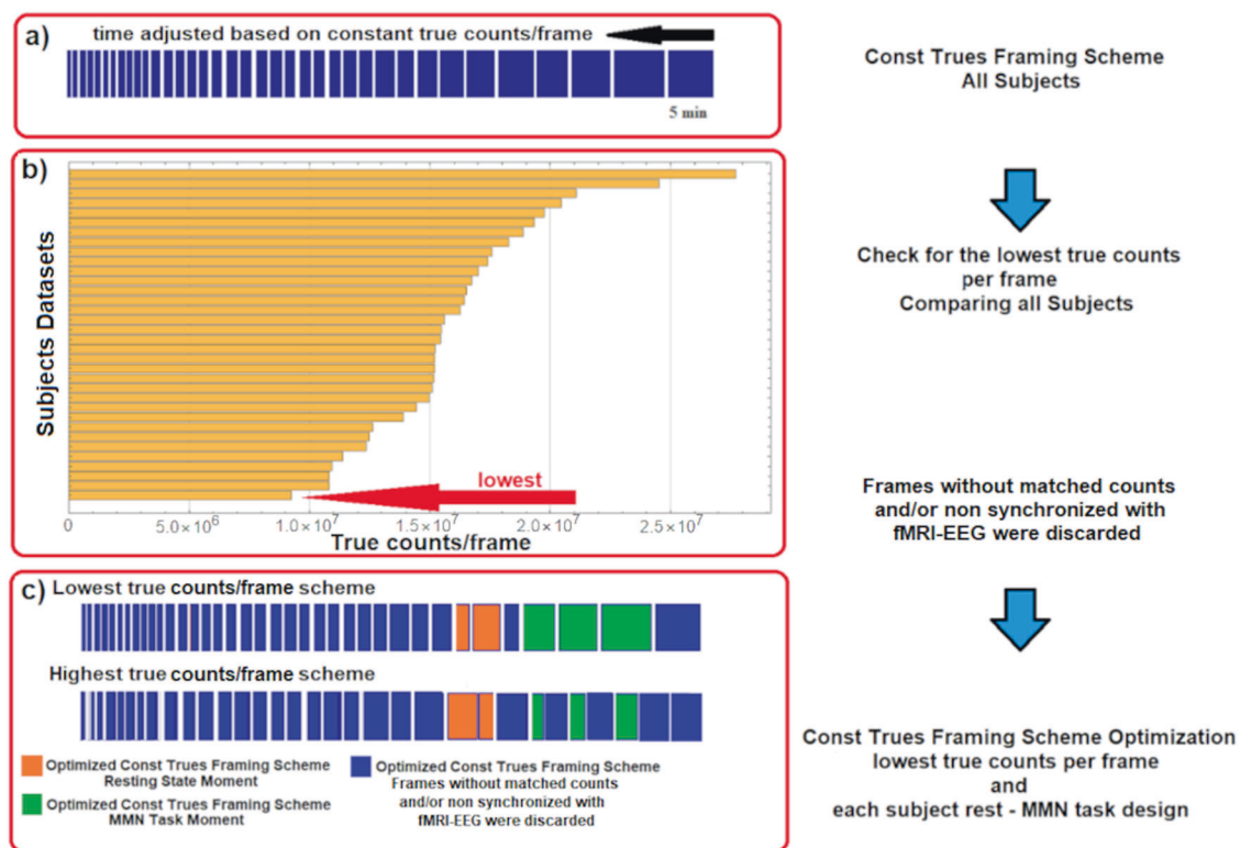
Fig. 2 PET-matched framing scheme applied in this [^{11}\text{C}]\text{ABP688} study. a General frame scheme with variable time-frame lengths, enabling constant true counts/frame. b Comparison of all subjects to find the lowest-average true counts per frame. c Two individual Const Trues framing schemes showing the optimization to match the lowest-average true counts per frame between subjects and synchronized with the different acquisition moments: pretask resting state and the MMN task.
