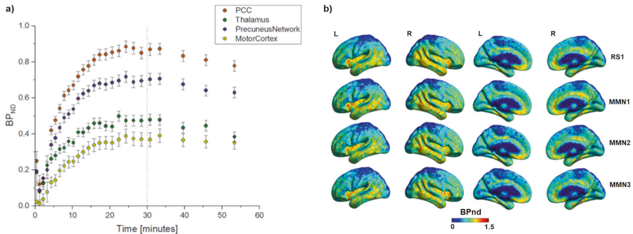
Fig. 4 Task effect results shown by the regional and voxel-wise cerebral uptake of [ ^{11} C]ABP688 expressed as distribution volume referenced to cerebellum grey matter, BP. a BP_{ND} curves for the anatomical and functional brain regions analyzed. Significant effects can be seen in the healthy group. The red line marks the start point of tracer equilibrium phase. After 30 min, the first two time points represent RS 1 and the remaining three time points represent the MMN task moments (MMN 1 , MMN 2 , and MMN 3 ). b BP_{ND} parametric images for the group average per acquisition moment.
