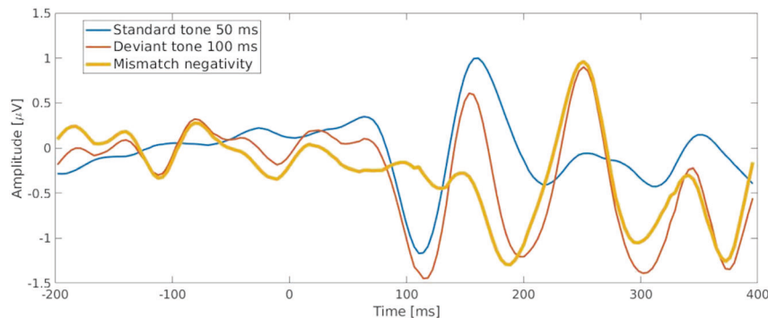
Fig. 5 Auditory-evoked potential (AEP) of standard and deviant tones during the MMN paradigm calculated by averaging F 3 , F z , F 4 , C 3 , C z , and C 4 channels. Additionally, the mismatch-negativity difference wave obtained by subtracting the standard from deviant event-related potentials is also shown.
