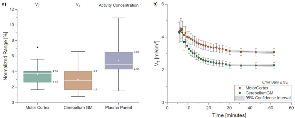
Fig. 3 Equilibrium quality evaluation/inspection represented by regional cerebral uptake of [ ^{11}\text{C} ]ABP688 expressed as distribution volume referenced to plasma parent, V_T . a Normalized-range variations of the V_T values in the plateau range (30–60 min) for the motor cortex and cerebellum GM-control regions during the equilibrium phase. The plasma parent compound normalized activity-concentration range for evaluating the equilibrium quality is also shown. b Average V_T curves and the linear regression applied to the data plateau range (30–60 min) for the slope analysis. SE = standard error of the mean ( \text{mean}/\sqrt{n} ), where n = sample size.
