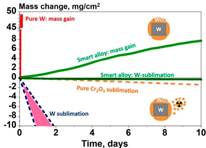
Figure 2. The evolution of mass change, due to oxidation and sublimation depending on exposure time of the SMART alloys, pure tungsten and chromia ( \text{Cr}_2\text{O}_3 ). Processes of oxidation leading to the mass gain and sublimation leading to the mass loss are shown with schemes in the upper and lower parts of the figure, correspondingly.
