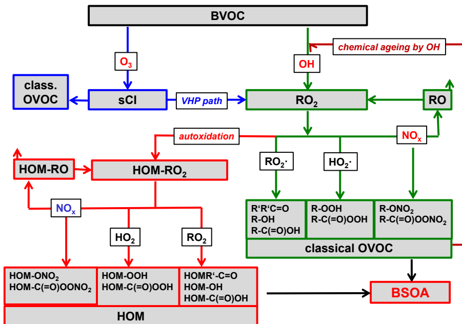
Figure 1.1: Reaction pathways of BVOC oxidation by O_3 and OH radicals. Blue boxes show a simplified ozonolysis path and green boxes show classical photochemical reactions that result in various closed-shell products (classical OVOC). These products can condense on particles if their volatility is sufficiently low. Red boxes represent a new class of highly oxygenated organic molecules which are connected to classical photochemistry by the process called autoxidation involving highly oxygenated peroxy radicals (HOM- RO_2 ).
