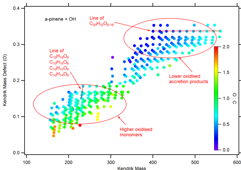
Figure 2.15: An example of the Kendrick mass defect plot for \alpha -pinene photooxidation. The x-axis shows Kendrick mass and the y-axis shows Kendrick mass defect. Reagent ions were not considered in the calculation. The O-atom was used as a unit. Color code represents the O:C ratio of the compounds.
