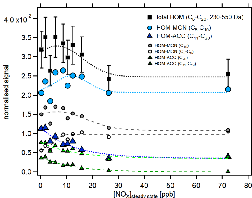
Figure 4.4: The normalised signals of total HOM, monomers, accretion products and HOM that resulted from fragmentation processes, in the mass range of 230 Da to 550 Da as a function of NO x . Black squares show total HOM, blue circles and triangles represent HOM monomers (HOM-MON) and accretion products (HOM-ACC). HOM-MON did not change much as NO x concentration increased while HOM-ACC decreased by \frac{2}{3} at the highest NO x level (72 ppb) compared to reference NO x level (0.3 ppb). Smaller grey and white circles show the signal of C 10 monomers and C 5-9 monomers, respectively. Smaller light green and dark green triangles represent C 20 accretion products and C 11-19 accretion products. From the gain of C 5-9 monomers and the relative gain of C 11-19 accretion products, the increasing importance of fragmentation is deduced. Dashed and dotted lines serve only to guide the eye and have no further meaning. All data presented here were corrected for turnover and particle surface as described in Chapter 2.4.1
