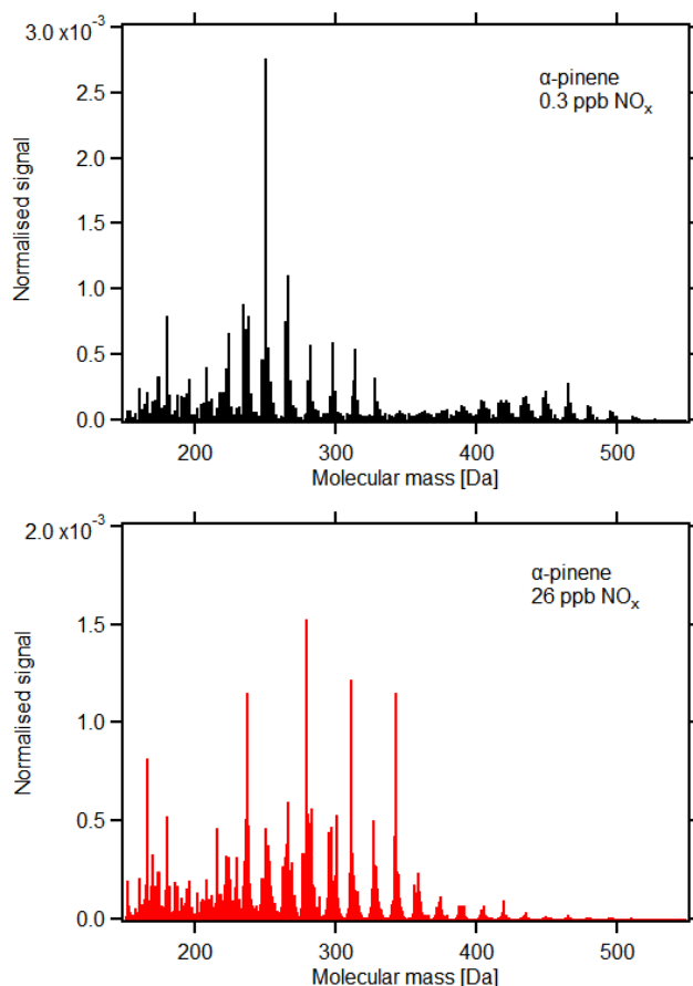
Figure 4.7: Mass spectra observed in the oxidation of \alpha -pinene by OH at 0.3 ppb background NO x (upper black mass spectrum) and in the presence of 26 ppb NO x (lower red mass spectrum) under steady state conditions. The x-axis represents the molecular mass without the mass of the reagent ion NO 3 - and the y-axis shows normalised signal.
