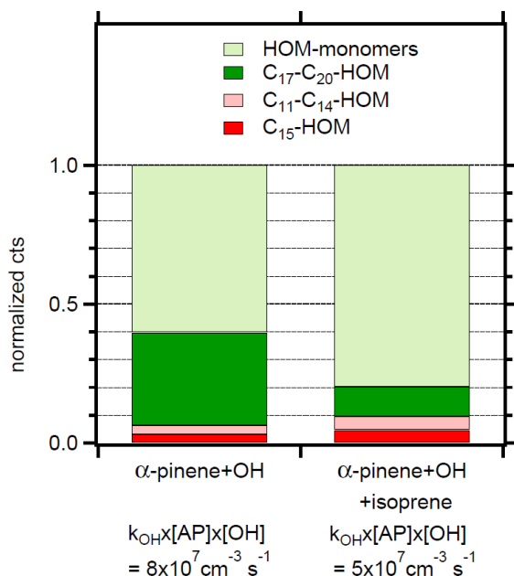
Figure 3.26: Relative contributions of HOM monomers and accretion products with a different numbers of carbon in the molecule. Left bar shows the fraction of HOM monomers (light green), C 17-20 accretion products (dark green) which were derived from \alpha -pinene OH oxidation. Pink bar showed the fraction of C 11-14 which were most likely coming from the reaction of mixed peroxy radicals from \alpha -pinene and isoprene OH oxidation. Right bar shows the fraction of each group in isoprene addition experiment. The data of two experiments were normalised by 344 cts (left) and 151 cts (right) respectively. Adapted from McFiggans et al. , 2019.
