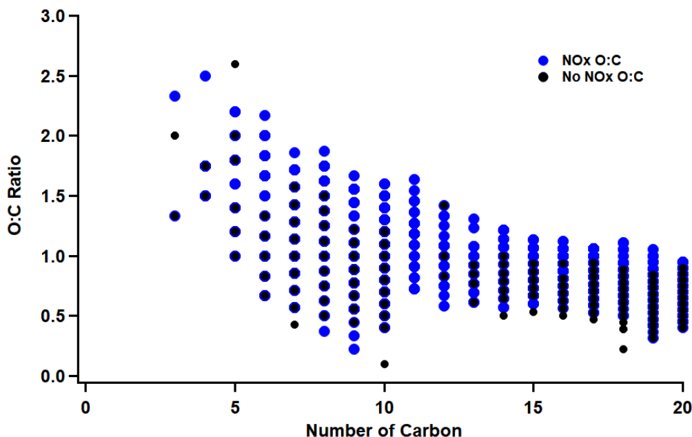
Figure 4.8: O:C ratio of \alpha -pinene photooxidation products in the presence of background level NO x (0.3 ppb, black circles) and 8.7 ppb of NO x (blue circles) as a function of the number of carbon atoms. Each point represents detected molecules during the experiment and identified with high resolution analysis. The x-axis shows the number of carbon in the compounds and the y-axis shows the ratio between oxygen and carbon in the molecule.
