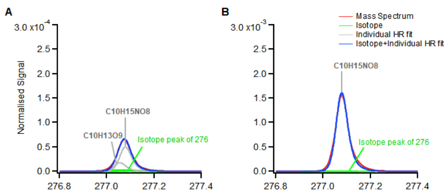
Figure 2.12: Comparison of peak identification at molecular mass 277 Da in the \text{NO}_x experiment. The concentration of \text{NO}_x was 0.3 ppb (A) and 8.7 ppb (B). The red line shows the measured mass spectrum and the grey lines show each individual peak. The green line shows the isotope signal from previous integer mass and the blue line is the sum of the signal from individual peaks and isotope signal (Grey and Green). Signals were normalised to the sum of all ions.
