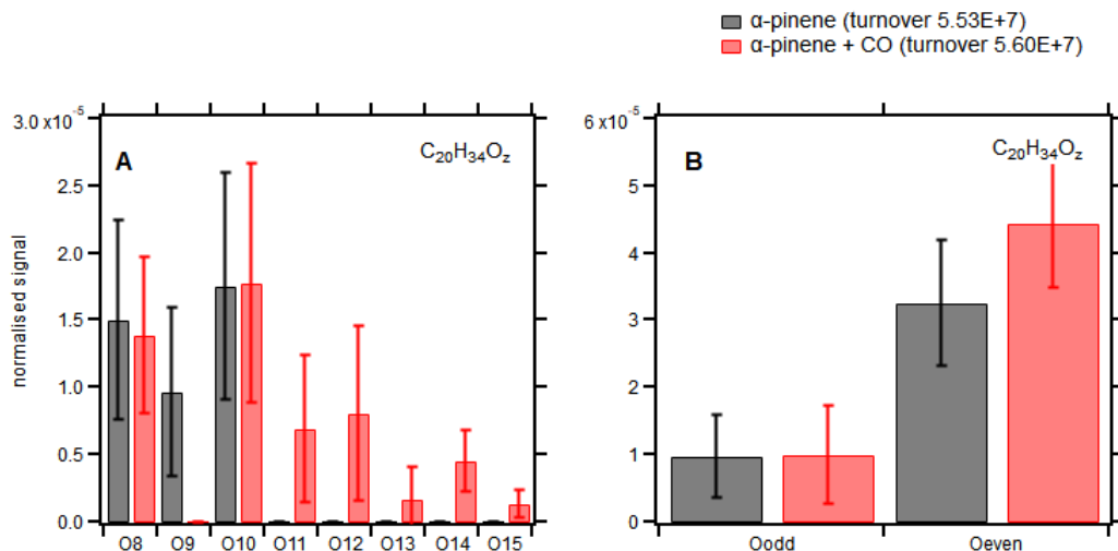
Figure 3.22: Bar graph of \text{C}_{20}\text{H}_{34}\text{O}_z accretion product family members of two experiments. Panel A shows the normalised signal of each member in the two experiments. The x-axis is the number of O-atoms in the family members' molecular formula. On the right side, sum of family members which have an odd or even number of oxygen in the molecule is shown for two experiments.
