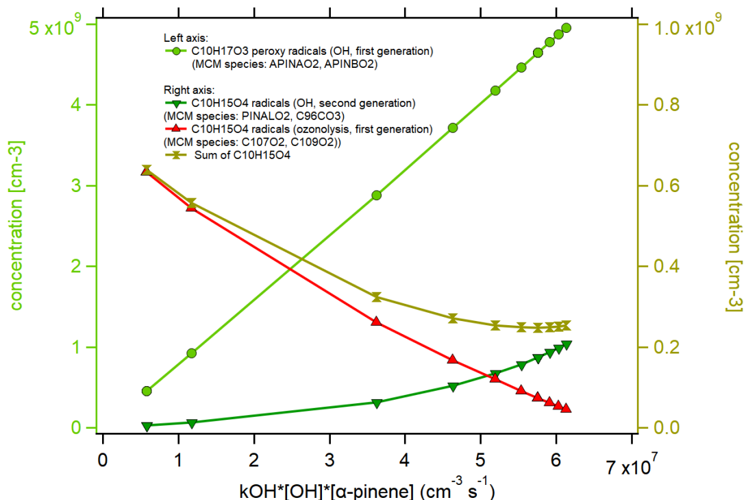
Figure 3.8: The modeled concentration of C_{10}H_{17}O_3 (light green circles), the primary peroxy radical of \alpha -pinene and OH, and C_{10}H_{15}O_4 , the peroxy radical from ozonolysis (red triangles) and secondary OH attack of oxidation product like pinonaldehyde (green upside down triangle) and sum of C_{10}H_{15}O_4 (olive green hourglass) as a function of turnover. The left y-axis represents the concentration of C_{10}H_{17}O_3 peroxy radicals and the right y-axis represents C_{10}H_{15}O_4 peroxy radicals from different sources.
