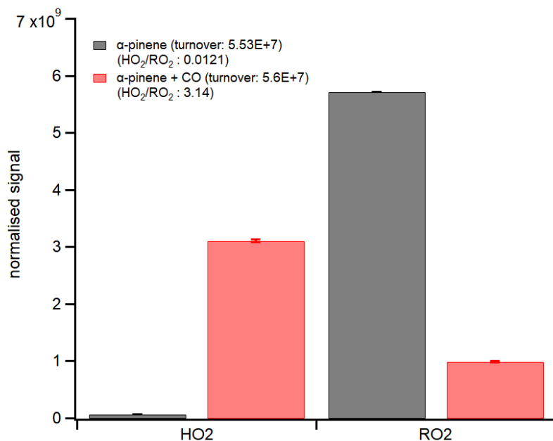
Figure 3.15: Bar graph of modeled HO 2 and RO 2 concentration of two experiments. The HO 2 /RO 2 ratio was 0.012 for the reference experiment and 3.1 for the CO experiment. (Model data were provided by Silvia Proff)
