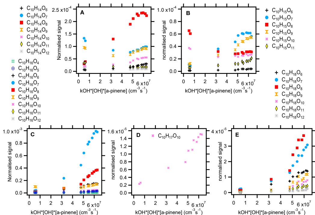
Figure 3.14: The normalised signal of the C_{10} family members versus turnover. Panel A shows C_{10}H_{14}O_x family members and panel B shows members of C_{10}H_{15}O_x peroxy radical family. Panel C shows C_{10}H_{16}O_x family members which was attributed to the mixture of alcohol, hydroperoxide and carbonyl from different peroxy radicals. Panel D shows C_{10}H_{17}O_x peroxy radical family members and panel E shows C_{10}H_{18}O_x family members which is the mixture of the alcohol and the hydroperoxide. Mind that the scale of the y-axes are not same.
