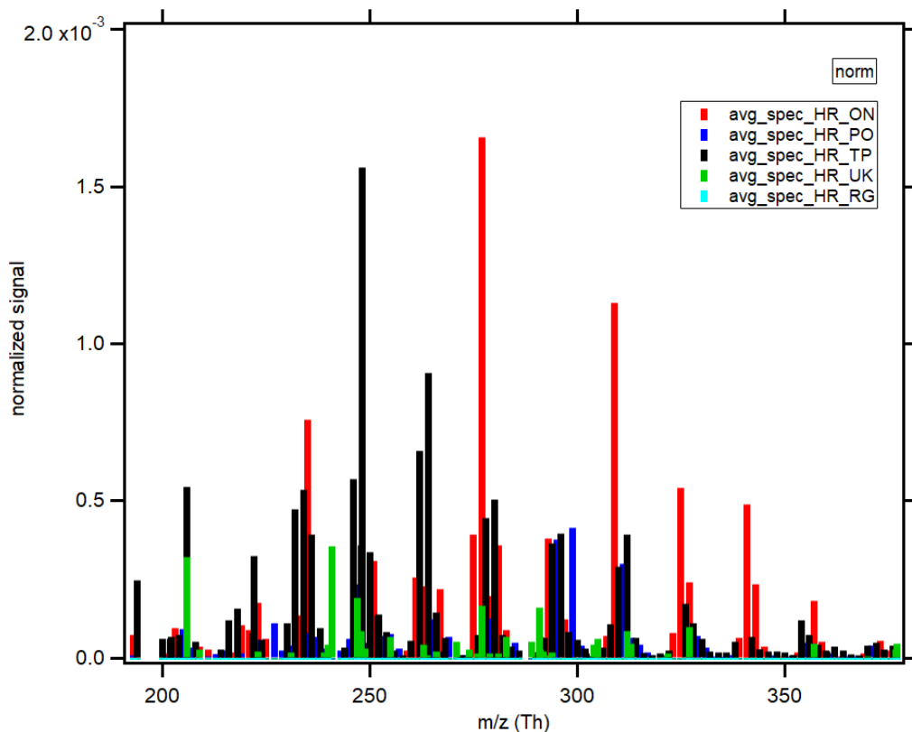
Figure B.2: The example of high resolution stick mass spectrum obtained by CIMS analyzer program. The x-axis shows mass per charge ratio and y-axis shows normalised signals. Peaks are colour coded according to their class. Red( avg_spec_HR_ON ) represents organic nitrates and blue( avg_spec_HR_PO ) represents peroxy radicals. Black( avg_spec_HR_TP ) represents permutation products i.e., HOM-PP. Green( avg_spec_HR_UK ) represents unknown peaks and light blue( avg_spec_HR_RG ) represents reagent ion.
