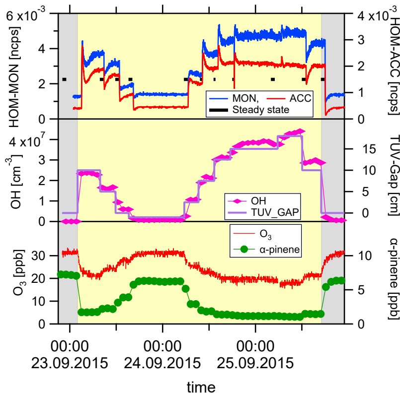
Figure 2.2: Time series of the \alpha -pinene OH oxidation experiment with varying j(\text{O}^1\text{D}) . The yellow shaded area represents the duration when UVC light was switched on for the production of OH radicals and the grey shaded area shows when UVC light was off. At the lowest graph, the measured concentration of \alpha -pinene (green circles) and \text{O}_3 (red line) concentration are shown. As UVC light is on, the concentration of \alpha -pinene and \text{O}_3 decreased because of the reaction with OH and being photolysed respectively. In the middle graph, the OH concentration (pink rhombus) and TUV gap (violet line) are shown. TUV gap means the gap between lamp shielding glasses and the higher TUV gap means the higher photolysis rate. On the top graph, the normalised signal of HOM (monomer (blue line) and accretion products (red line)) and the steady-state interval (black line) are shown. HOM concentration increased and decreased with varying OH concentrations.
