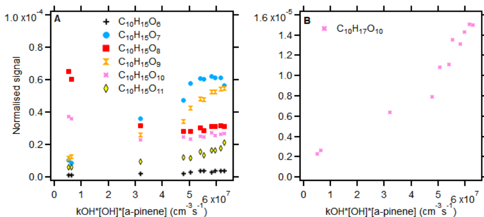
Figure 3.12: The normalised signal of family members of C_{10}H_{15}O_z (panel A) and C_{10}H_{17}O_z (panel B) as function of turnover.
