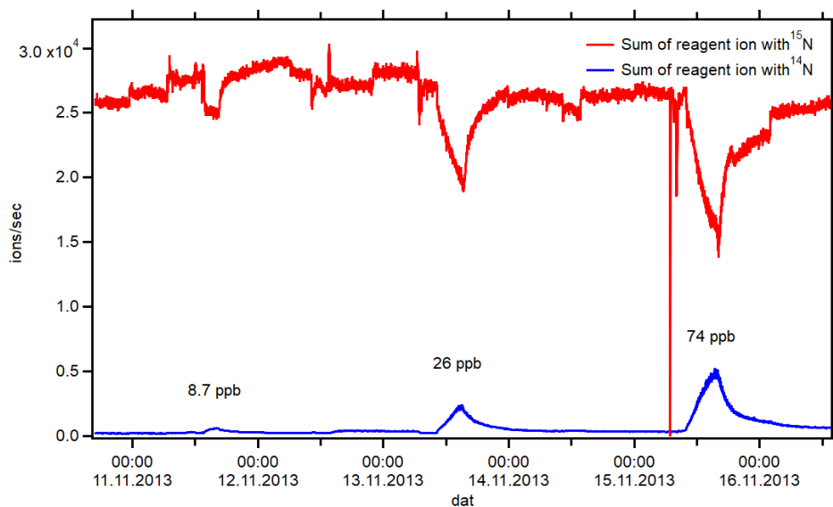
Figure 2.8: Time series of the summed up signal of ^{14}\text{NO}_3^- (blue), ^{15}\text{NO}_3^- (red), and their clusters in three different NOx experiments. The concentration of NOx was 8.7, 26 and 72 ppb, respectively. The percentage of ^{14}\text{N} nitrate reagent ions increased from 1.9 %, 10 % and 25 %.
