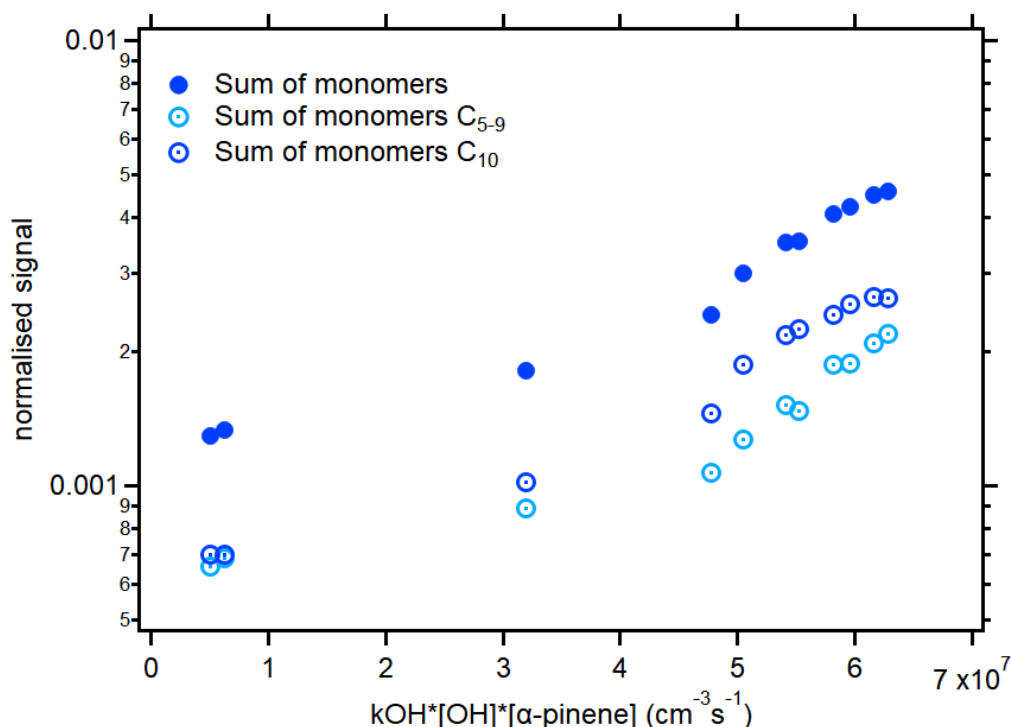
Figure 3.5: The sum of monomers vs turnover. Signals were normalised to total ion counts. Blue filled circles represent the sum of all monomers. Light blue open circles show the sum signal of fragmented monomers that have 5-9 carbon atoms. Blue open circles show monomers with 10 carbon atoms.
