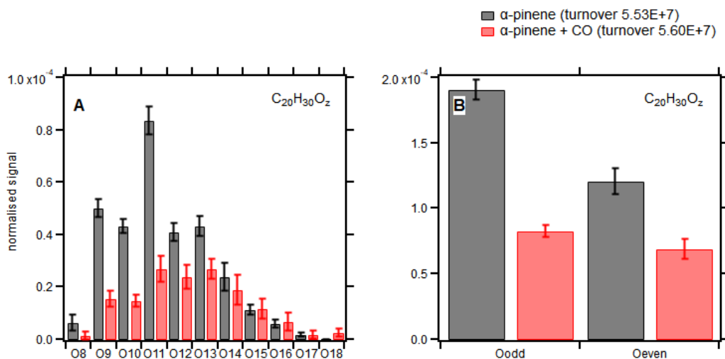
Figure 3.20: Bar graph of C 20 H 30 O z accretion product family members of two experiments. On the left side, panel A shows the normalised signal of each member in the two experiments is shown. The x-axis is the number of O-atoms in the family members' molecular formula. On the right side, sum of family members which have an odd or even number of oxygen in the molecule is shown for two experiments.
