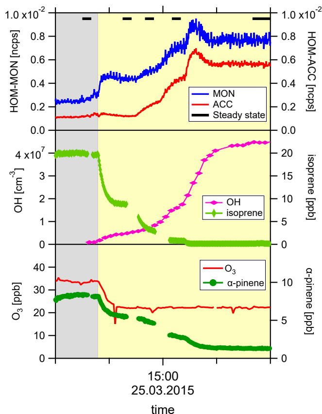
Figure 2.4: Time series of the \alpha -pinene OH oxidation experiment in the presence of isoprene. The yellow shaded area represents the duration when UVC light was switched on for the production of OH radicals and the grey shaded area shows when UVC light was off. At the lowest graph, the measured concentration of \alpha -pinene (green circles) and O_3 (red line) concentration are shown. As UVC light is on, the concentration of O_3 decreased because it was photolysed. In the middle graph, the OH (pink rhombus) and isoprene (light green diamonds) concentrations are shown. Isoprene concentration decreased dramatically because of the reaction with OH (OH scavenging effect of isoprene). As isoprene concentration decreased, OH concentration increased. On the top graph, normalised signal of HOM (monomer (blue line) and accretion products (red line)) and the steady-state interval (black line) are shown.
