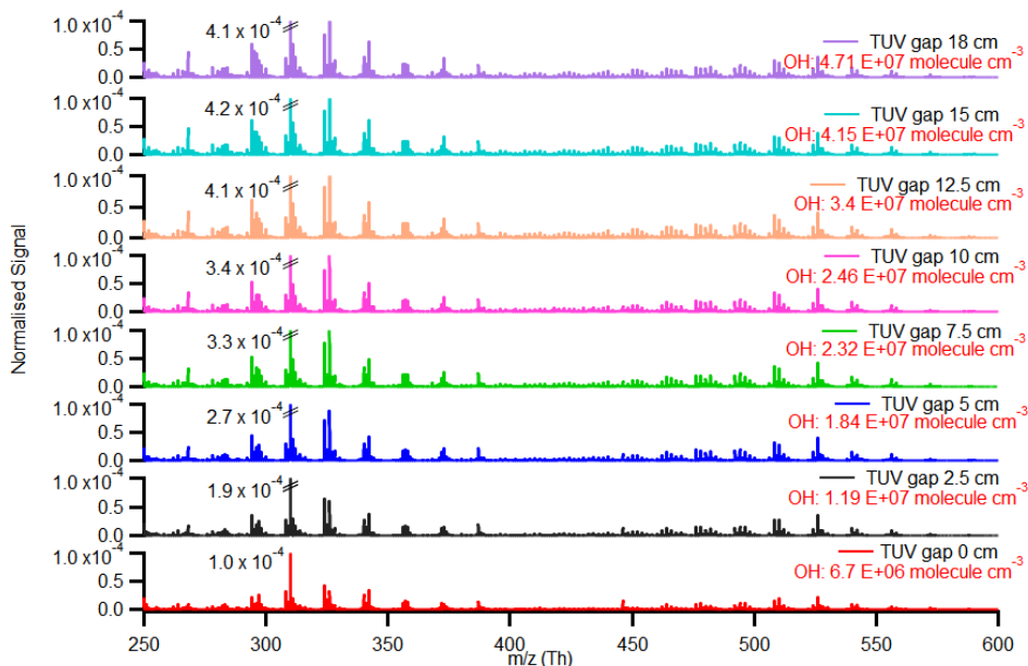
Figure 3.3: Mass spectra observed at different OH concentrations in "j(O 1 D)" experiment. The mass spectra was averaged over 30-60 minutes for steady state periods. The y-axis shows signal normalised to the total ion signal and the x-axis shows mass per charge ratio, including the reagent ion. On the right upper corner of each mass spectrum, TUV gap and OH radical concentration during steady state are given. Note that highest peak at 310 Th is cut off. The normalised signal of \text{C}_{10}\text{H}_{16}\text{O}_7 is written next to the peak.
