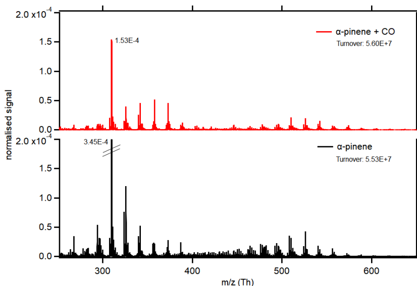
Figure 3.16: Mass spectra obtained for experiments with (red) and without CO (black) at steady state conditions and at similar turnover. Lower black mass spectrum was taken at a turnover of 5.53 \times 10^7 \text{ cm}^{-3}\text{s}^{-1} (reference mass spectrum). Upper red mass spectrum shows the situation of an experiment with 3 ppm of CO with turnover 5.60 \times 10^7 \text{ cm}^{-3}\text{s}^{-1} . The x-axis shows the mass per charge ratio. Compounds were detected as nitrate clusters. The y-axis shows the signal normalised to the total ion count. Because of the high signal at 310 Th in the reference mass spectra (normalised signal 3.45 \times 10^{-4} \text{ ncps} ), not the entire peak is shown in the mass spectrum for better comparison.
