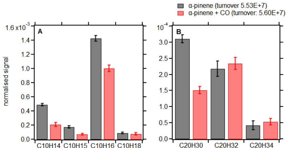
Figure 3.18: Bar graph of C 10 monomer families and C 20 accretion product families of two experiments are shown here. C 10 H 17 O z family and C 20 H 28 O z family did not shown here because they were not detected in CO experiment.
