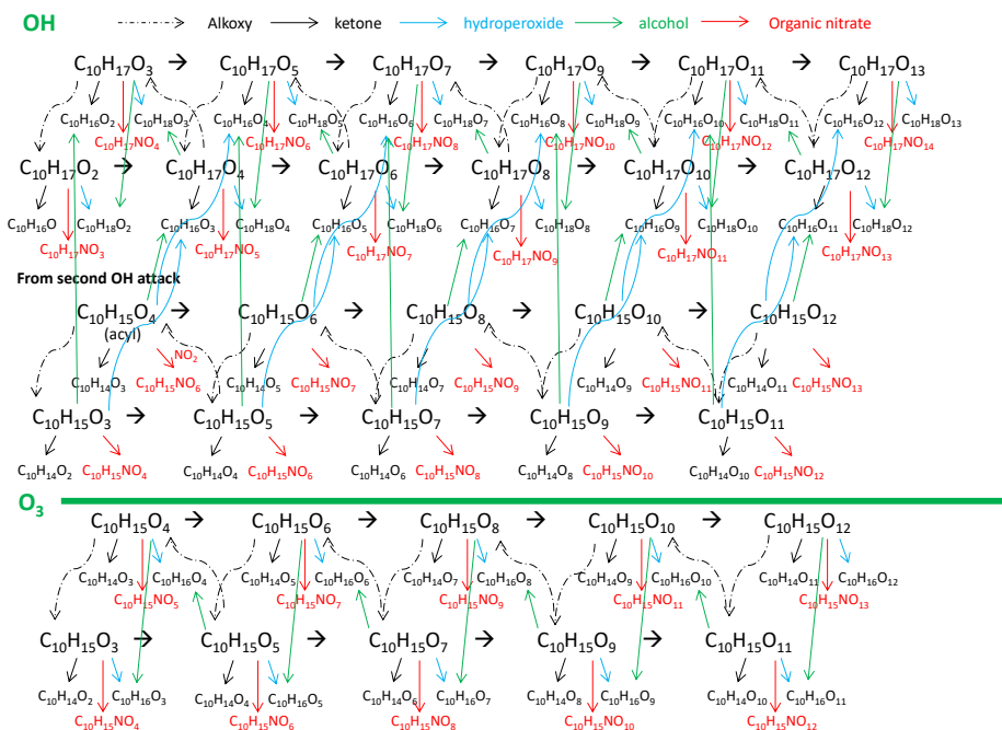
Figure 2.13: The map of the \alpha -pinene oxidation by the OH radical and O 3 . The upper part shows the oxidation of \alpha -pinene by the OH radical and the lower part shows the ozonolysis. Peroxy radicals, reaction pathways, and resulting products are shown. The C 10 H 15 O 4 peroxy radical in the beginning of the ozonolysis is formed via VHP. Autooxidation goes from the left to the right and increases the oxygen number by two. Dashed lined arrow indicates the alkoxy radical involving path. The black arrow pathways produce carbonyl termination products, while blue arrows pathways produce hydroperoxides. The green and red arrows pathway produce alcohols and organic nitrates, respectively. In this way, the potential origin of an observed compound can be tracked and possible information on the formation mechanism can be achieved.
