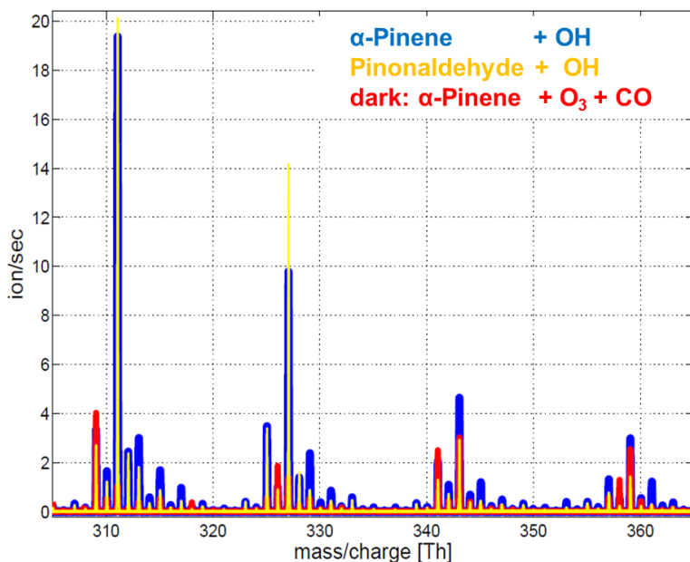
Figure 3.11: Overlapped mass spectrum of \alpha -pinene ozonolysis(red), \alpha -pinene OH oxidation(blue) and pinonaldehyde OH oxidation (yellow). The x-axis shows mass per charge ratio and the y-axis shows non-normalised signal. Pinonaldehyde mass spectrum was scaled to match the \alpha -pinene peak at 310 Th. Compound's mass/charge is shown with a cluster with NO_3^- ion. Data from Iida Pullinen.
