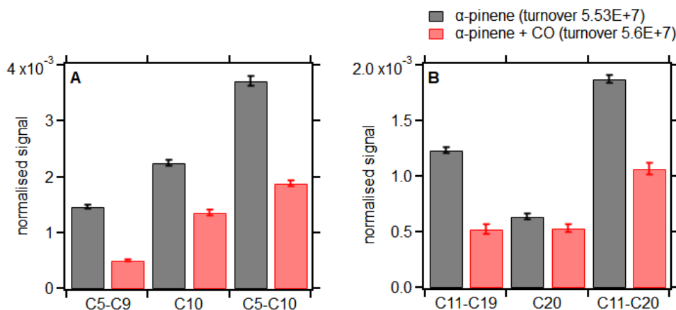
Figure 3.17: Bar graph of monomer and accretion products of two experiments are shown here. On the left side, panel A shows the comparison of monomers. C 5-9 shows the fragmented monomers and C 5-10 shows the sum of monomers. On the right side, panel B shows the comparison of accretion products. C 11-19 shows the smaller accretion products and C 11-20 shows the sum of all accretion products.
