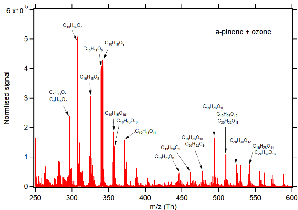
Figure 3.1: Typical mass spectrum of \alpha -pinene ozonolysis. The x-axis shows mass to charge ratio (m/z) and the y-axis shows the signal normalised to the total ion signal. The m/z shown is including the nitrate ion ( NO_3^- ). Compounds with relatively high signal are shown.
