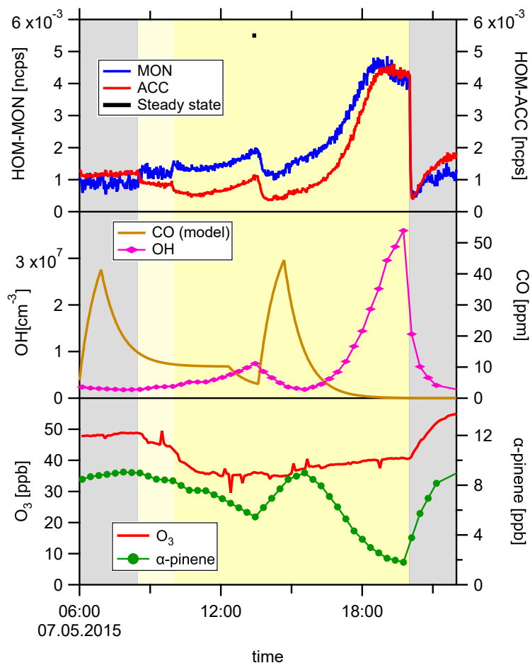
Figure 2.3: Time series of the \alpha -pinene OH oxidation experiment in the presence of CO. The yellow shaded area represents the duration when UVC light was switched on for the production of OH radicals and the grey shaded area shows when UVC light was off. At the lowest graph, the measured concentration of \alpha -pinene (green circles) and O_3 (red line) concentration are shown. As UVC light is on, the concentration of O_3 decreased because O_3 was photolysed. \alpha -pinene concentration did not decrease as dramatic as in the OH varying experiment because of the scavenging effect of CO on OH radical (pink rhombus in the middle graph). In the middle graph, CO (orange line) concentrations are shown as well. The concentration of CO is taken from the model calculation. In the presence of high CO concentration, OH was scavenged. However, OH radical concentration increased when CO was flushed out. On the top graph, the normalised signal of HOM (monomer (blue line) and accretion products (red line)) and the steady-state interval (black line) are shown. Changes in CO and OH radical concentration resulted in the changes in normalised HOM concentrations.
