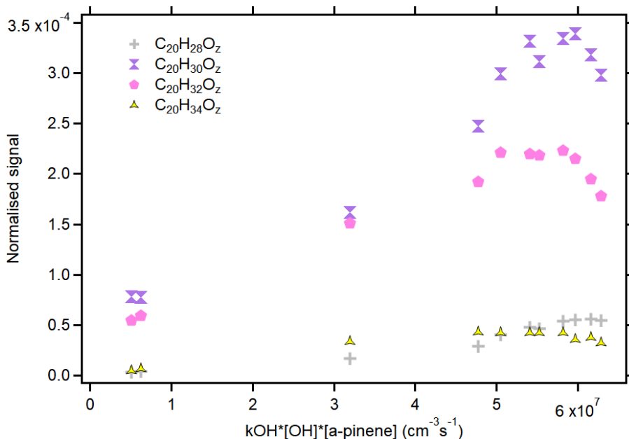
Figure 3.10: Signal of each \text{C}_{20} family normalised to total ion counts are plotted as a function of turnover. The grey crosses and the lilac hourglasses represents \text{C}_{20}\text{H}_{28}\text{O}_z and \text{C}_{20}\text{H}_{30}\text{O}_z family respectively. The pink pentagons and yellow triangular symbols shows normalised signal of \text{C}_{20}\text{H}_{32}\text{O}_z and \text{C}_{20}\text{H}_{34}\text{O}_z family.
