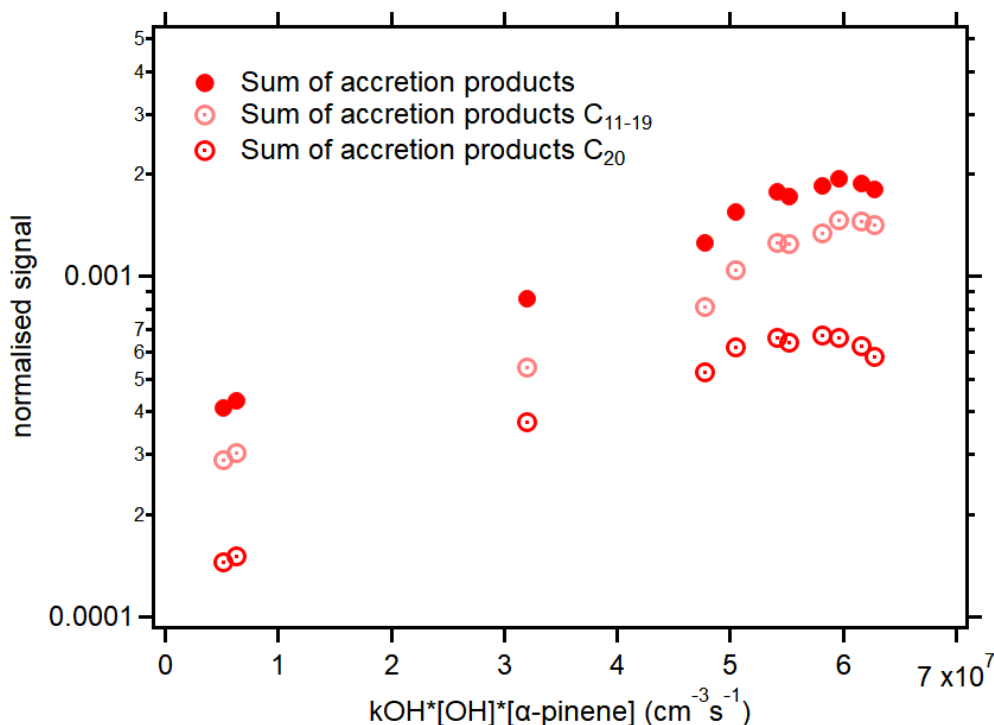
Figure 3.6: The sum of the signal of accretion products normalised to total ion counts vs turnover. Red filled circles represent the sum of all accretion products. Pink open circles show sum signal of accretion products with less than 20 carbons in the molecule ( C_{11-19} ). Red open circles show accretion products that had 20 carbons in the molecule.
