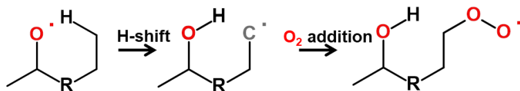
Figure 4.9: Reaction scheme of the alkoxy-peroxy pathway. Intramolecular hydrogen shift to the alkoxy site generates an alkyl radical site. It is followed by O 2 addition forming another peroxy radical, which could undergo autoxidation. By this way, alkoxy radicals do not fragment and maintain its carbon backbone with 10 C-atoms for \alpha -pinene.
