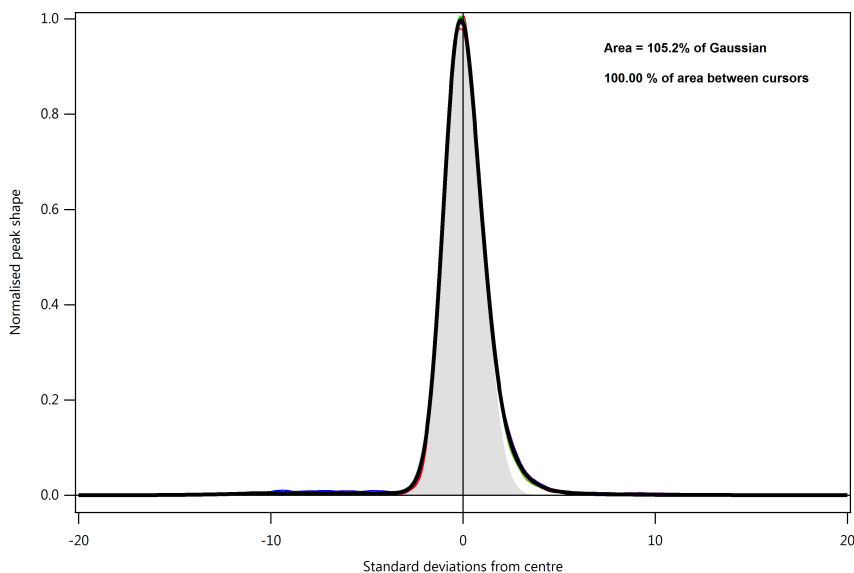
Figure 2.10: Peak shape determined for j(\text{O}^1\text{D}) experiment series. Selected peaks are normalised to 1. The thick coloured lines show selected peaks and the black thick line shows averaged peak shape of selected peaks. Grey area shows the Gaussian graph and the area of peak shape was calculated to be 105.2 % of Gaussian graph area.
