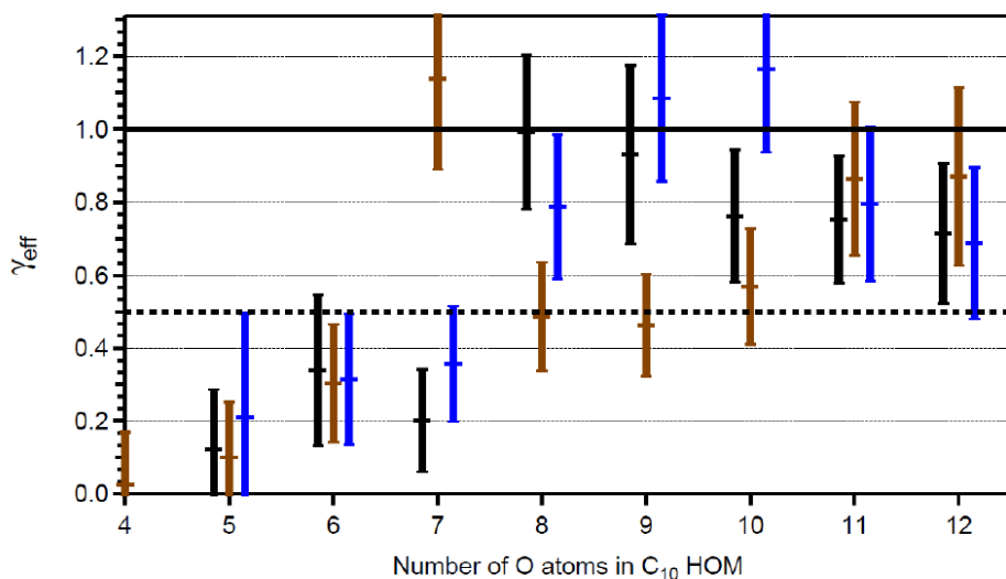
Figure 4.3: Effective uptake coefficients \gamma_{\text{eff}} for HOM-PP ( \text{C}_{10}\text{H}_{14}\text{O}_z (black bars), \text{C}_{10}\text{H}_{16}\text{O}_z (brown bars)) and HOM-ON ( \text{C}_{10}\text{H}_{15}\text{O}_z\text{NO}_2 , (blue bars)) are shown as a function of the number of O-atoms in the mother \text{C}_{10} peroxy radical. Because of the limited mass spectral resolution \text{C}_9 -HOM where one carbon and four hydrogens were replaced by one oxygen atom, e.g., \text{C}_{10}\text{H}_{16}\text{O}_8 and \text{C}_9\text{H}_{12}\text{O}_9 , are treated together. The black line indicate \gamma_{\text{eff}} = 1 and 0.5. The average Fuchs-Sutugin correction factor of 0.70 (for a median surface diameter d_p=175 nm) was applied to
