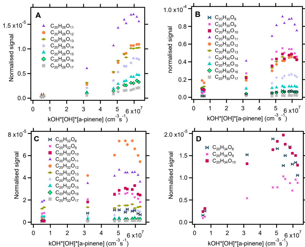
Figure 3.13: The normalised signal of C_{20} family versus turnover. Panel A and B show the signal of the C_{20}H_{28}O_z and the C_{20}H_{30}O_z family members. Panel C and D show the normalised signal of C_{20}H_{32}O_z and C_{20}H_{34}O_z family members respectively.
