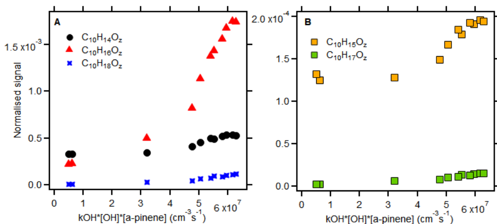
Figure 3.9: The signal of each C 10 family normalised to total ion counts are plotted as a function of turnover. In panel A, the black circles represent normalised signal of C 10 H 14 O z family and red triangles, blue stars show the normalised signal of C 10 H 16 O z , and C 10 H 18 O z respectively. Panel b shows the normalised signal of C 10 H 15 O z and C 10 H 17 O z family in orange and green squares.
