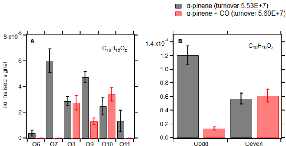
Figure 3.19: Bar graph of C_{10}H_{15}O_z accretion product family members of two experiments are shown here. On the left side, panel A shows the normalised signal of each member in the family members' molecular formula and the y-axis shows the normalised signal. On the right side, sum of family members which have an odd or even number of oxygen in the molecule was shown for two experiments.
