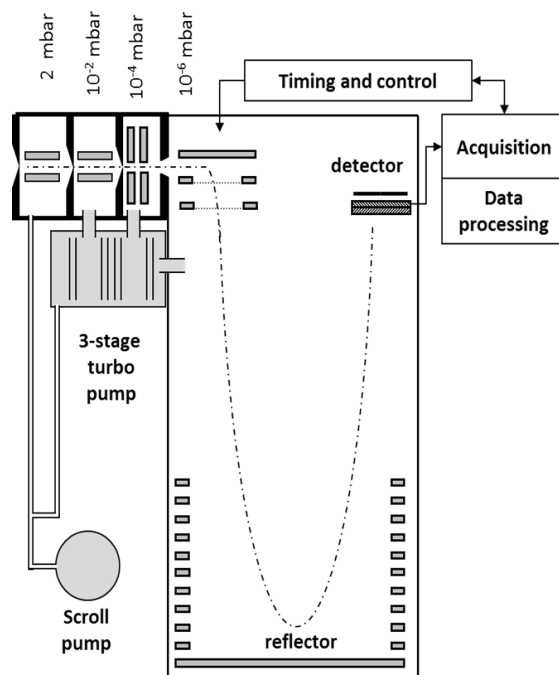
Figure 2.6: Schematics of the Atmospheric Pressure interface Time-of-Flight Mass Spectrometer. Sample air enters the first chamber through a critical orifice. Two quadrupoles and an electrical lens system guide the ions into the extraction region of the ToF-MS. The ToF path is folded by using a reflectron. Ions are detected by a multi-channel plate detector. A scroll pump and a three-stage turbo pump allow for a reduction of the pressure in four steps from atmospheric pressure to 10 -6 mbar.
