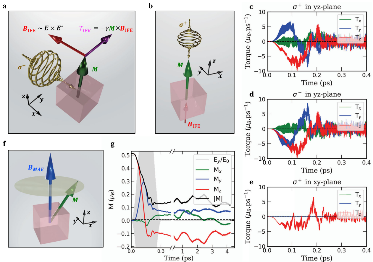
Fig. 4 Laser-induced ultrafast magnetic torques on bulk Ni. a, b Schematic illustrations representing a laser acting on an initial magnetization along the z -axis: (a) a right-circularly polarized pulse ( \sigma^+ ) in the yz -plane induces an inverse Faraday-like magnetic field ( \mathbf{B}_{\text{IFE}} ) opposite to the polarisation direction ( -x ), which at t = 0 exerts a torque ( \mathbf{T}_{\text{IFE}} ) on the magnetization ( \mathbf{M} ) along the +y direction; (b) a right-circularly polarized pulse in the xy -plane would generate an inverse Faraday-like magnetic field parallel to the magnetization ( +z ) and so at t = 0 it exerts no torque. c–e The components of the torques induced by a 300 fs wide pulse with the intensity of E_0 = 9.7 \times 10^9 \text{ V m}^{-1} that is c right-circularly polarized in the yz -plane, d left-circularly polarized ( \sigma^- ) in the yz -plane, and e right-circularly polarized in the xy -plane, respectively, computed according to Eq. (1). f The magnetization dynamics also have a contribution from the internal field due to the magnetic anisotropy (MAE) which induces precession. g The three components of magnetization ( \mathbf{M} ) along with the total length correspond to the case shown in (c) .
