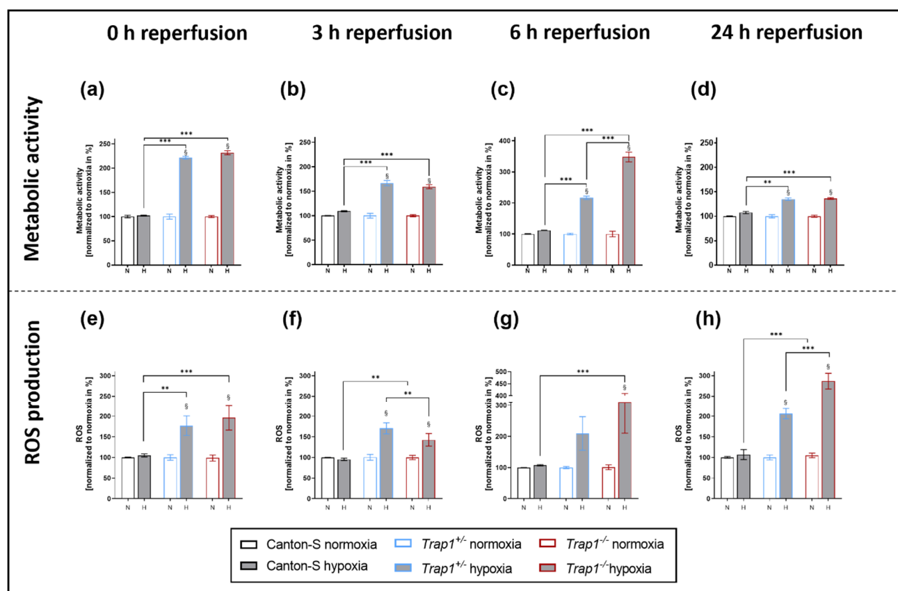
Figure 3. Metabolic activity and ROS production of Canton-S, Trap1 +/- and Trap1 -/- flies during a reperfusion period of 24 h. (a–d) Metabolic activity in the supernatant in fly head lysates after 3 h of hypoxia. ROS production in the fly head lysates is shown in (e–h). The graphs present the means \pm SEM of 4 independent experiments. Two-way ANOVA followed by Tukey post-hoc. ** p < 0.01 , *** p < 0.001 . § p < 0.05 indicates significance compared to corresponding normoxia.
