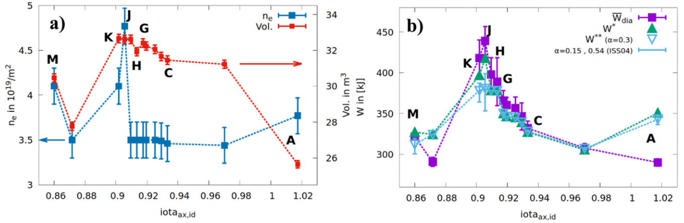
Figure 6. Configuration and experiment parameters displayed versus \text{iota} on axis making configuration labels (A to M) run sequentially from right to left. For orientation, some experimental points have been supplied with their label. Missing labels can be inferred from the indicated sequence. (a) Line-integrated density (@3.5 s) and volume of the vacuum configurations of the HSI-scan. The errorbar of \pm 2 \times 10^{18} \text{ m}^{-2} encompasses the statistical and systematic errors of the diagnostic [19]. The errorbar in the volume illustrates a variation in the minor radius \delta r_{\text{eff}} = \pm 2 \text{ mm} where r_{\text{eff}} is in the range of 49 cm to 54 cm. (b) Measured diamagnetic energy W_{\text{dia}} @3.5 s (violet), energy W^* which is scaled to a norm-volume of 31.5 \text{ m}^3 (green filled triangles) and energy W^{**} which is additionally scaled to a norm-line-density of 3.5 \times 10^{19} \text{ m}^{-2} (blue, open, upside-down triangles).
