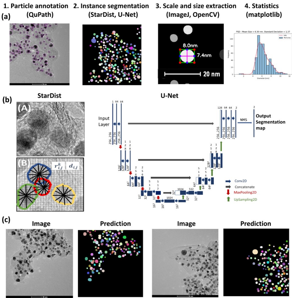
Fig. 1 (a) Methodical pipeline for deep learning-based analysis of particle size distribution involving 1. particle annotation, 2. supervised training for the instance segmentation of particles, 3. setting scale for image calibration and particle size extraction with computer vision implemented using OpenCV library 42 , 4. Obtaining particle size statistics with visualization libraries, e.g., matplotlib. (b) The left panel shows a TEM image with overlapped Pt particles supported on a carbon agglomerate; the StarDist method used in this work predicts star-convex polygons parameterized by the radial distances r_{i,j}^k , and object probabilities d_{i,j} for the pixel i,j . 43 The right panel shows the U-Net architecture 44 and selected the final instances via the non-maximum suppression (NMS) technique. (c) Example TEM images and their corresponding predicted instance segmentation of Pt particles using StarDist and U-Net.
