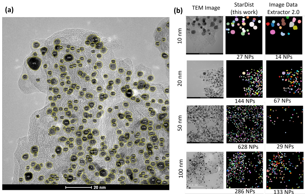
Fig. 5 (a) Localization and counting the particles made available by the deep learning approach. (b) Comparison between the predicted segmentation maps of test images at different scales using the StarDist model employed in this work and the ImageDataExtractor 2.0 64
