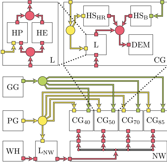
Fig. 9. Superstructure with components for the gas grid (GG), power grid (PG), waste heat source (WH) and network (NW) as well as subsystems for linking (L) and consumer groups (CG), see top. The superstructure of the linking subsystem contains a heat pump (HP) and a heat exchanger (HE) and that of the consumer group subsystems contains two heat source (HS) components parameterized as a heating rod (HS HR ) and a boiler (HS B ) and demand (DEM) as well as a decentral linking subsystem. To connect the different consumer groups, the necessary pipe segments (depicted as gray bars within NW) need to be built.
