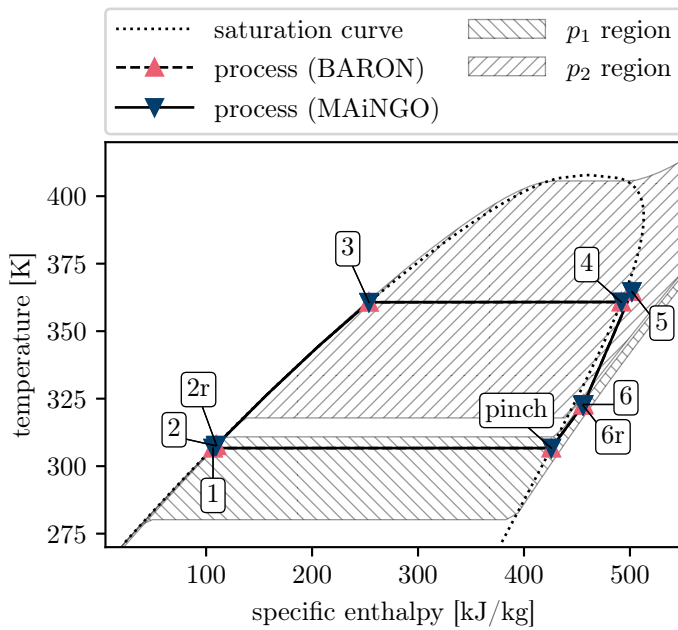
Fig. 13. Processes resulting from the optimization using BARON and MAiNGO and boundaries of pressure variables p_1 and p_2 .
