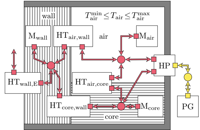
Fig. 7. Structure of the considered building energy system and implementation in COMANDO: three instances of the thermal mass class ( M_{\text{air}} , M_{\text{core}} , M_{\text{wall}} ), four instances of the heat transfer class ( HT_{\text{air,wall}} , HT_{\text{wall,E}} , HT_{\text{air,core}} , HT_{\text{core,wall}} ), heat pump (HP), and power grid (PG). Red arrows represent heat flows and yellow arrows electric power flows.
