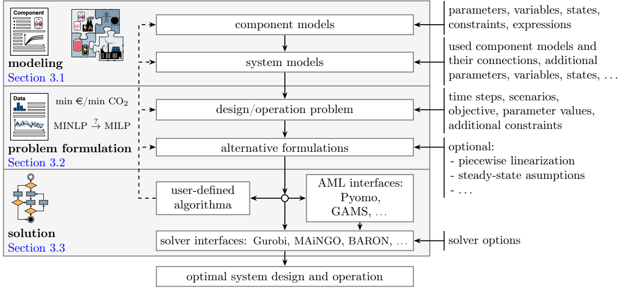
Fig. 1. Workflow for modeling, problem formulation, and optimization using COMANDO.
