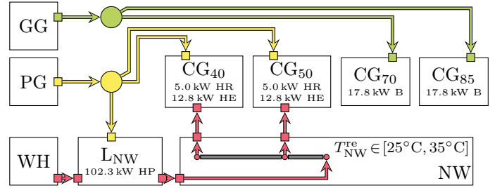
Fig. 11. Optimal system structure: A central heat pump HP supplies waste heat from WH to the network NW. Consumer groups CG 40 and CG 50 are connected to NW via heat exchangers (HE) and use heating rods (HR) for peak demands. Consumer groups CG 70 and CG 85 are not connected and satisfy their heat demand via boilers (B).
