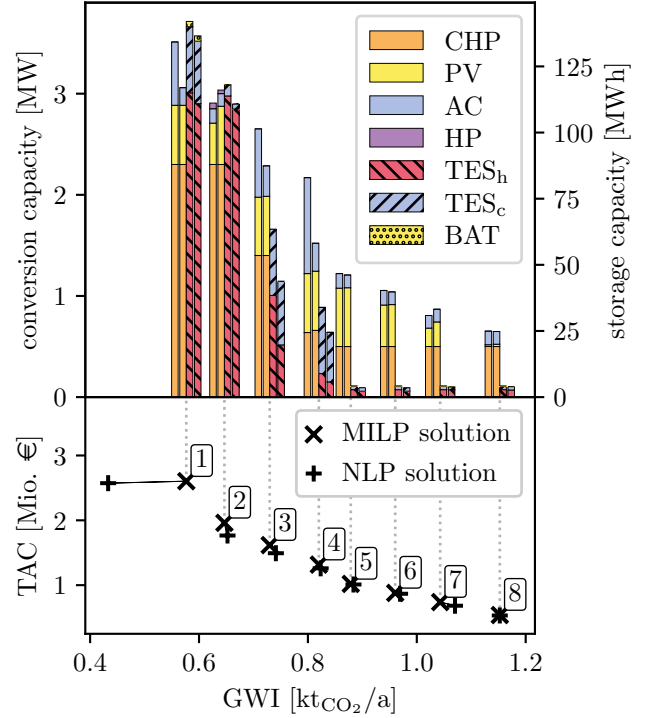
Fig. 6. Bottom: eight Pareto-optimal designs, determined from multi-objective optimization regarding total annualized cost (TAC) and global warming impact (GWI). Top: corresponding capacities of conversion (left) and storage components (right) from the MILP (inner bars) and NLP (outer bars) formulations. CHP: Combined heat and power unit, PV: photovoltaic array, AC: absorption chiller, HP: heat pump, TES_h : hot thermal energy storage, TES_c : cold thermal energy storage, BAT: battery. Note that boilers and compression chillers are not part of any design and thus excluded from the legend.
