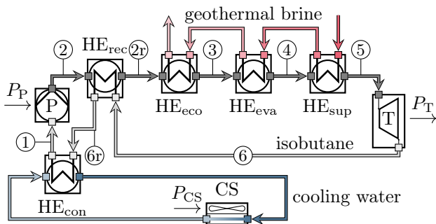
Fig. 12. System model of the ORC process from Huster et al. (2019). The components are a pump (P), a recuperator ( HE_{rec} ), an economizer ( HE_{eco} ), an evaporator ( HE_{eva} ), a superheater ( HE_{sup} ), a turbine (T), a condenser ( HE_{con} ), and a cooling system (CS). Flows of geothermal brine, the working fluid isobutane, and cooling water are depicted in red, gray, and blue, respectively. Electrical power is consumed by pump ( P_P ) and cooling system ( P_{CS} ) and produced by the turbine ( P_T ).
