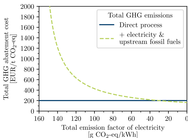
Fig. 11. Total GHG abatement cost for complete decarbonization of copper production by Power-to- \text{H}_2 , i.e., 100% reduction of direct emissions. The remaining indirect GHG emissions of electricity are based on the total emission factor of electricity and the fossil fuels consider the avoided upstream GHG emissions from natural gas and coke supply.
