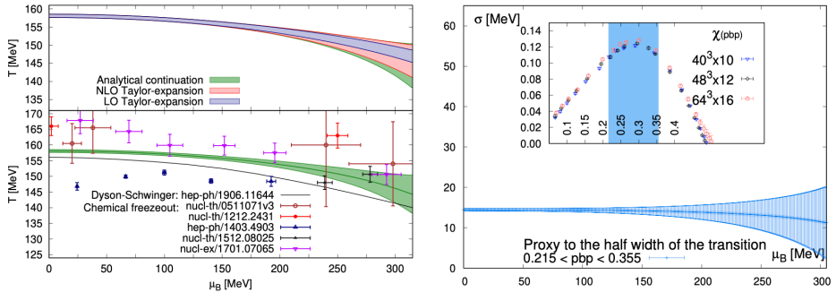
Fig. 2. (Color online) Left: Top — Transition line extrapolated from lattice simulations at imaginary chemical potential (gray/green band) compared with an extrapolation using the formula in Eq. (1) up to \kappa_4 (light gray/red band) or up to \kappa_2 (dark gray/blue band). Bottom — Our crossover transition line compared to a prediction from truncated Dyson-Schwinger equations [36] and some estimates of the chemical freezeout parameters in heavy-ion collisions [37–41]. Right: Half width of the transition. In the inset we show a plot of the \chi(\langle\bar{\psi}\psi\rangle) peak, where the shaded region corresponds to \langle\bar{\psi}\psi\rangle_c \pm \Delta\langle\bar{\psi}\psi\rangle/2 . Both are extrapolated to real \mu_B .
