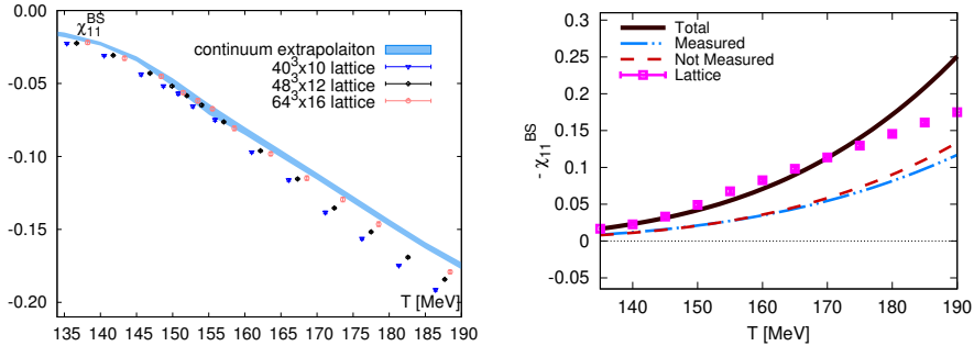
Fig. 3. (Color online) From Ref. [33]. Left: Continuum extrapolated results for the correlator \chi_{11}^{BS} as a function of the temperature at \mu_B = 0 (gray/blue band). The different datapoints correspond to results at finite lattice spacing. Right: Lattice results compared to HRG model calculations (solid black line), with the contribution from measured (dot-dashed blue line) and non-measured (dashed red line) hadronic species.
