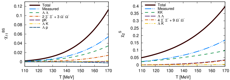
Fig. 4. From Ref. [33]. Contributions from ‘measured’ states to -\chi_{11}^{BS} (left panel) and \chi_2^S (right panel), at \mu_B = 0 , as functions of the temperature.
