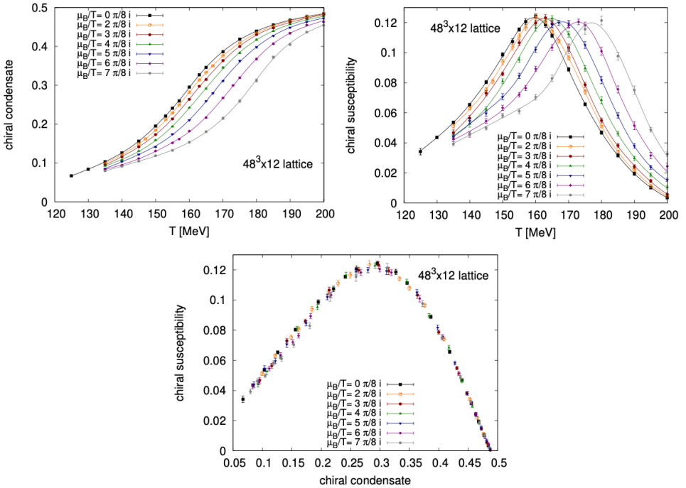
Fig. 1. (Color online) Renormalized chiral condensate \langle \bar{\psi}\psi \rangle (upper left) and chiral susceptibility \chi (upper right) as functions of the temperature for the intermediate lattice spacing in this study. The black, first from the top, curves correspond to vanishing baryon density, while results for various imaginary values of the chemical potential are shown in shades of grey (other colors). Finally, in the lower panel, we show the susceptibility as a function of the condensate. In this representation, the chemical potential dependence is very weak.
