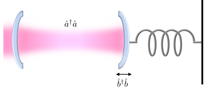
FIG. 1. Cavity optomechanics is one realization of the Hamiltonian (1). A semitransparent mirror allows the electromagnetic field to enter the cavity and interact with a moving-end mirror, which therefore affects the frequency of the fundamental modes that can be trapped in the cavity [33]. The degree of freedom of the mirror (i.e., its position) can be modeled as a harmonic oscillator coherently interacting with the field.
