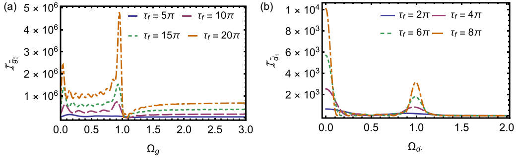
FIG. 3. QFI for estimation of (a) \tilde{g}_0 and (b) \tilde{d}_1 for different frequencies. Parameters are \tilde{g}_0 = 1 , \epsilon = 0.5 , and \mu_c = 1 for (a), and \tilde{g}_0 = 1 and \mu_c = 1 for (b). We find that the constant case and the resonances perform best. While the resonance at about \Omega_g = 1 gives the best QFI for the estimation of \tilde{g}_0 , the QFI for the estimation of \tilde{d}_1 at the resonance \Omega_{d_1} = 1 is smaller compared with when \tilde{D}_1(\tau) is constant.
