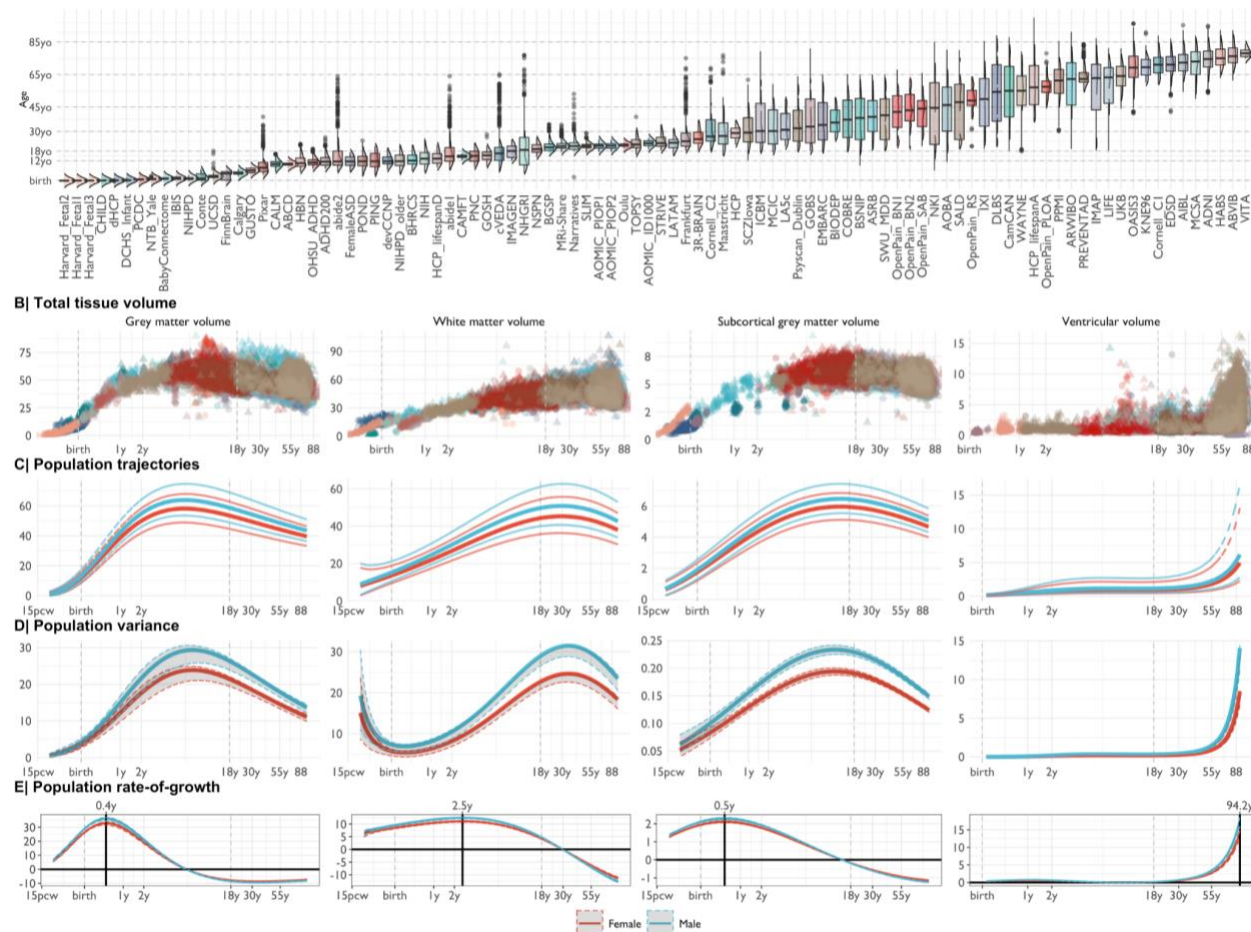
Fig. 1: Neuroimaging growth charts. A| MRI data were aggregated from 96 primary studies of 120,685 scans collectively spanning the age range from late pregnancy to 100 postnatal years. Box-violin plots show age distributions (log-scaled) of each study. B| Raw, non-centiled bilateral volume estimates plotted for each participant, coloured by study, as a function of age (log-scaled) and scaled to 10,000mm 3 . C| Normative growth curves estimated by generalised additive modelling for location scale and shape (GAMLSS), accounting for study offsets, processing pipeline, stratified by sex (female/male as red/blue) and providing reference centile boundaries of 95% (dotted lines), analogous to a paediatric growth chart. D| Across-individual variance with the 95% confidence interval determined by 1000 bootstraps stratified by sex. E| Rate of change across the lifespan (first derivative of the primary trajectory) stratified by sex, with solid black lines at zero (where the sign of the trajectory flips) and at age of peak growth (exact year denoted on the top mirrored x-axis).
