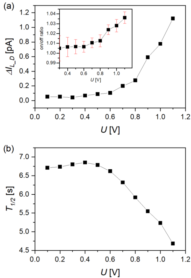
Figure 6: Photoconductance of \text{Ru}(\text{MPTP})_2\text{-AuNP} devices. (a) Difference between light current and dark current, \Delta I_{L_D} ; inset: on/off ratio. Red bars correspond to standard deviation. (b) Half-life of current decline after peak induced by switching the light source “on” or “off”.
