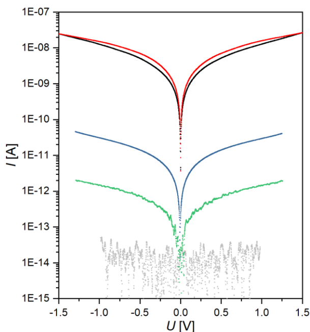
Figure 3: Log current versus voltage curves of \text{Ru(TP)}_2 -complex wire devices (green), multiple \text{Ru(MPTP)}_2 -AuNP devices (blue), single \text{Ru(MPTP)}_2 -AuNP devices (red/black), and empty nanogaps representing the noise level (grey).
