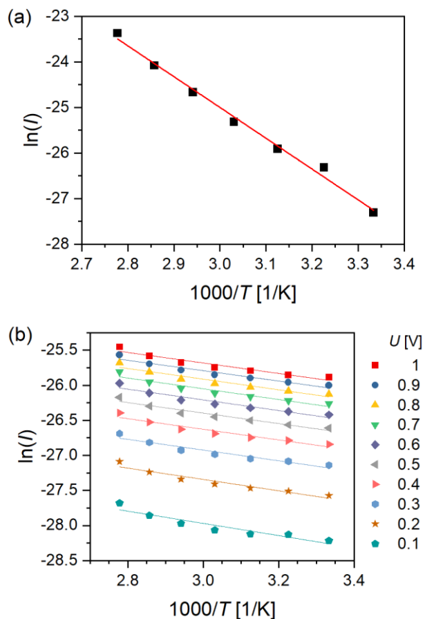
Figure 4: Arrhenius plots. (a) Ru(TP) 2 -complex wire device ( U = 1 V). (b) Ru(MPTP) 2 -AuNP device for voltages between 0.1 V and 1 V. Points correspond to measurements while lines correspond to linear regressions.
